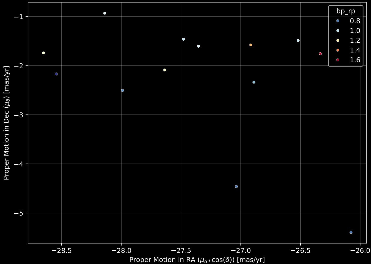
Gaia Stream: [New-14] Proper Motion Diagram (n= 13)
