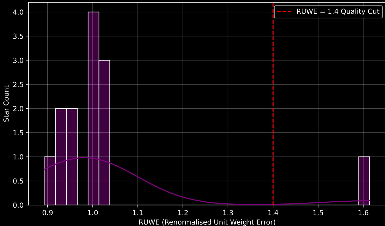
Gaia Stream: [New-14] RUWE Distribution (n= 13)
