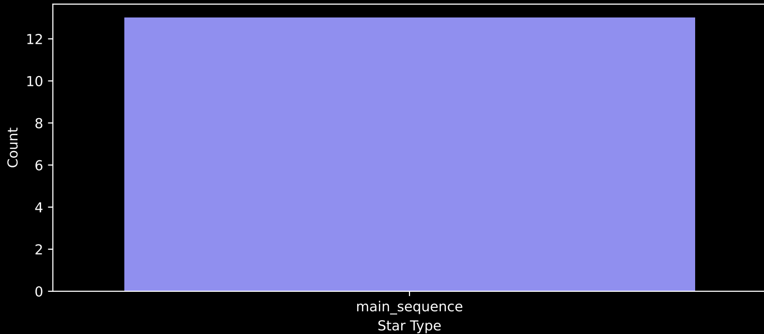
Gaia Stream: [New-14] Count plot of Star Type
