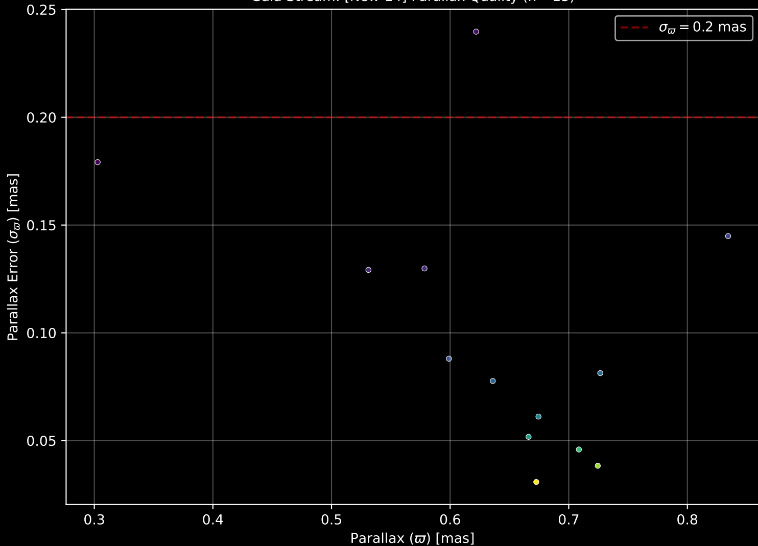
Gaia Stream: [New-14] Parallax Quality (n= 13)
