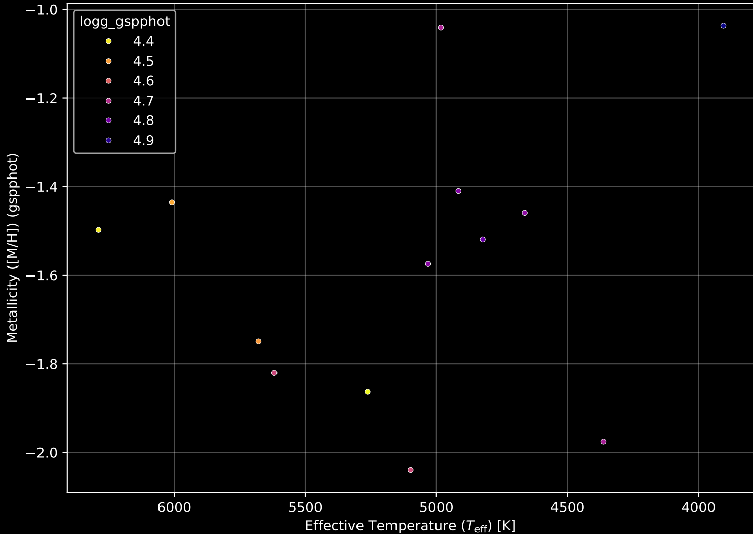
Gaia Stream: [New-14] Stellar Population Parameters (n= 13)
