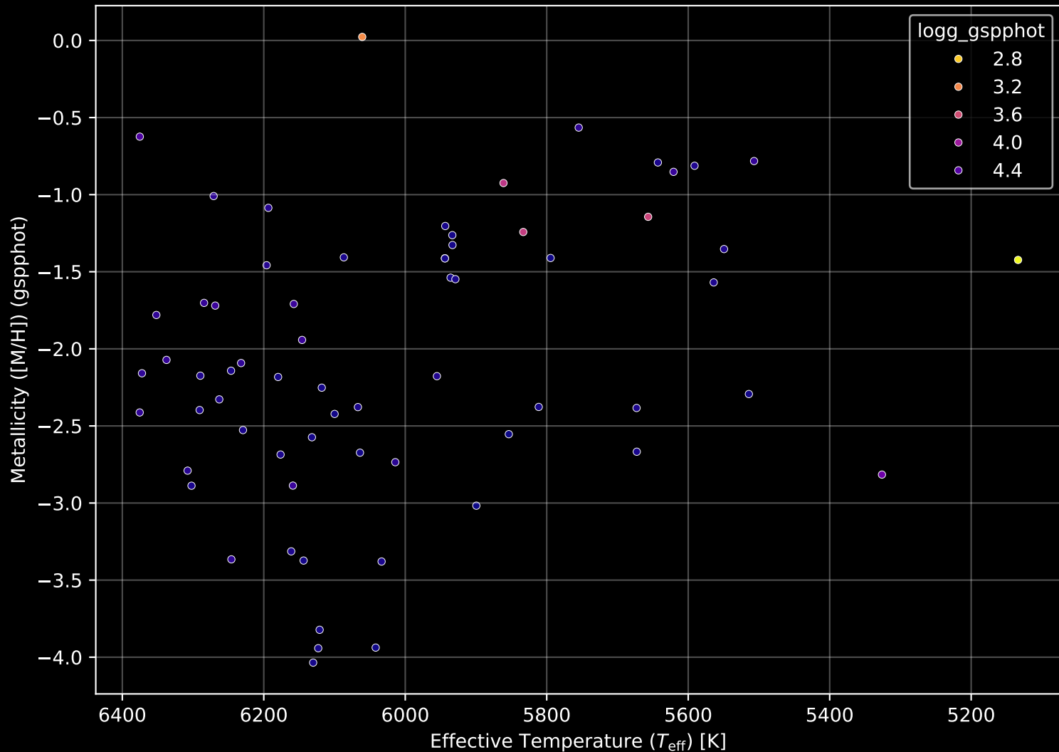
Gaia Stream: [New-15] Stellar Population Parameters (n= 66)
