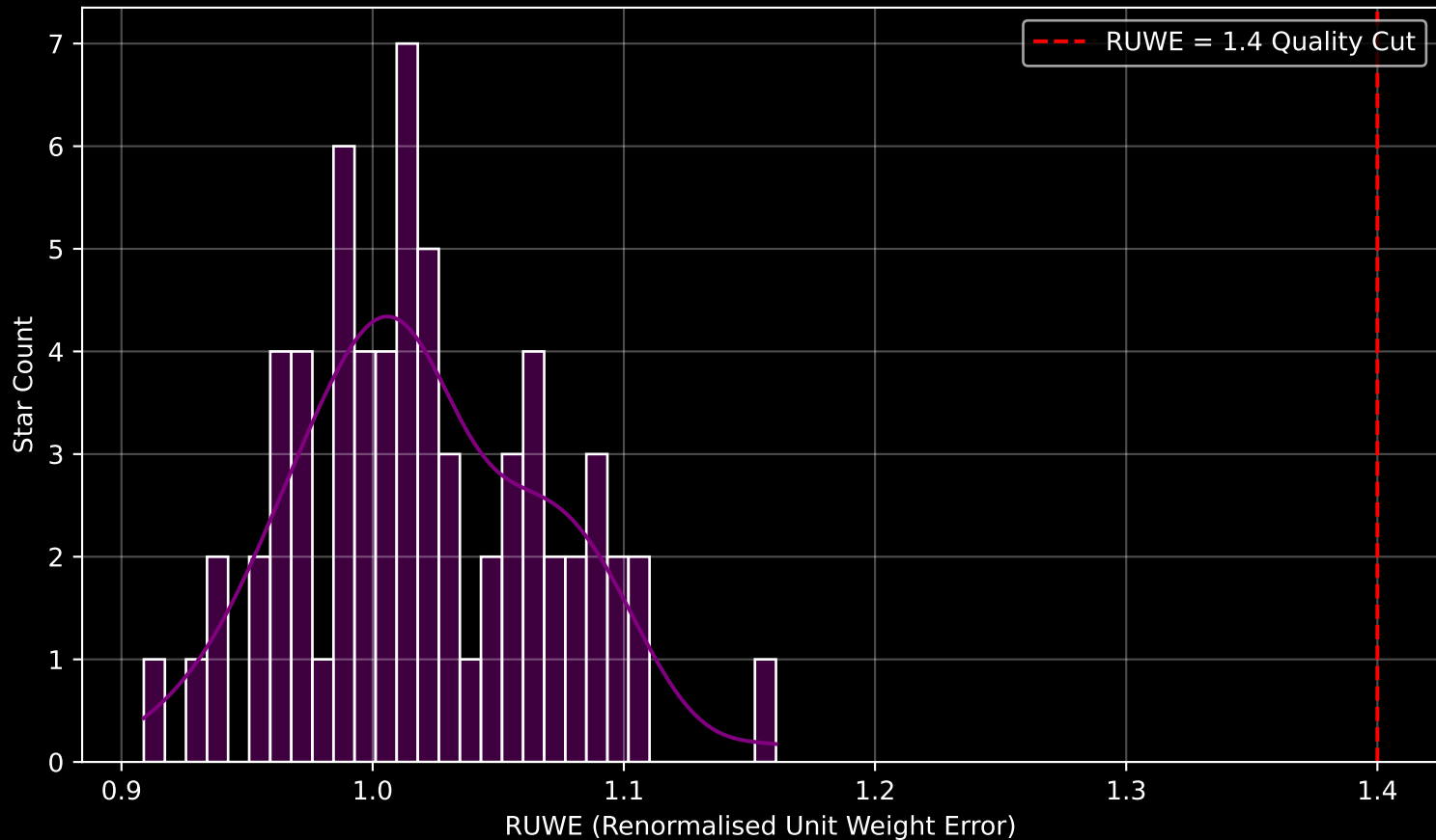
Gaia Stream: [New-15] RUWE Distribution (n= 66)
