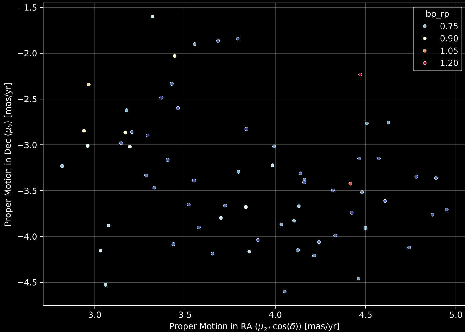
Gaia Stream: [New-15] Proper Motion Diagram (n= 66)
