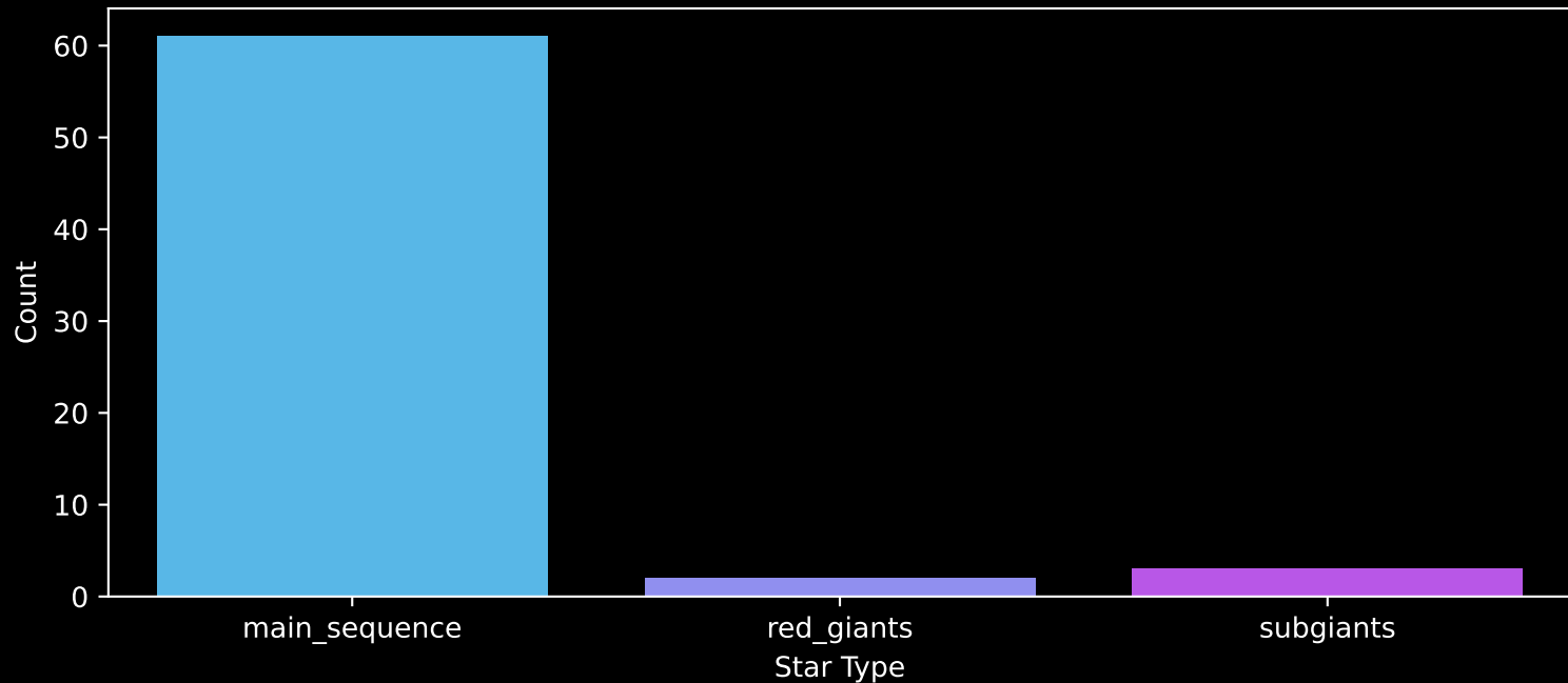
Gaia Stream: [New-15] Count plot of Star Type
