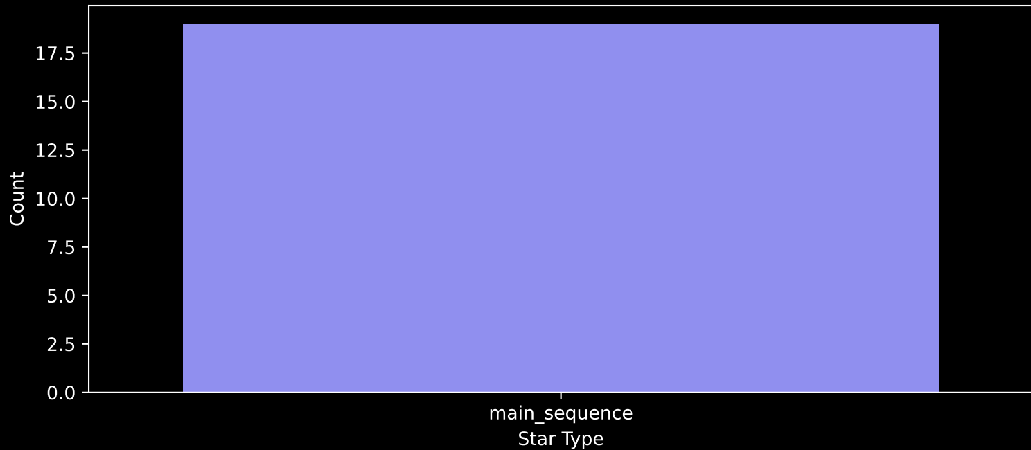
Gaia Stream: [New-16] Count plot of Star Type
