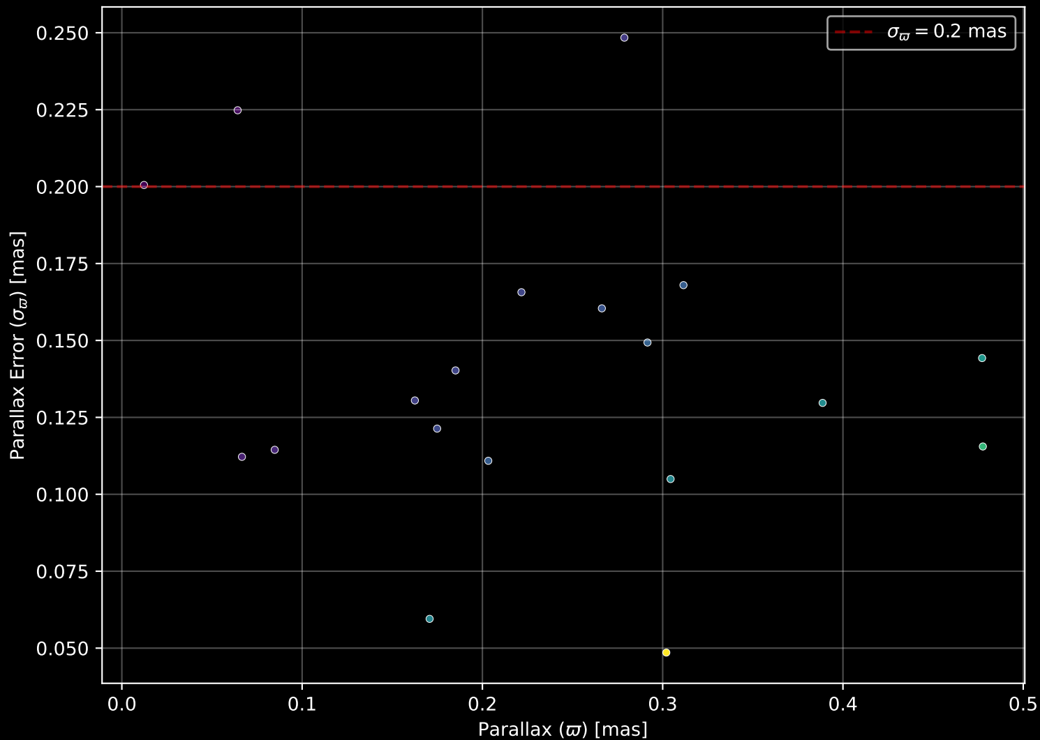
Gaia Stream: [New-16] Parallax Quality (n= 19)
