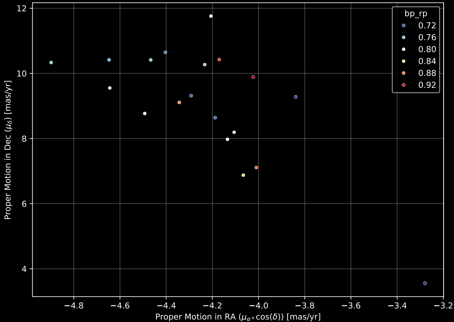
Gaia Stream: [New-16] Proper Motion Diagram (n= 19)
