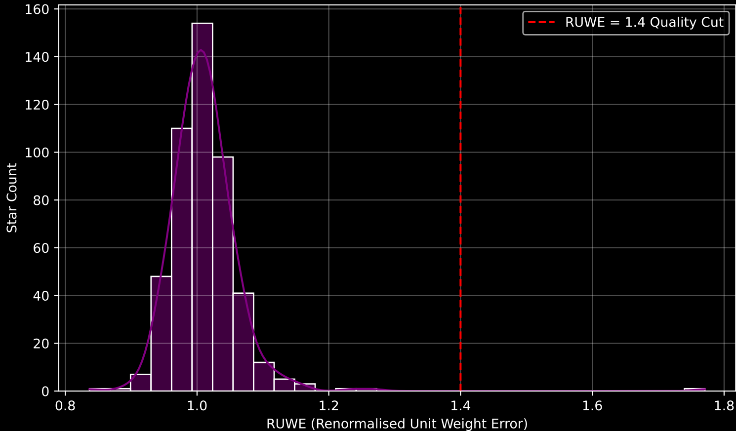
Gaia Stream: [New-21] RUWE Distribution (n= 483)
