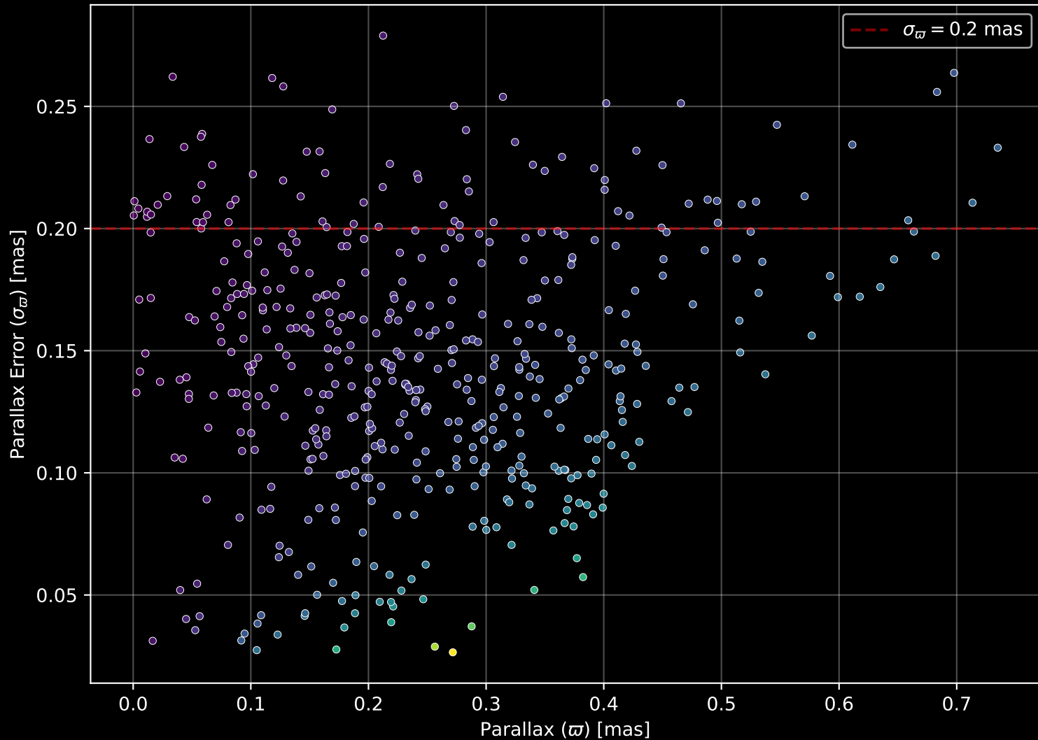
Gaia Stream: [New-21] Parallax Quality (n= 483)
