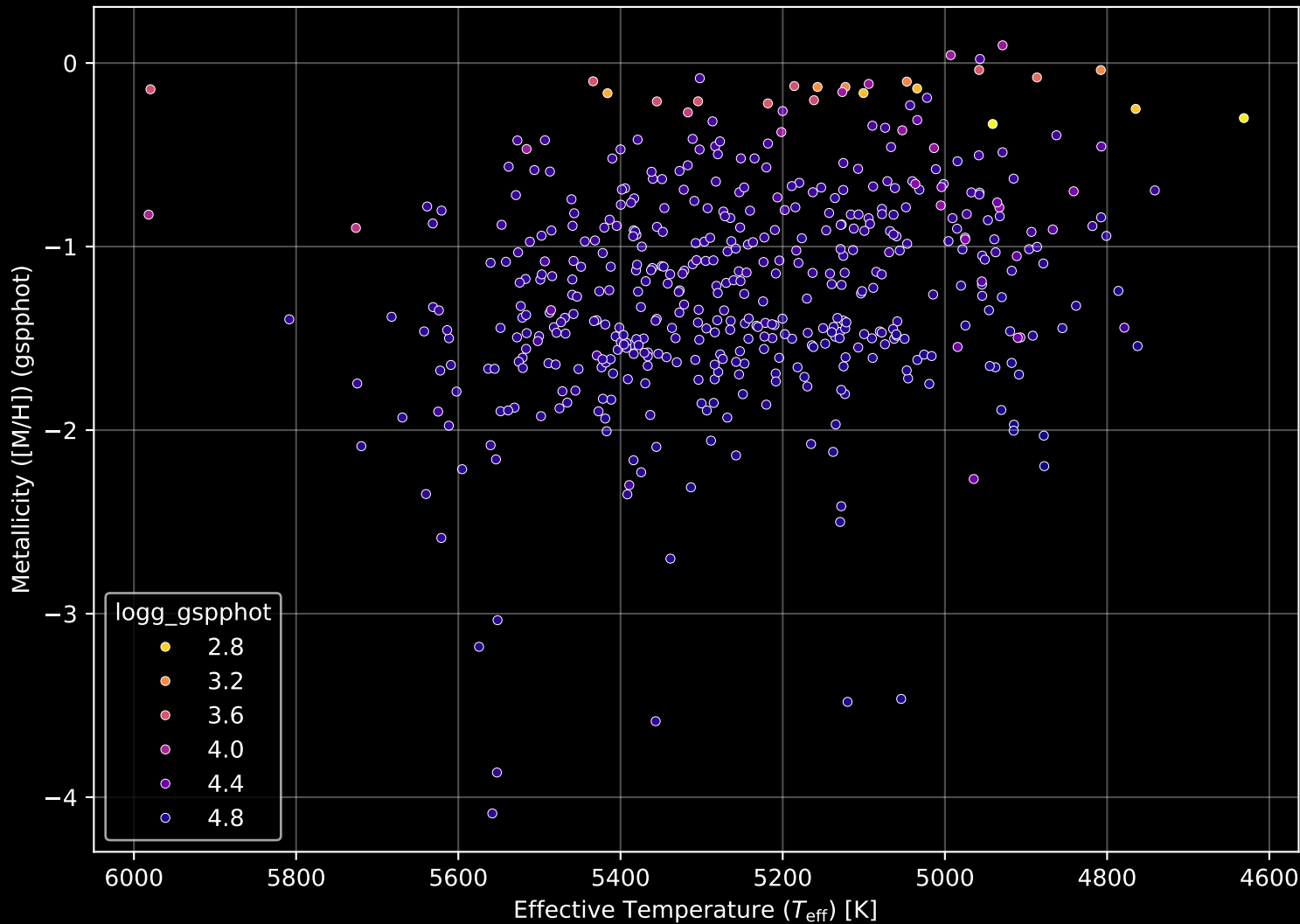
Gaia Stream: [New-21] Stellar Population Parameters (n= 483)
