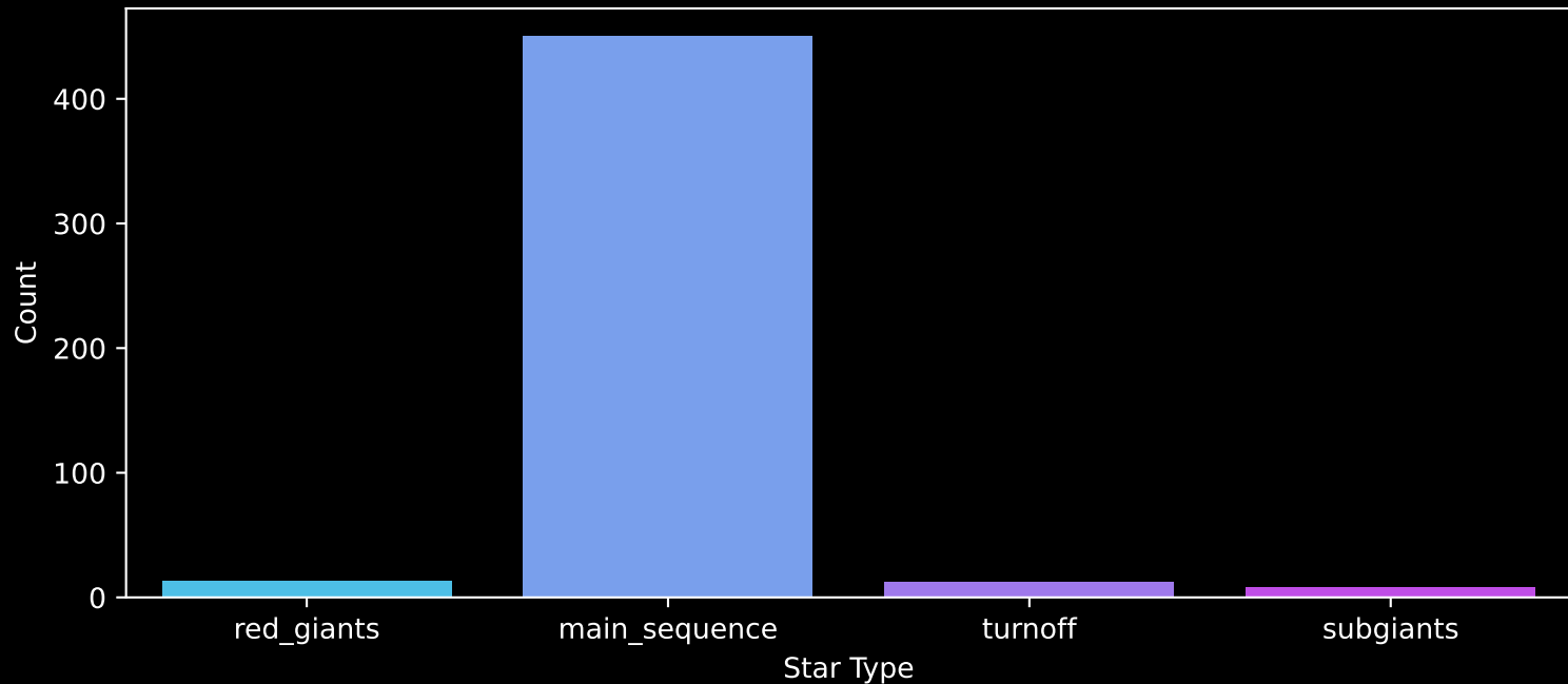
Gaia Stream: [New-21] Count plot of Star Type
