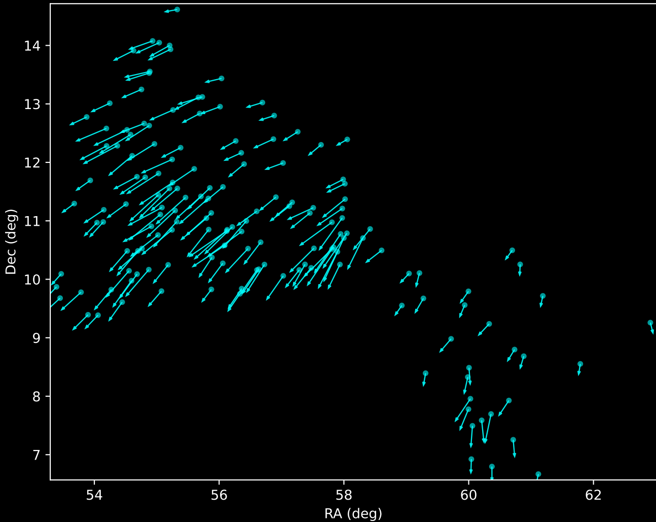
Gaia DR3 Noise Stream Proper Motion Vectors (n=155)
