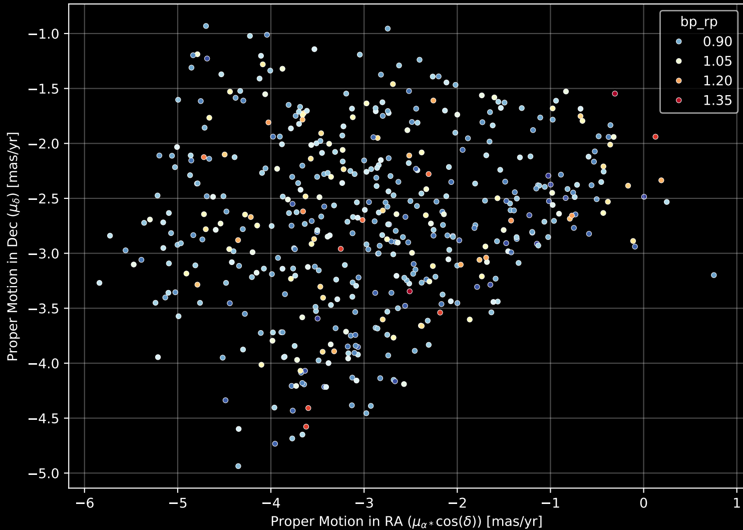
Gaia Stream: [New-21] Proper Motion Diagram (n= 483)
