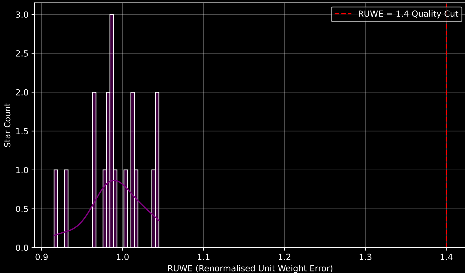
Gaia Stream: [New-22] RUWE Distribution (n= 18)
