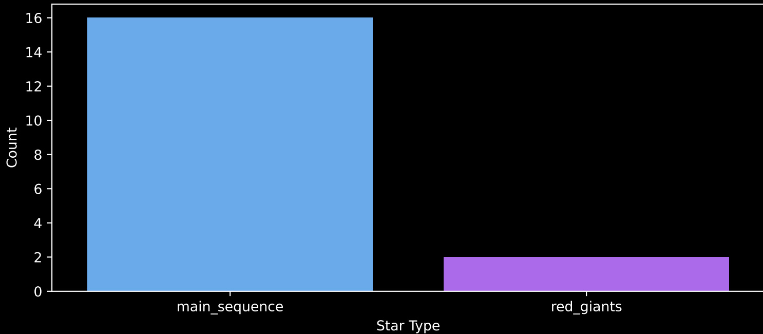
Gaia Stream: [New-22] Count plot of Star Type
