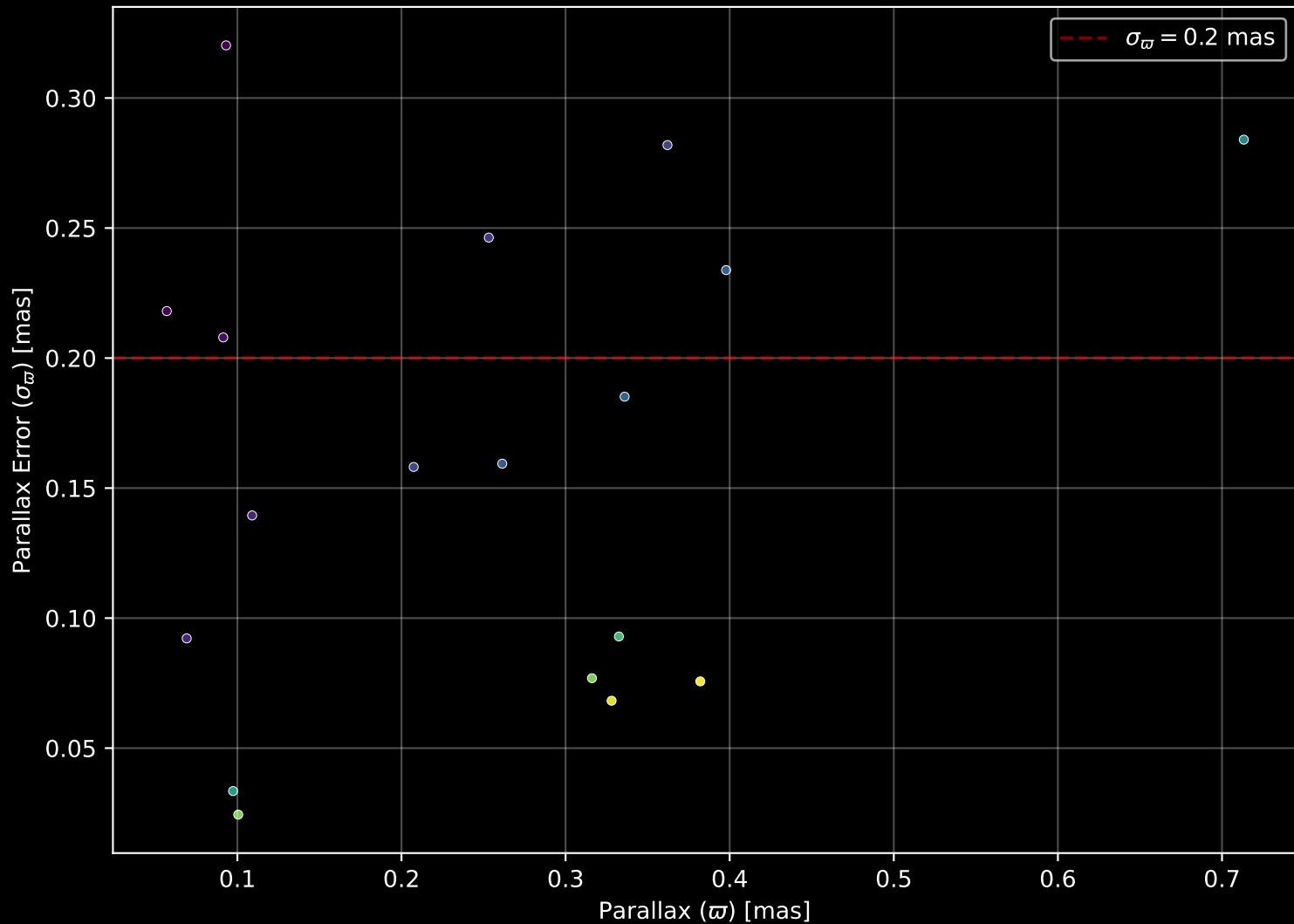
Gaia Stream: [New-22] Parallax Quality (n= 18)
