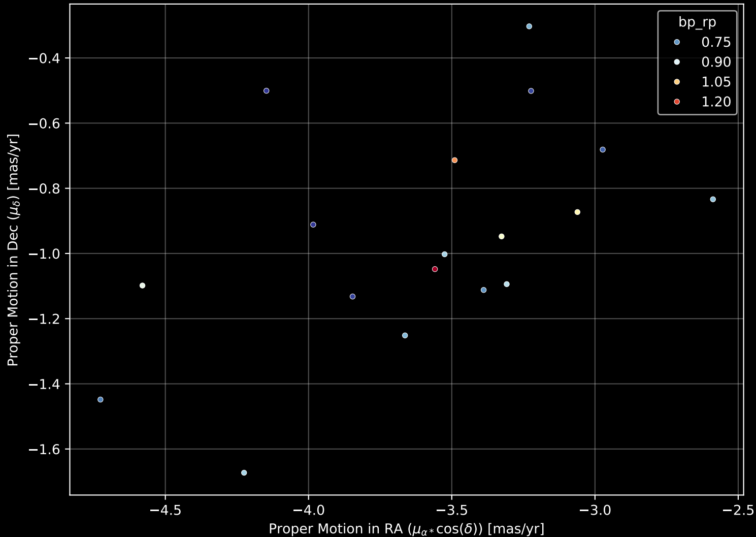
Gaia Stream: [New-22] Proper Motion Diagram (n= 18)
