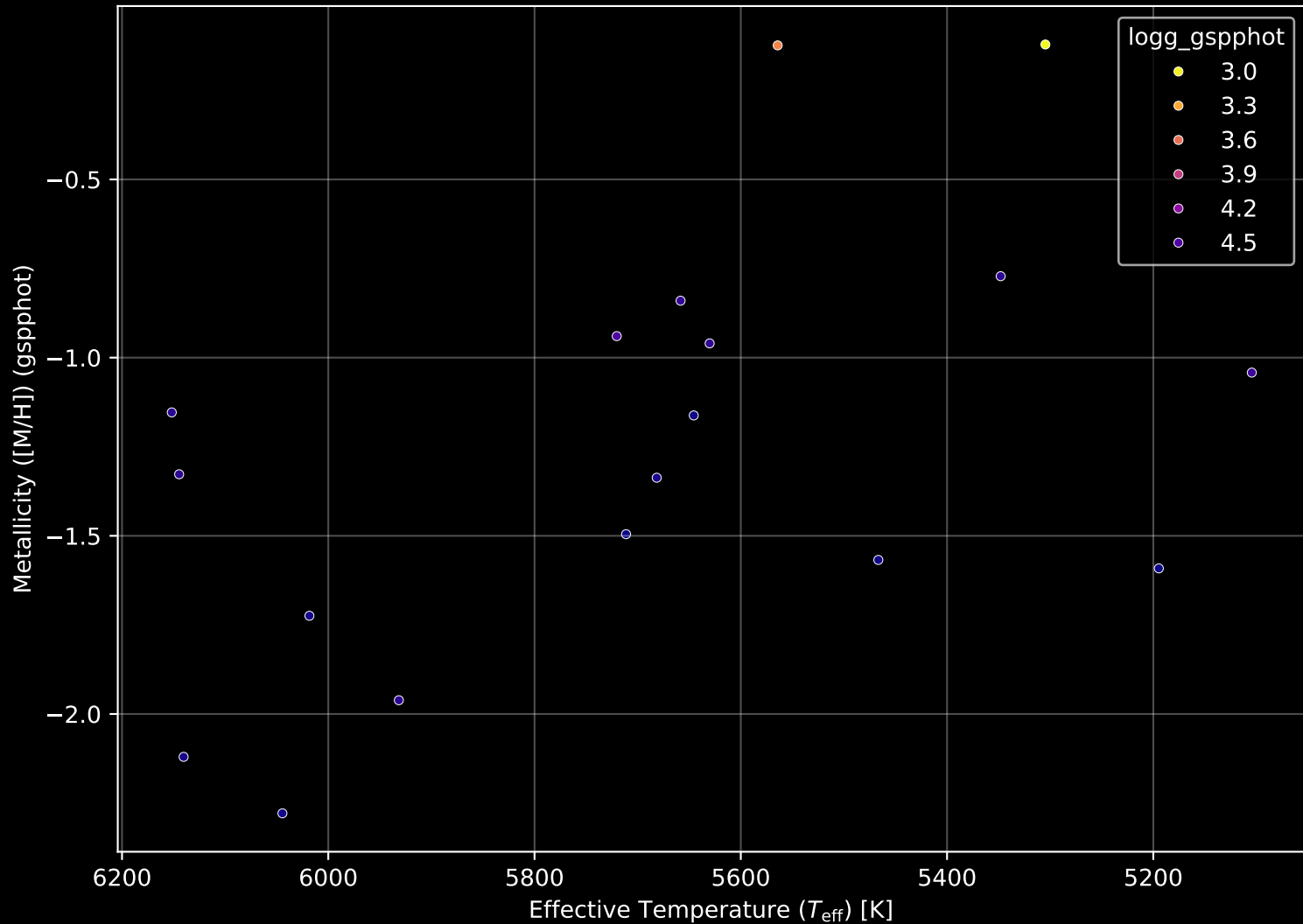
Gaia Stream: [New-22] Stellar Population Parameters (n= 18)
