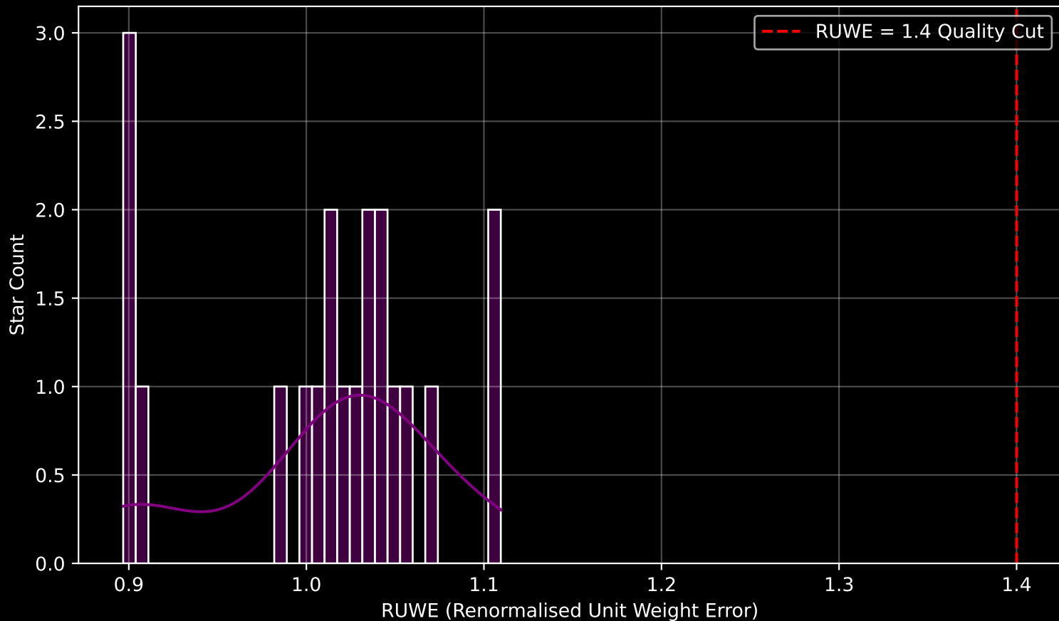
Gaia Stream: [New-23] RUWE Distribution (n= 20)
