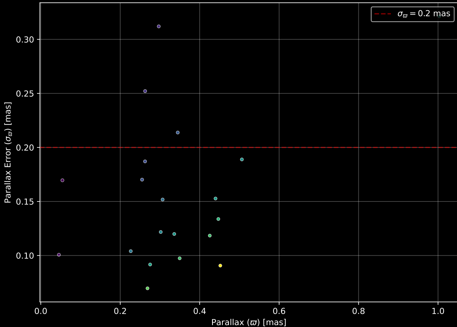
Gaia Stream: [New-23] Parallax Quality (n= 20)
