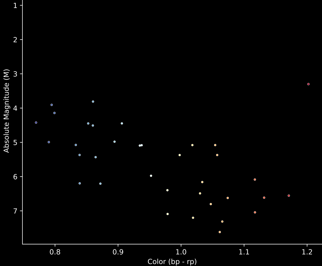
Gaia Stream: [New-24] Stream (n= 36) Hertzsprung-Russel Diagram
