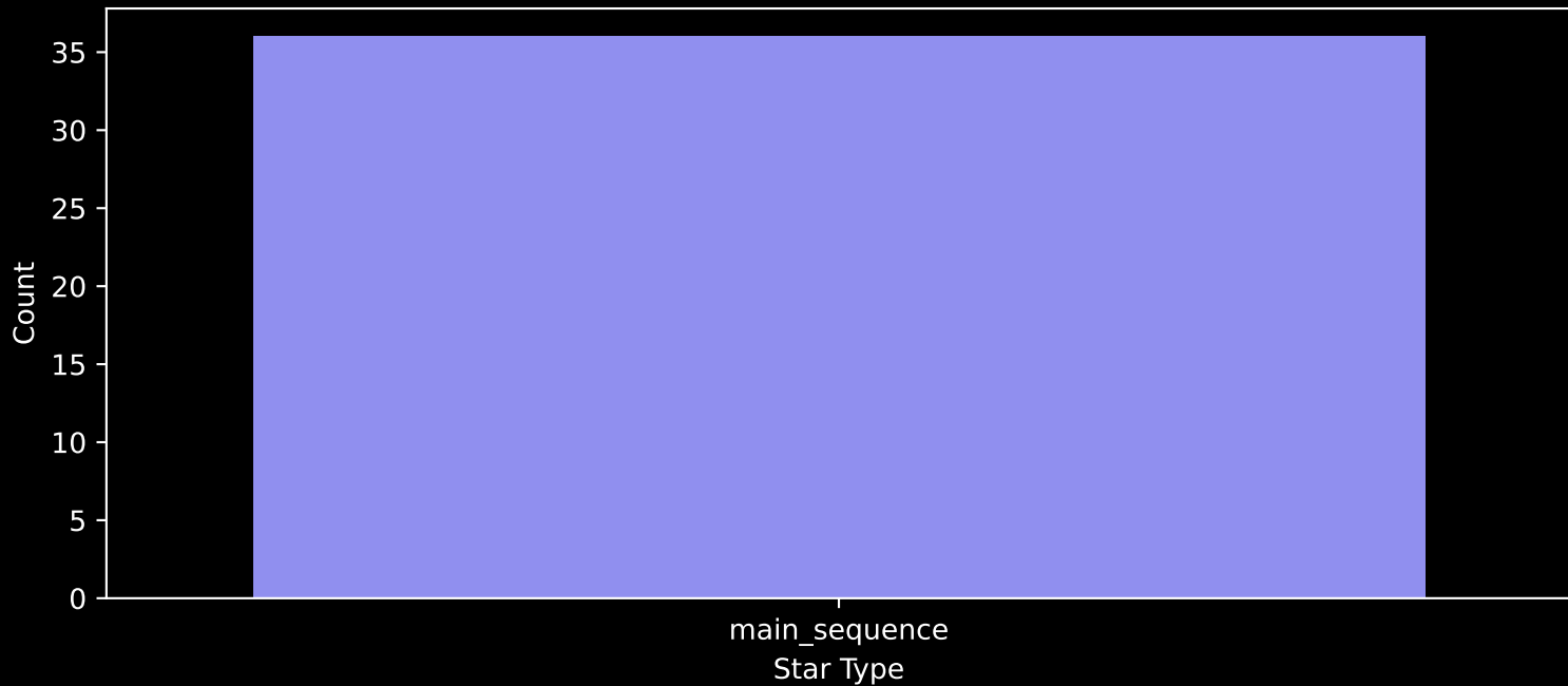
Gaia Stream: [New-24] Count plot of Star Type
