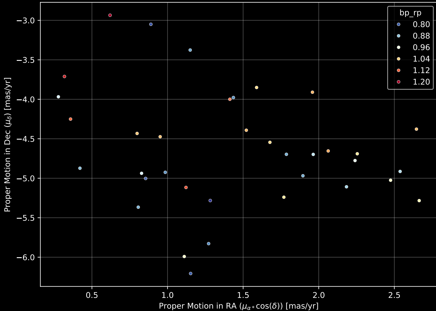
Gaia Stream: [New-24] Proper Motion Diagram (n= 36)
