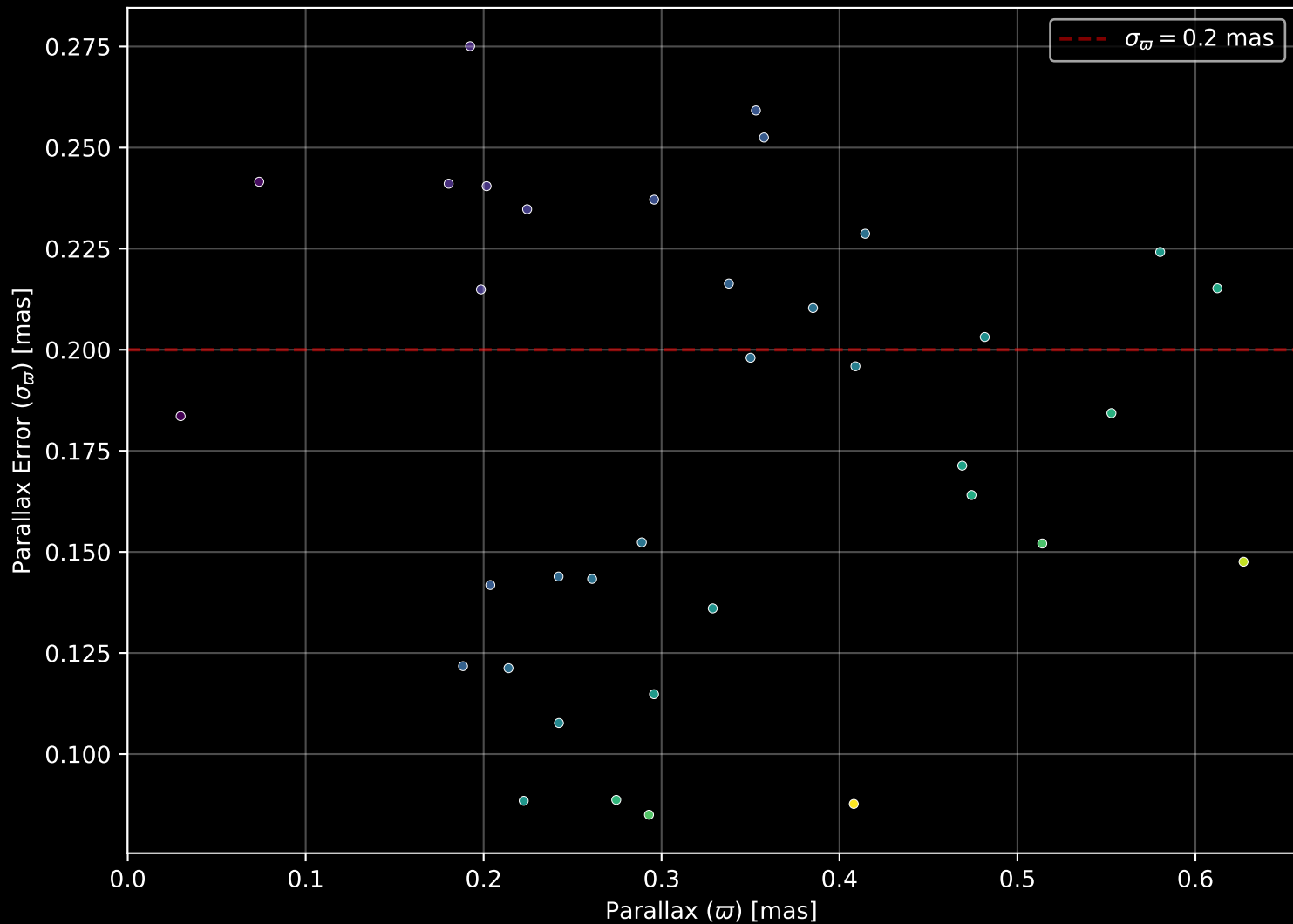
Gaia Stream: [New-24] Parallax Quality (n= 36)
