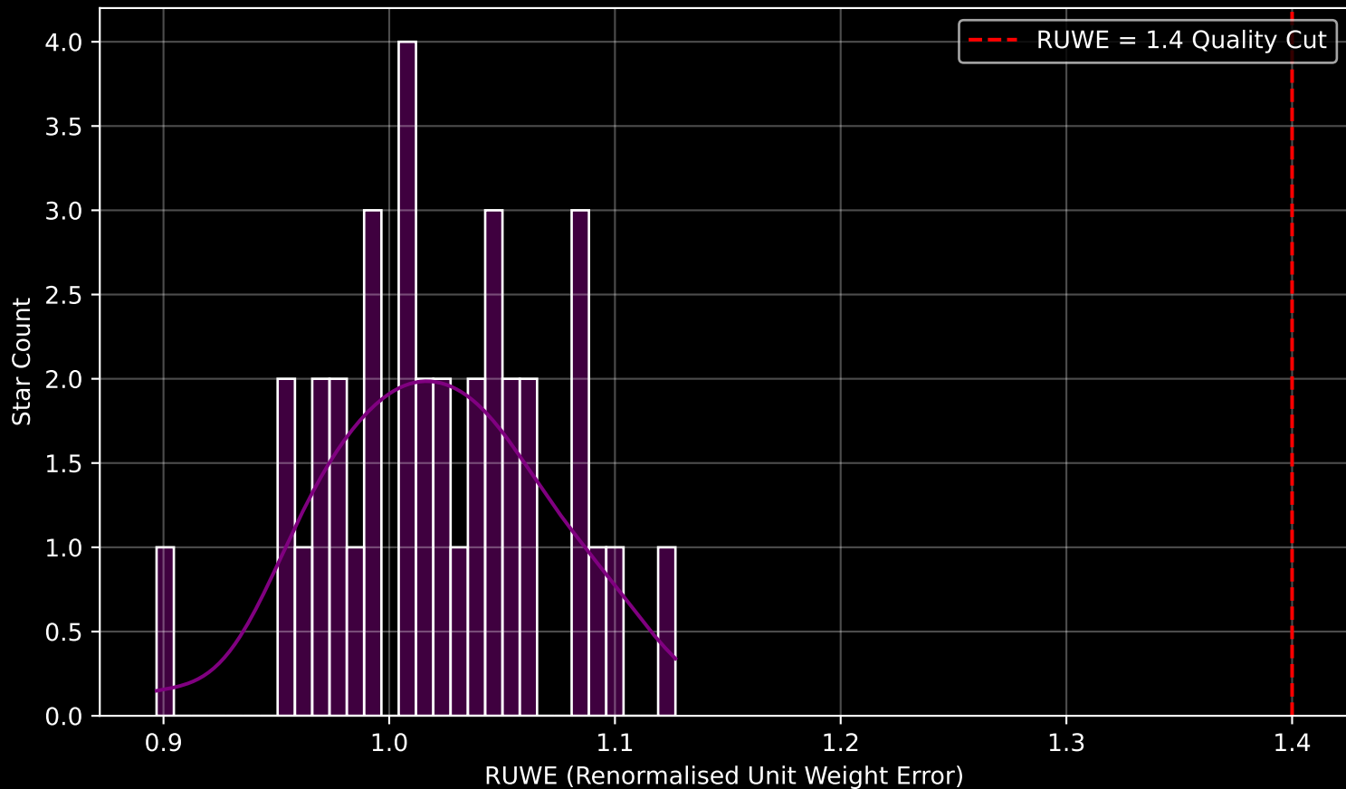
Gaia Stream: [New-24] RUWE Distribution (n= 36)
