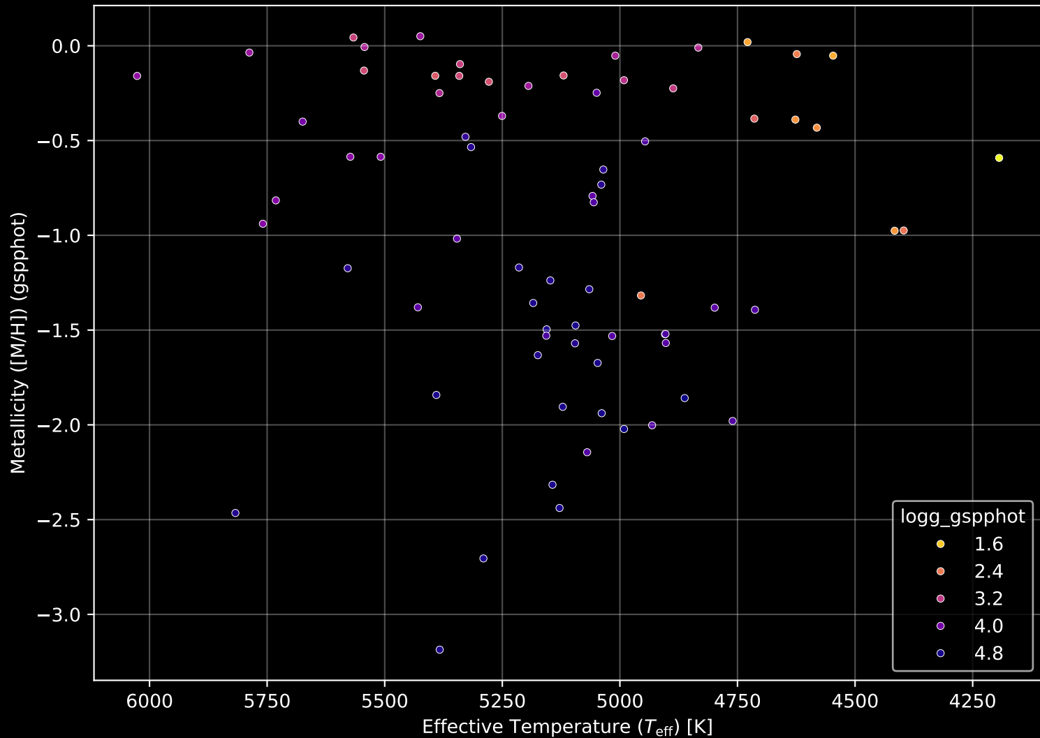
Gaia Stream: [New-25] Stellar Population Parameters (n= 73)
