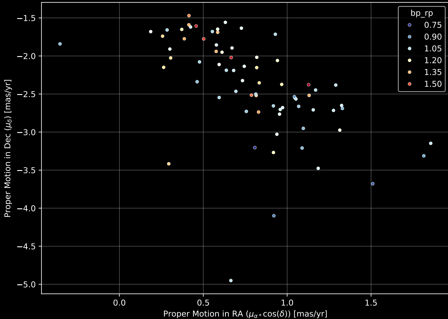
Gaia Stream: [New-25] Proper Motion Diagram (n= 73)
