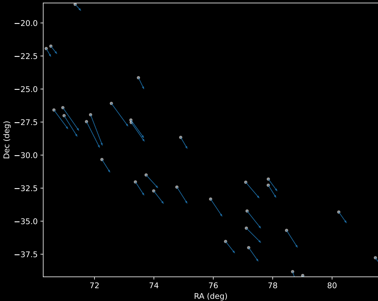
Gaia DR3 Cluster 0 Proper Motion Vectors (n=31)
