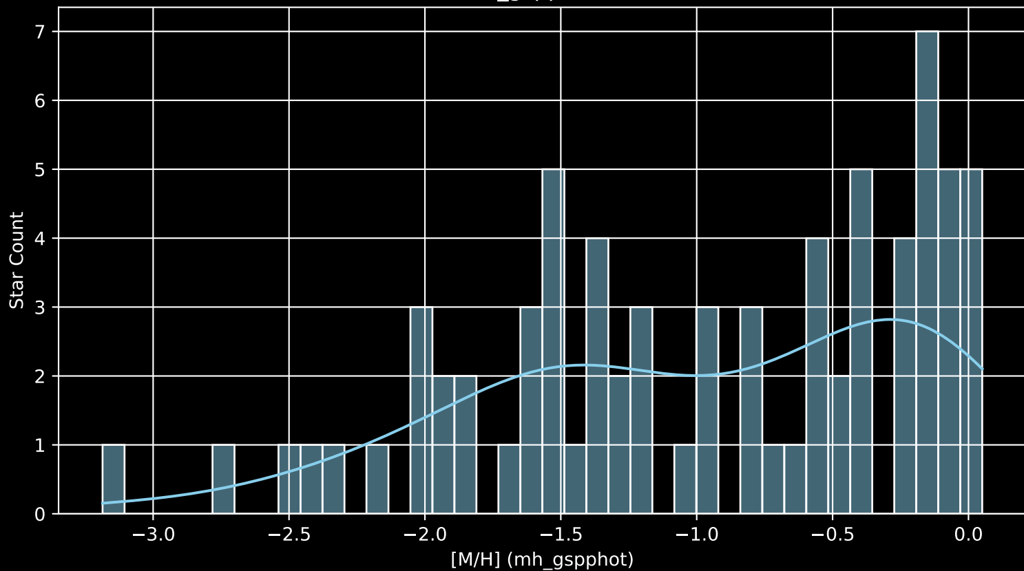
Gaia Stream: [New-25 [M/H] (mh_gspphot) (n= 73)
