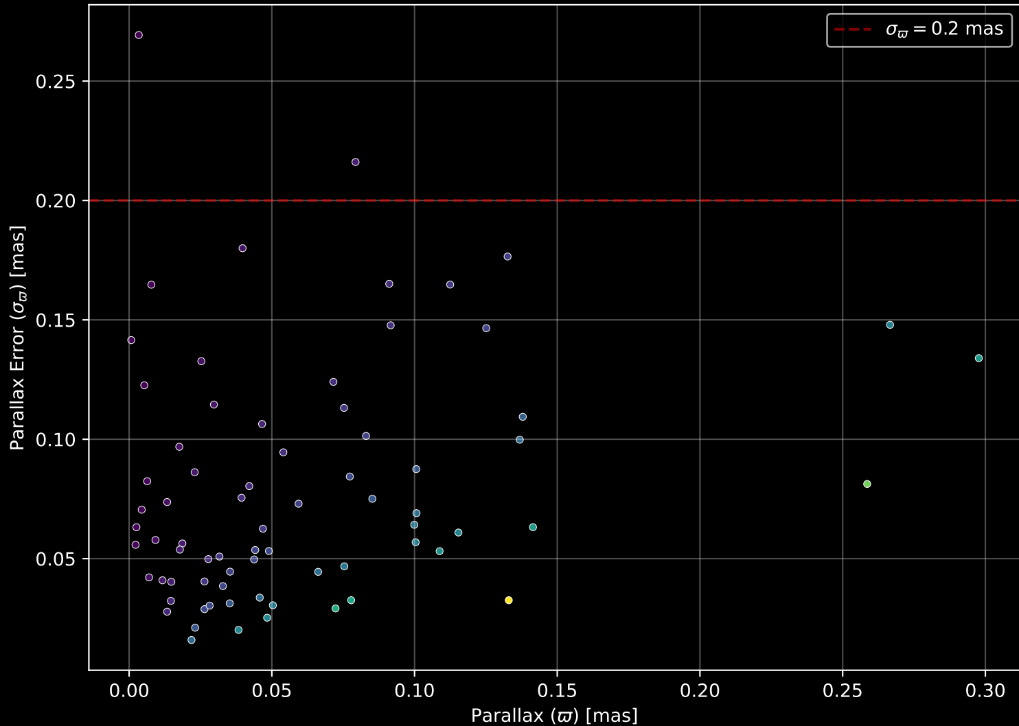
Gaia Stream: [New-25] Parallax Quality (n= 73)
