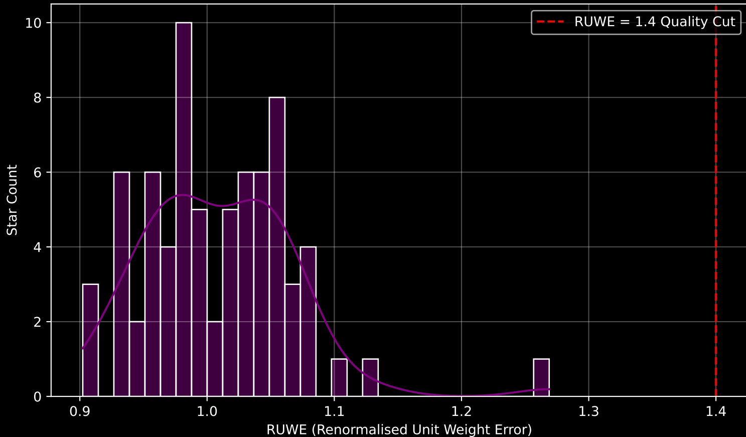
Gaia Stream: [New-25] RUWE Distribution (n= 73)
