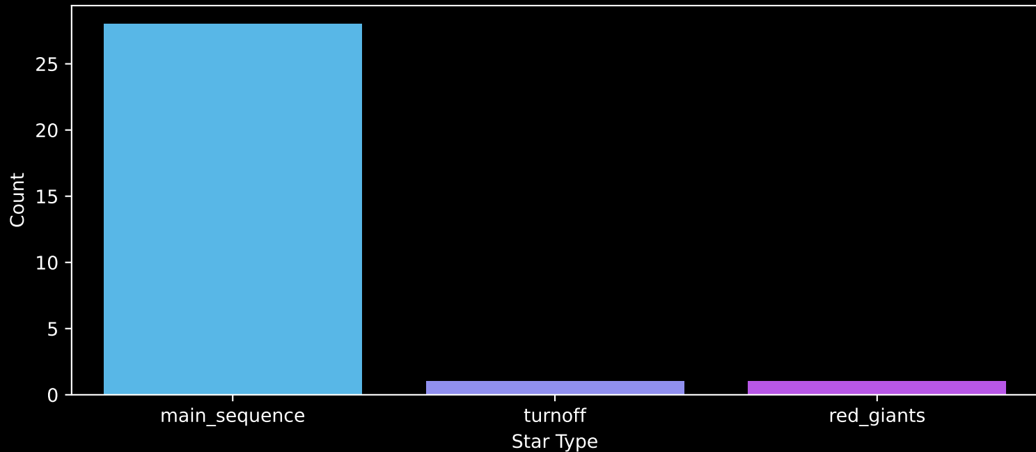
Gaia Stream: [New-26] Count plot of Star Type
