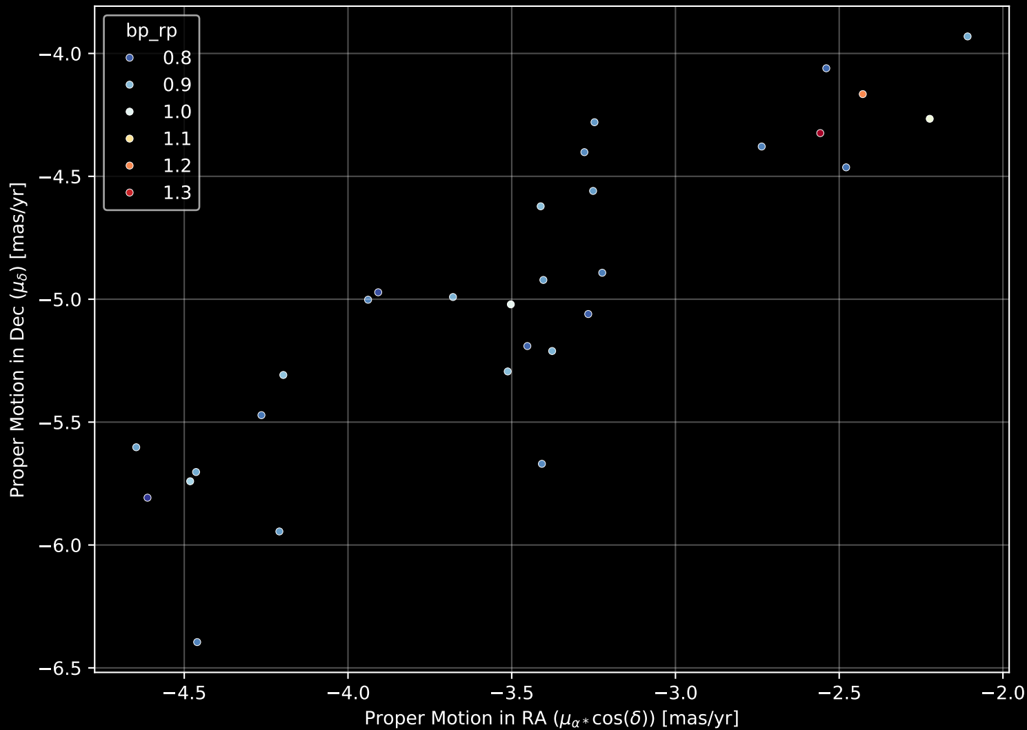
Gaia Stream: [New-26] Proper Motion Diagram (n= 30)
