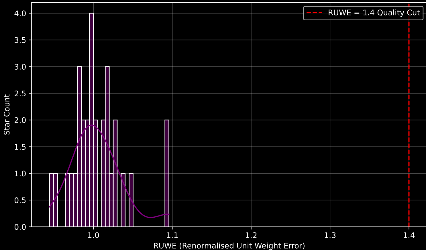
Gaia Stream: [New-26] RUWE Distribution (n= 30)
