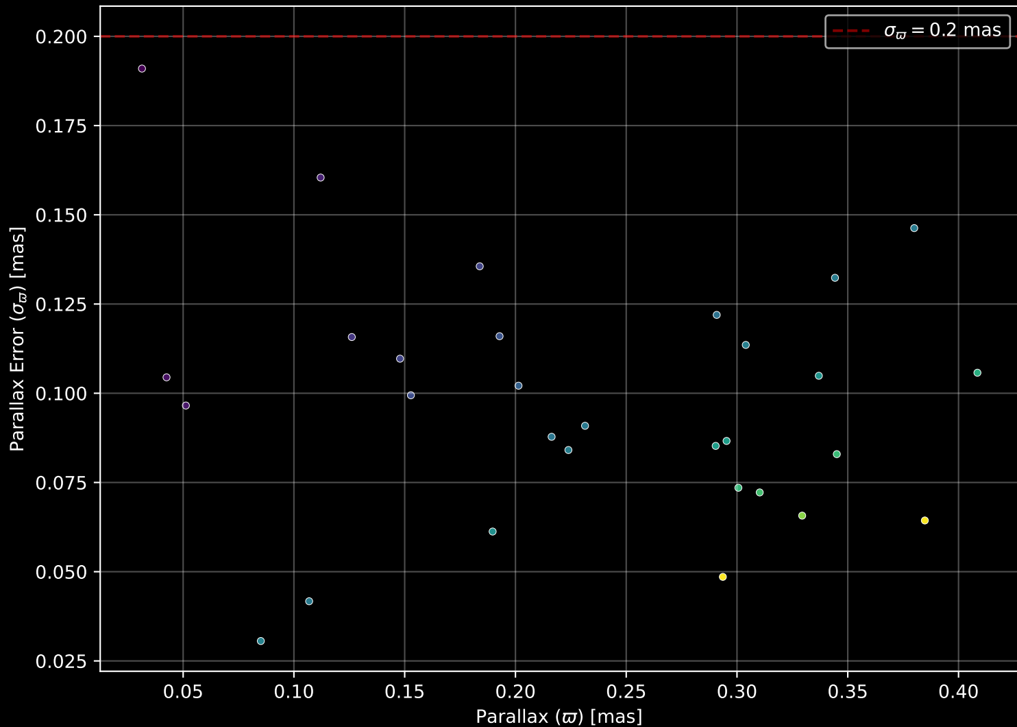
Gaia Stream: [New-26] Parallax Quality (n= 30)
