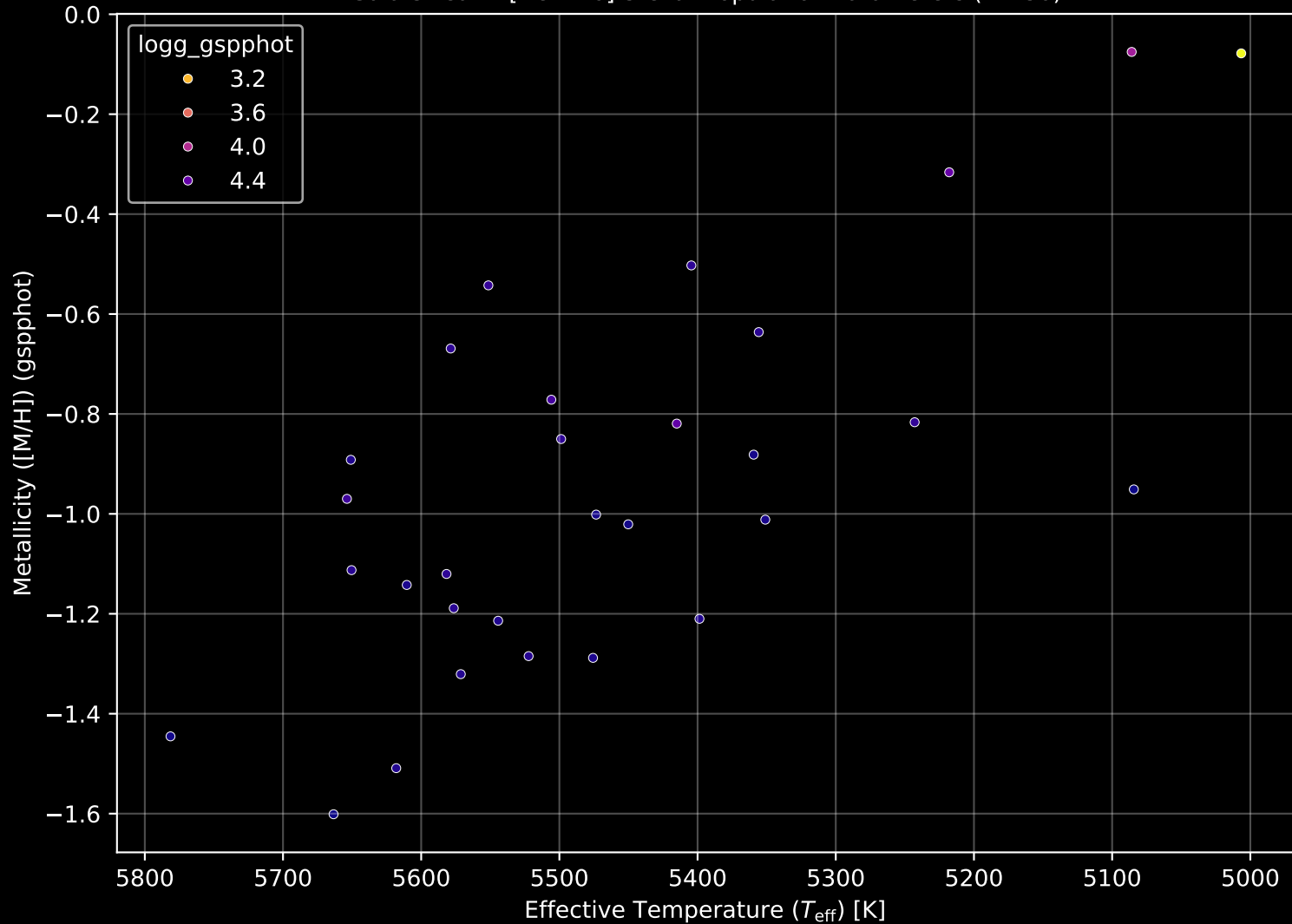
Gaia Stream: [New-26] Stellar Population Parameters (n= 30)
