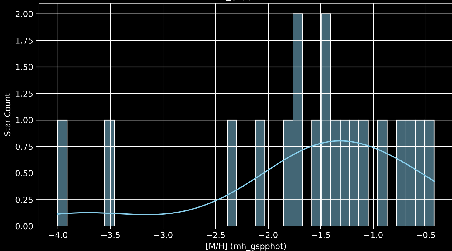
Gaia Stream: [New-27 [M/H] (mh_gspphot) (n= 19)
