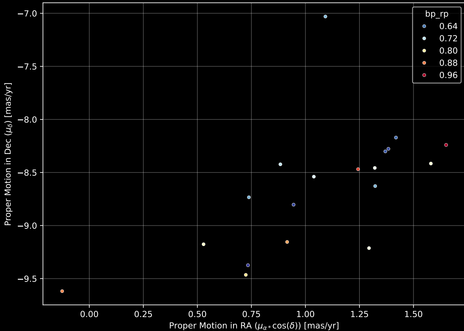
Gaia Stream: [New-27] Proper Motion Diagram (n= 19)
