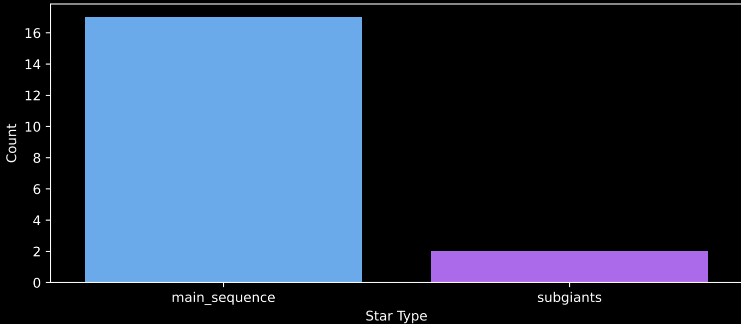
Gaia Stream: [New-27] Count plot of Star Type
