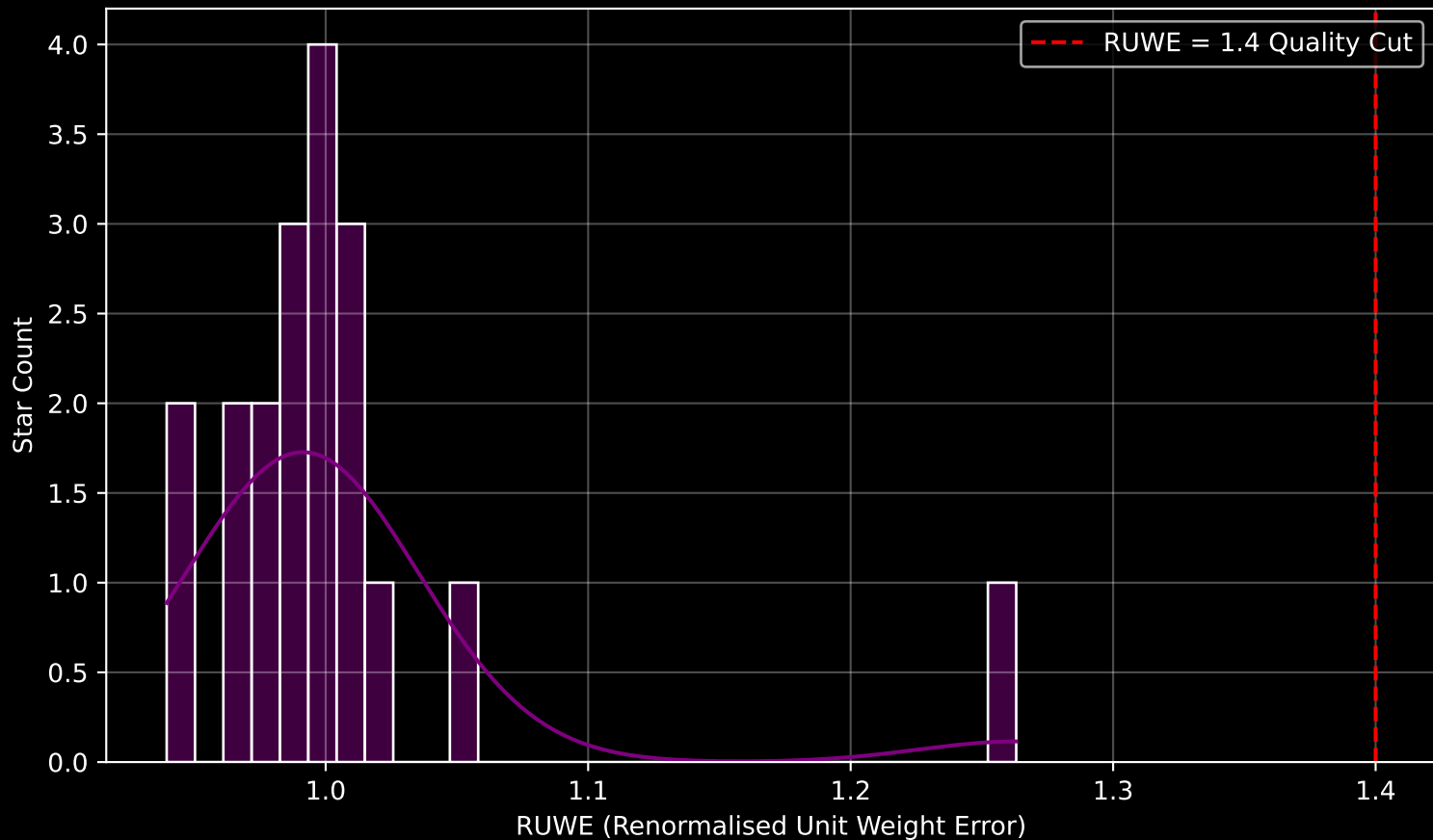
Gaia Stream: [New-27] RUWE Distribution (n= 19)
