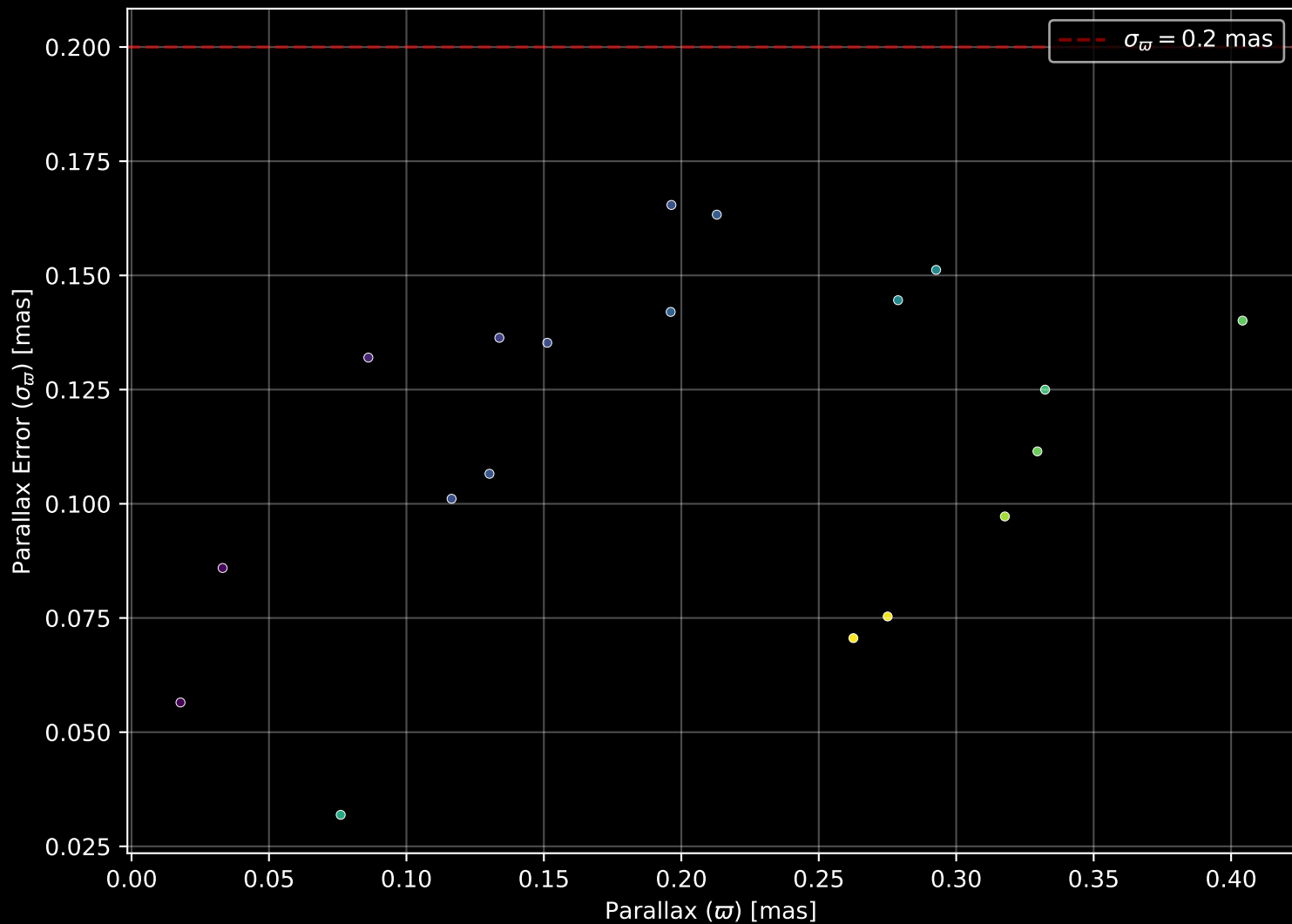
Gaia Stream: [New-27] Parallax Quality (n= 19)
