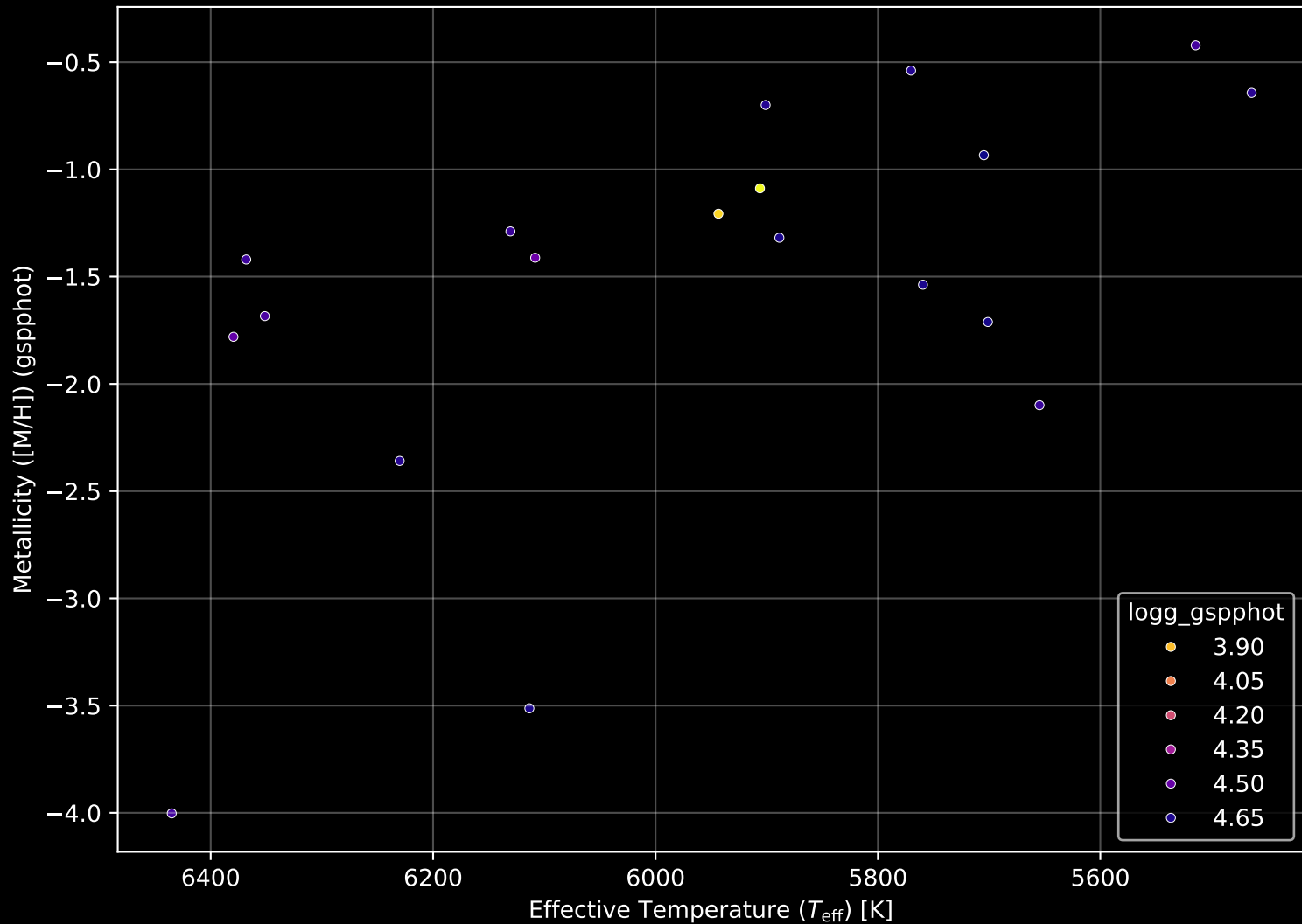
Gaia Stream: [New-27] Stellar Population Parameters (n= 19)
