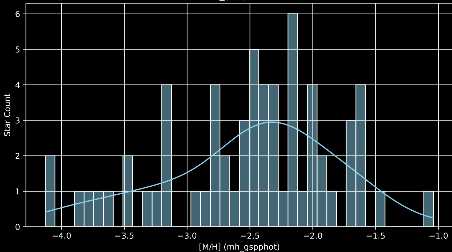
Gaia Stream: [New-3 [M/H] (mh_gspphot) (n= 63)
