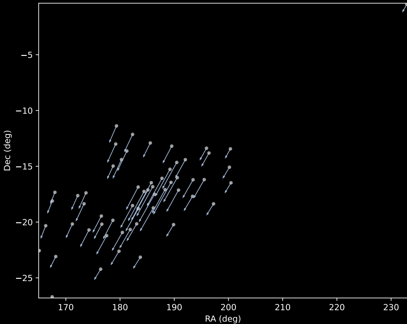
Gaia DR3 Cluster 1 Proper Motion Vectors (n=57)
