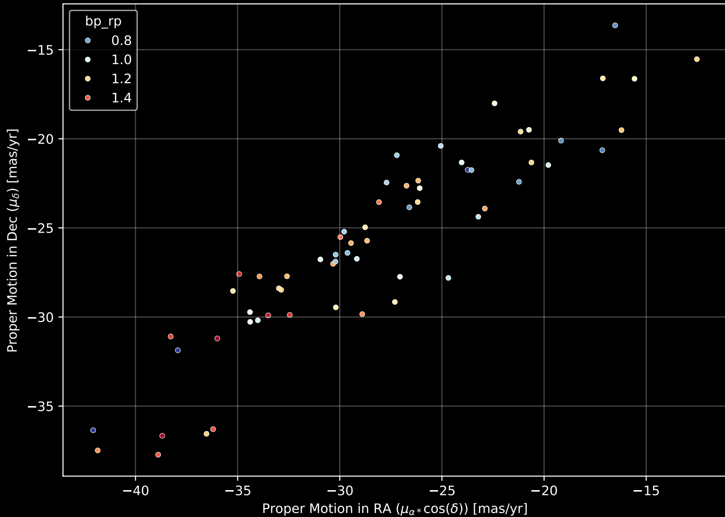
Gaia Stream: [New-3] Proper Motion Diagram (n= 63)
