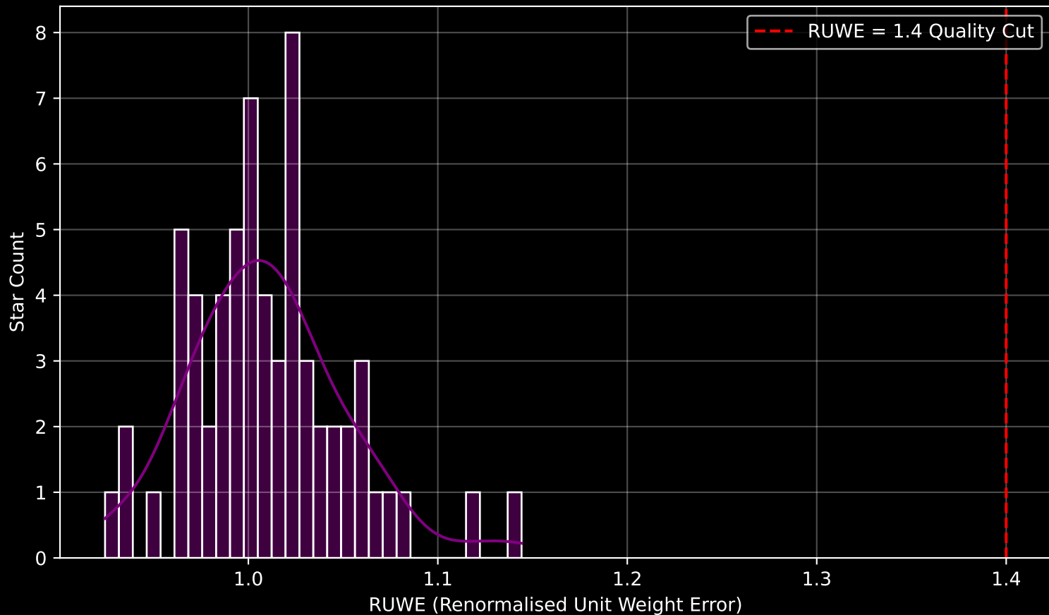
Gaia Stream: [New-3] RUWE Distribution (n= 63)
