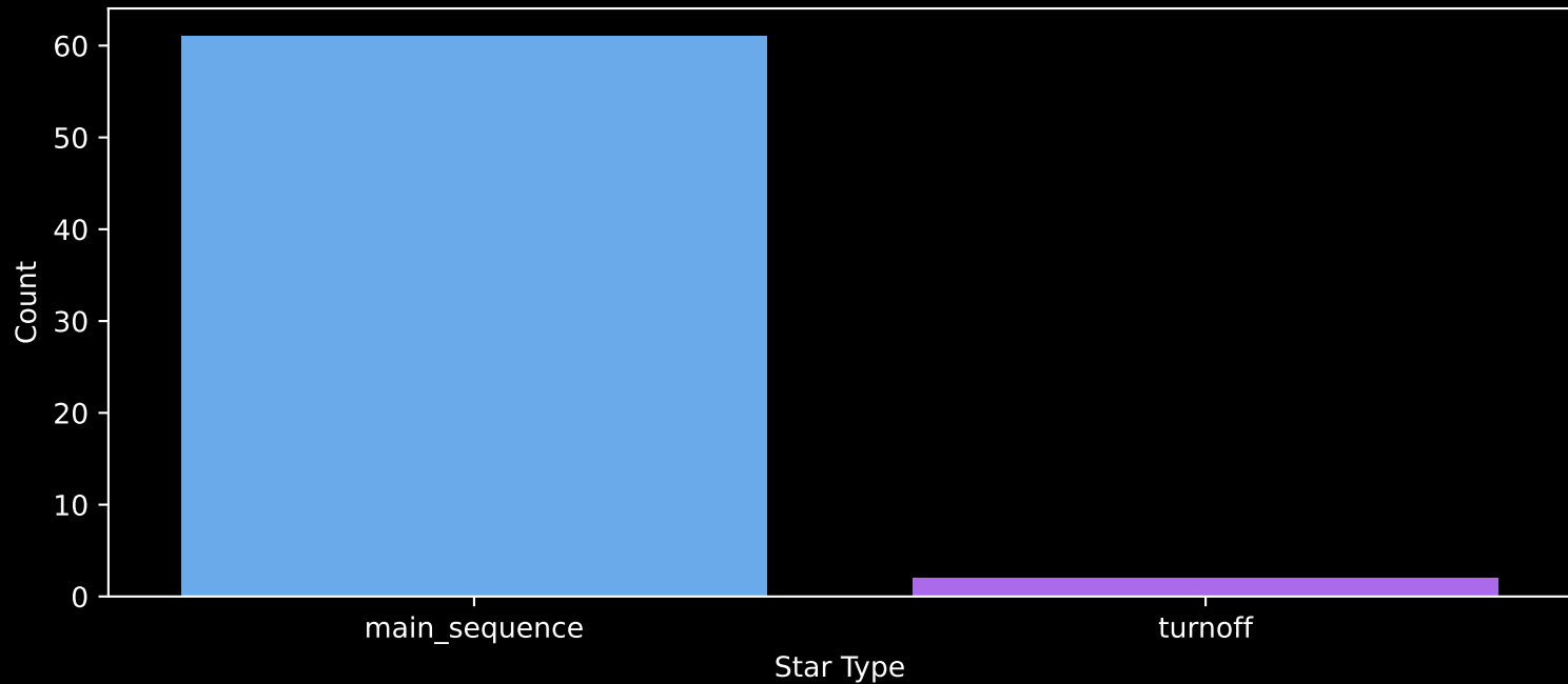
Gaia Stream: [New-3] Count plot of Star Type
