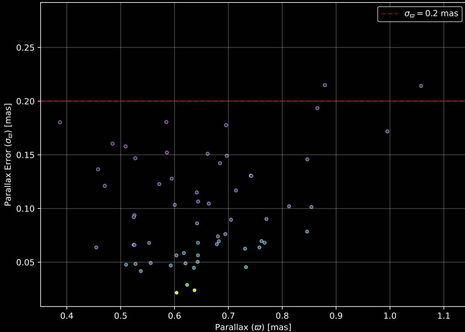
Gaia Stream: [New-3] Parallax Quality (n= 63)
