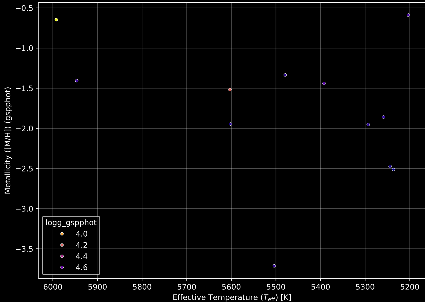
Gaia Stream: [New-4] Stellar Population Parameters (n= 12)
