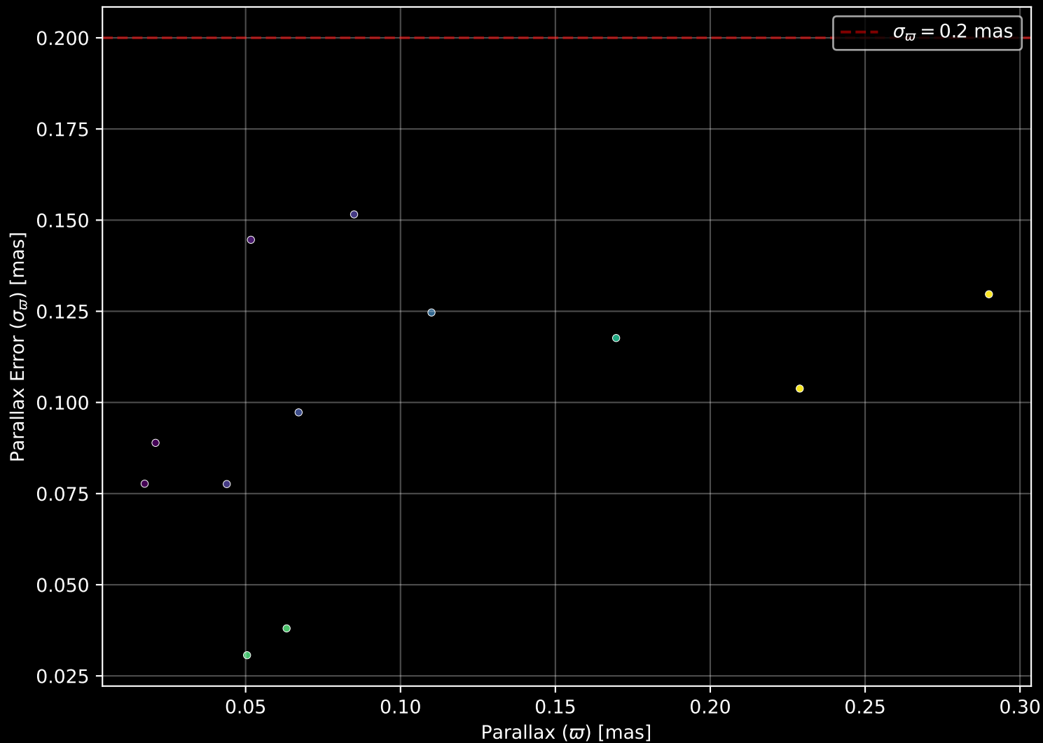
Gaia Stream: [New-4] Parallax Quality (n= 12)
