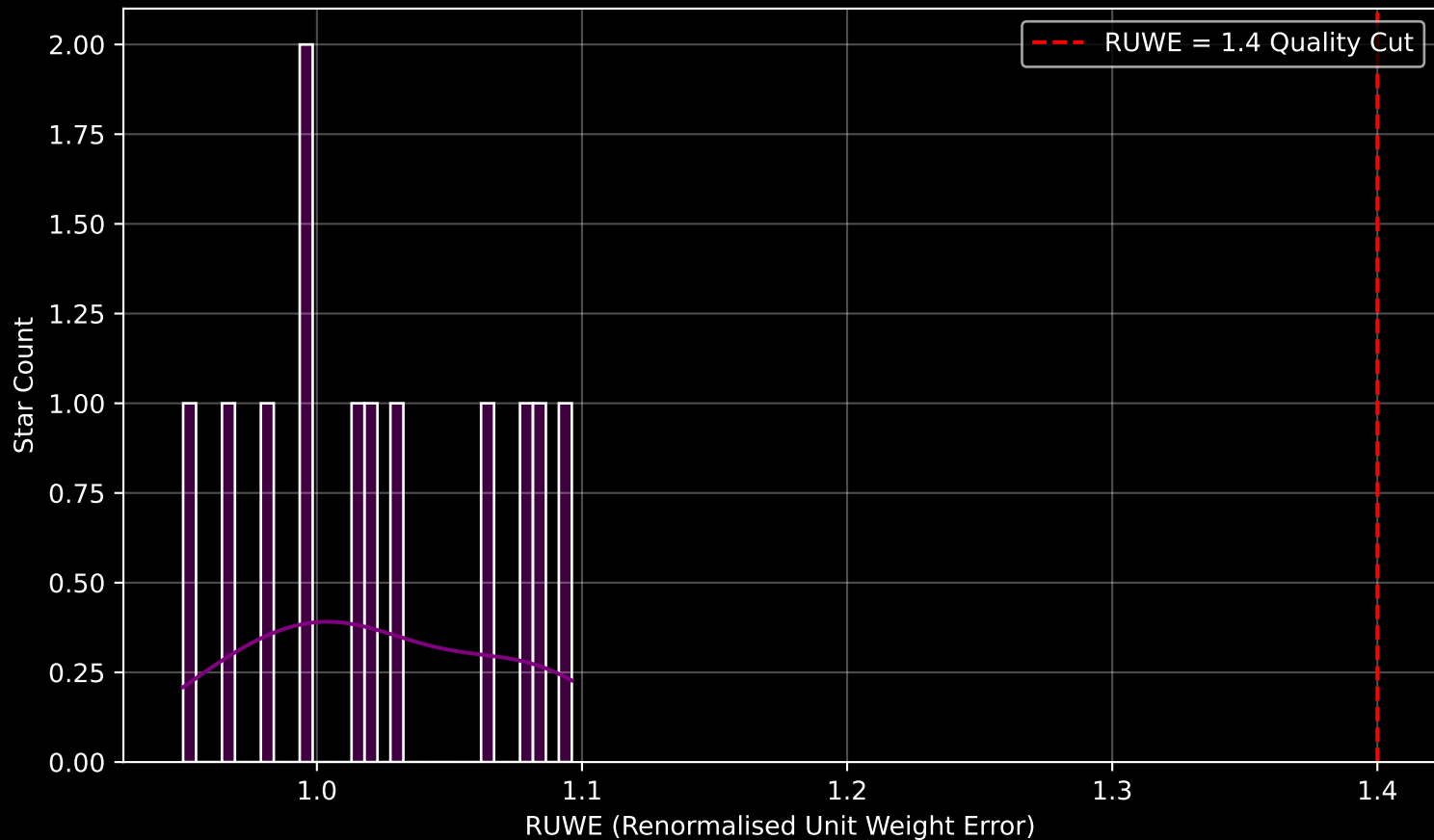
Gaia Stream: [New-4] RUWE Distribution (n= 12)
