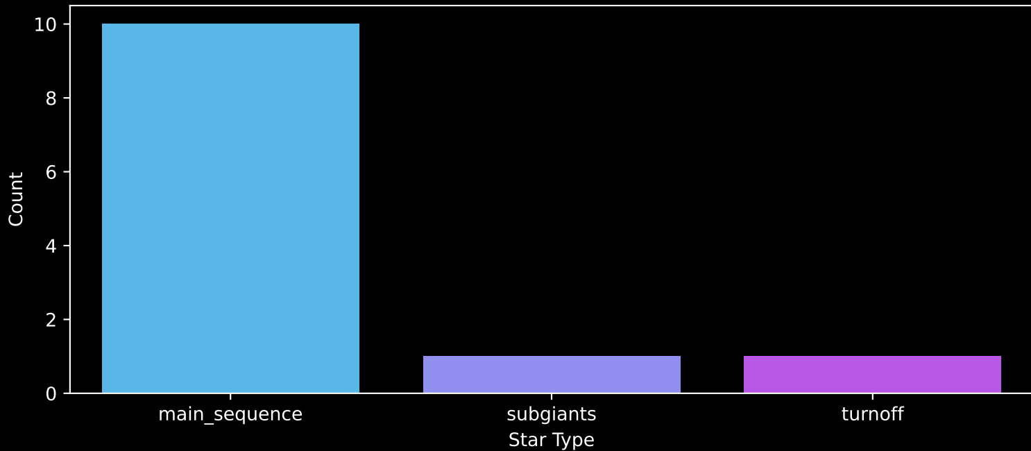
Gaia Stream: [New-4] Count plot of Star Type
