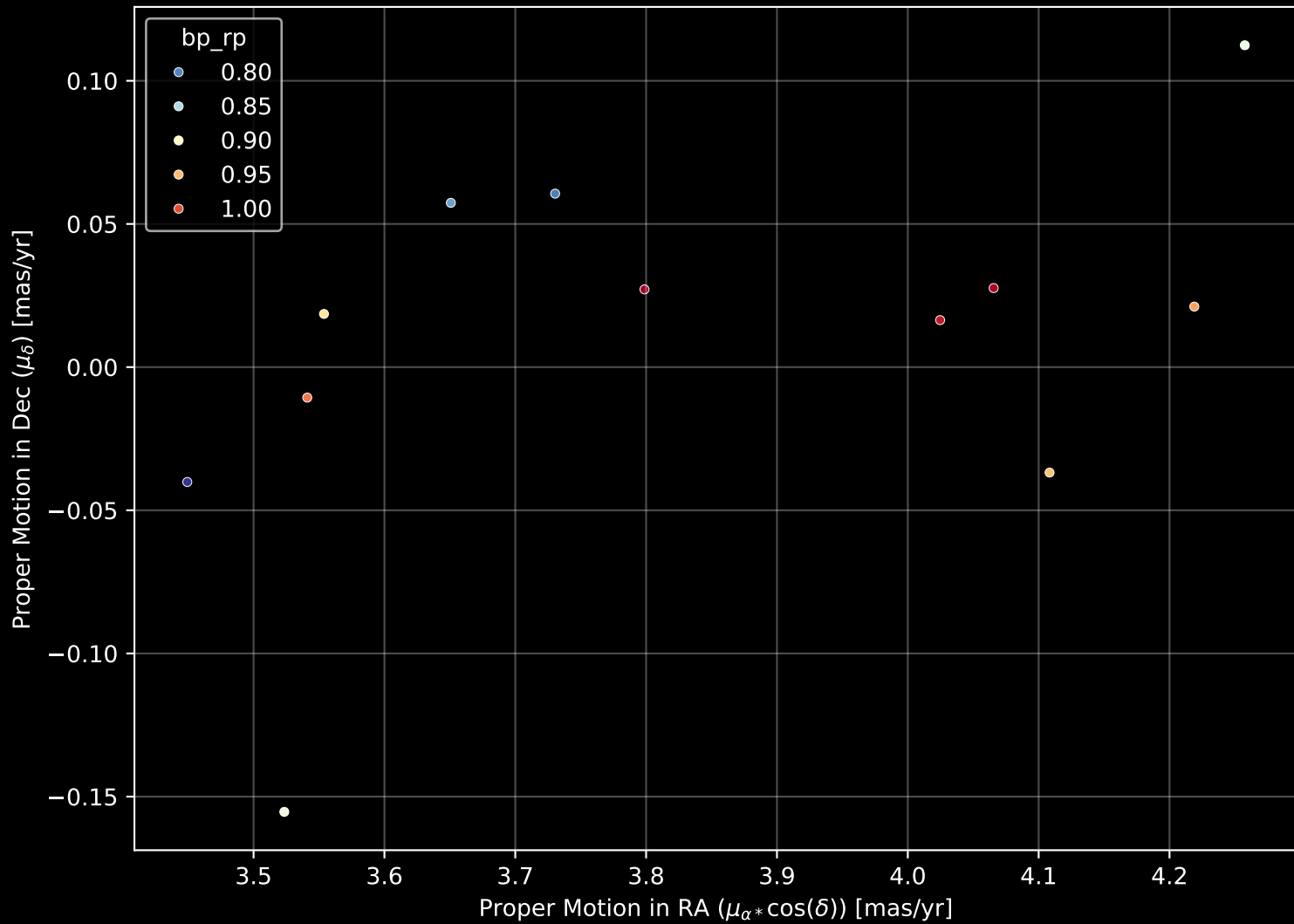
Gaia Stream: [New-4] Proper Motion Diagram (n= 12)
