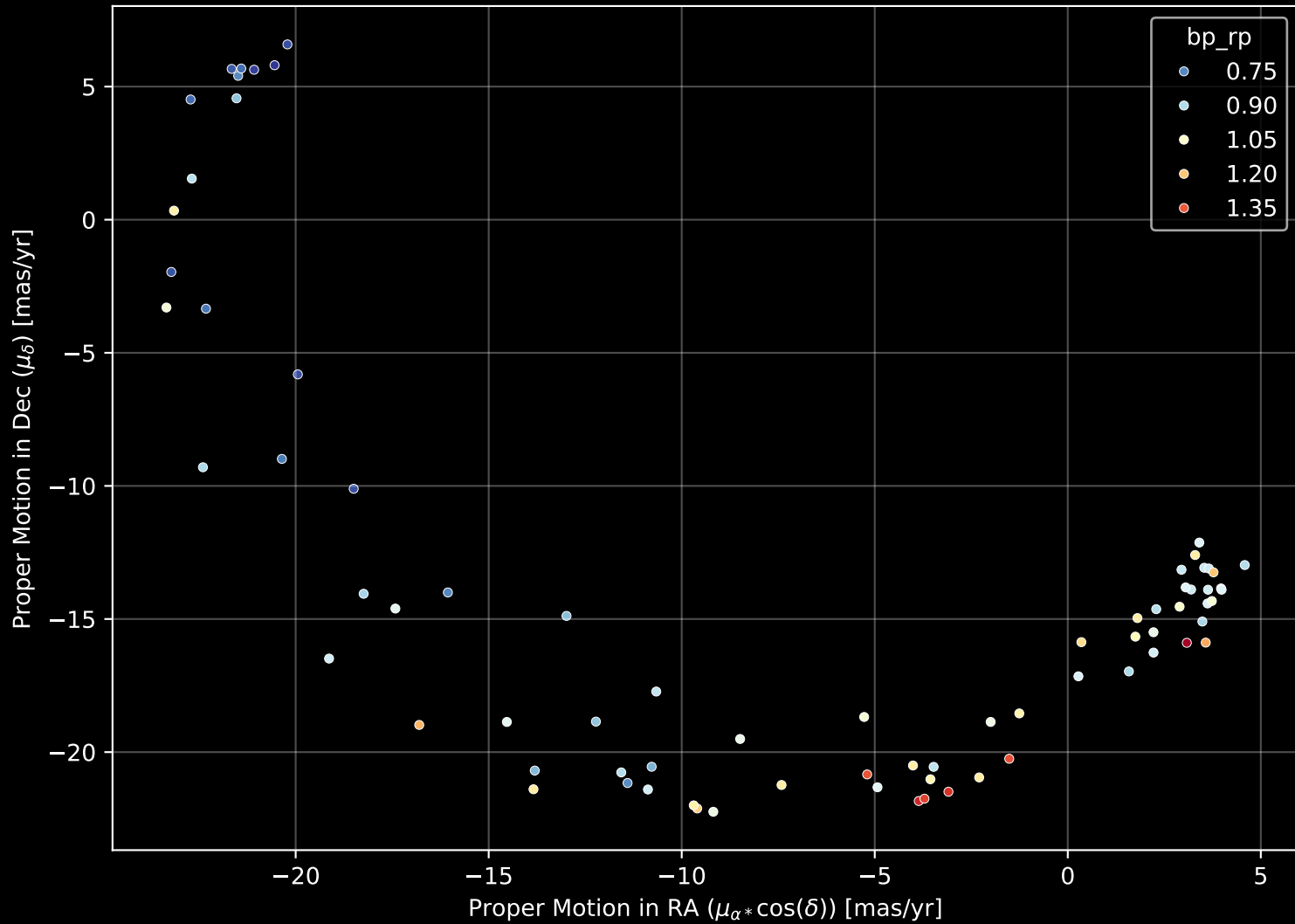
Gaia Stream: [New-6] Proper Motion Diagram (n= 76)
