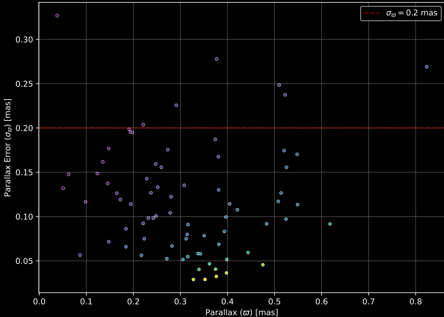
Gaia Stream: [New-6] Parallax Quality (n= 76)
