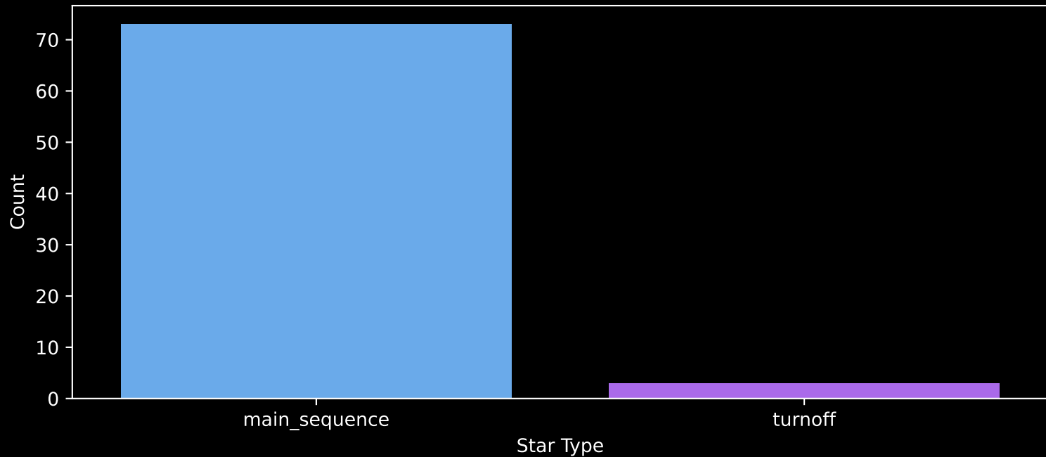
Gaia Stream: [New-6] Count plot of Star Type
