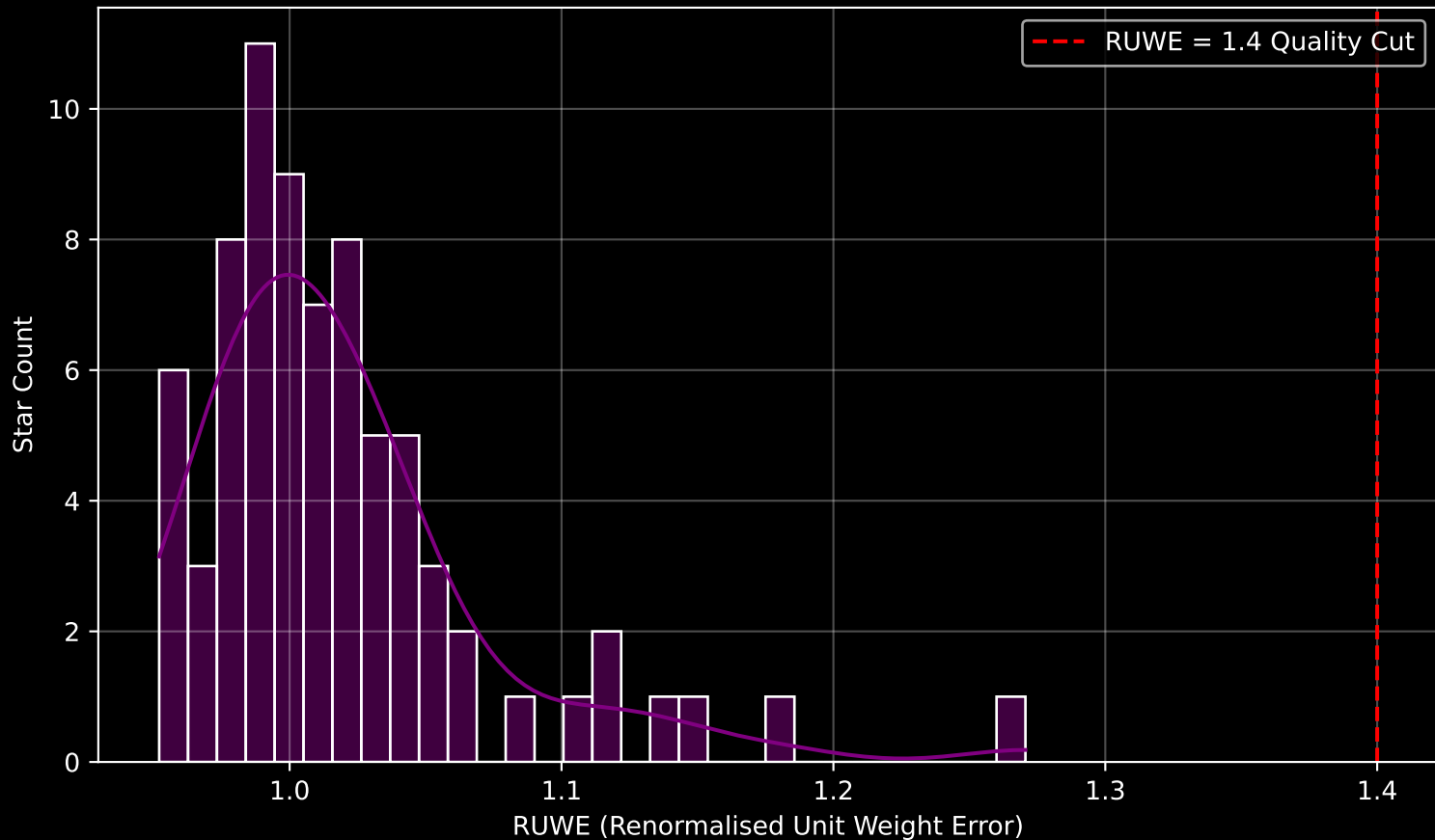
Gaia Stream: [New-6] RUWE Distribution (n= 75)
