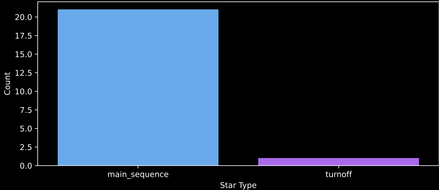
Gaia Stream: [New-7] Count plot of Star Type
