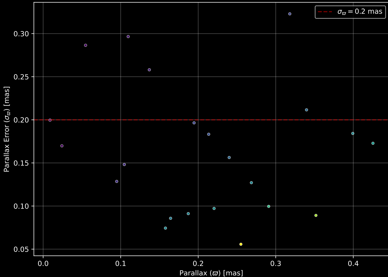
Gaia Stream: [New-7] Parallax Quality (n= 22)
