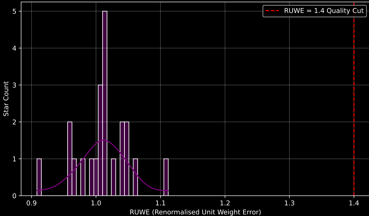
Gaia Stream: [New-7] RUWE Distribution (n= 22)
