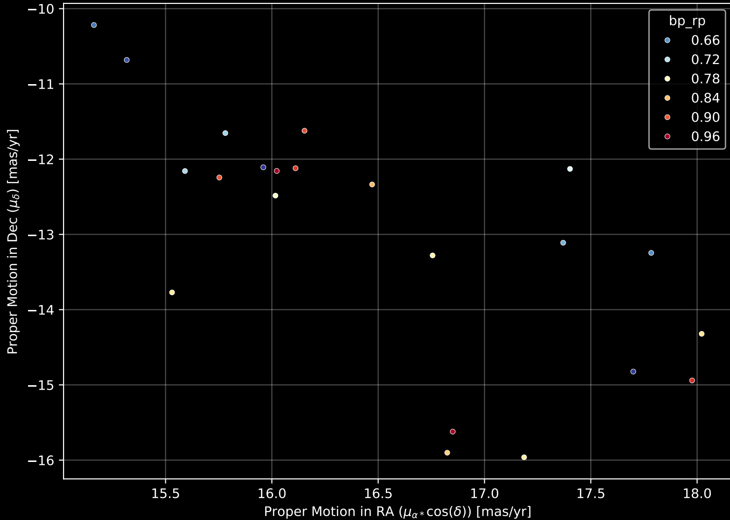
Gaia Stream: [New-7] Proper Motion Diagram (n= 22)
