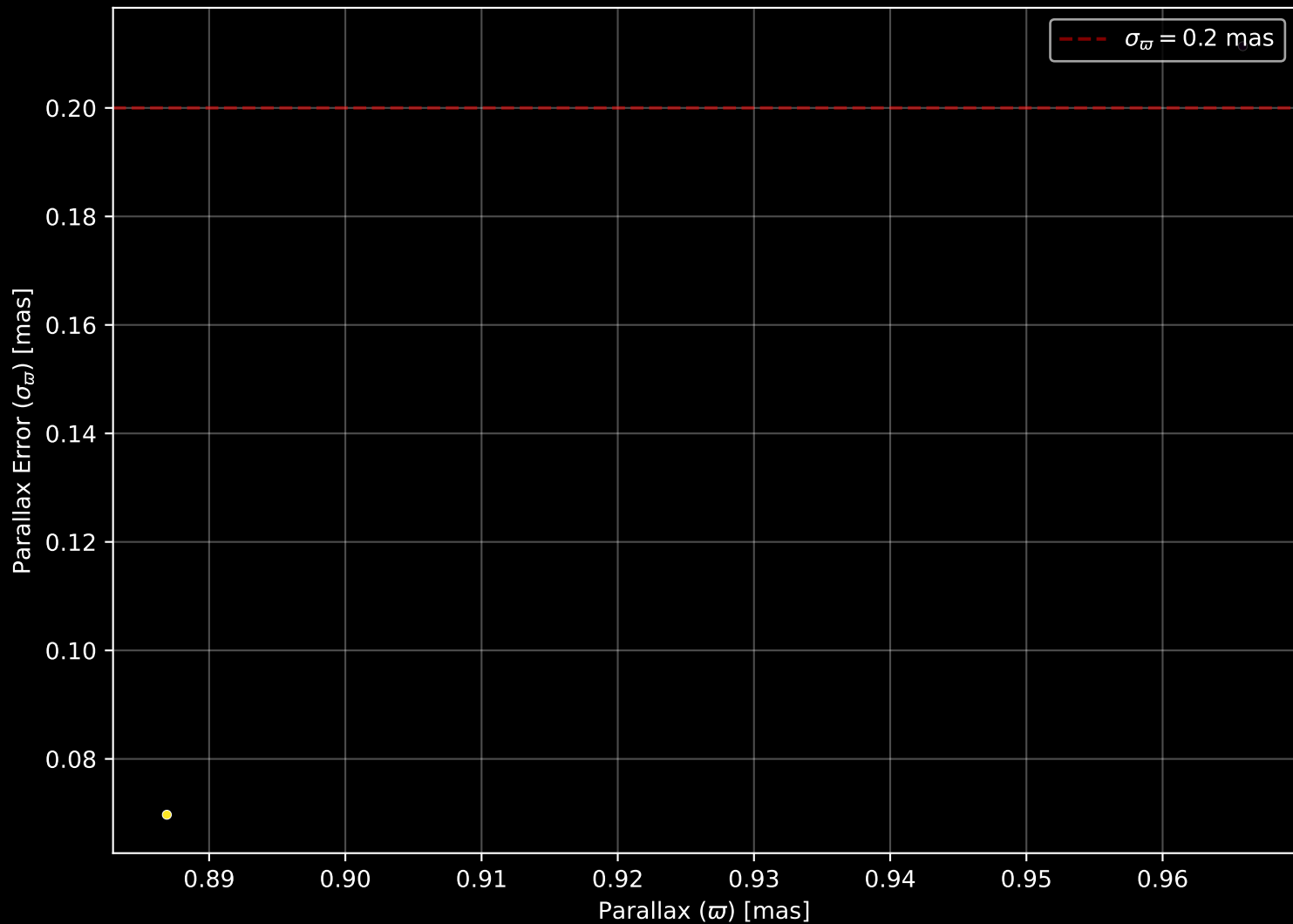
Gaia Stream: [New-8] Parallax Quality (n= 2)
