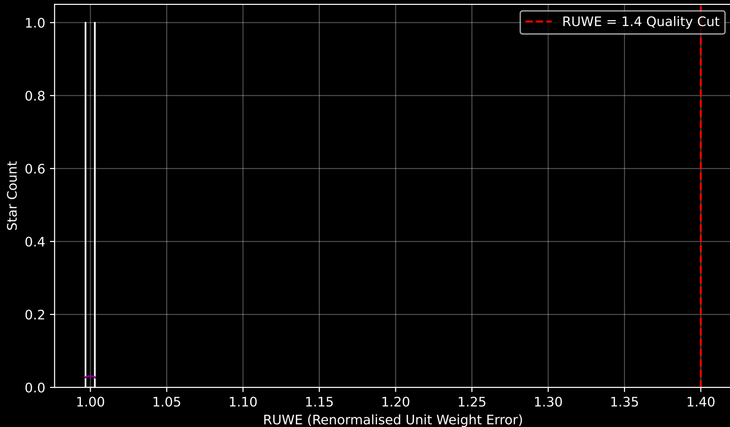
Gaia Stream: [New-8] RUWE Distribution (n= 2)
