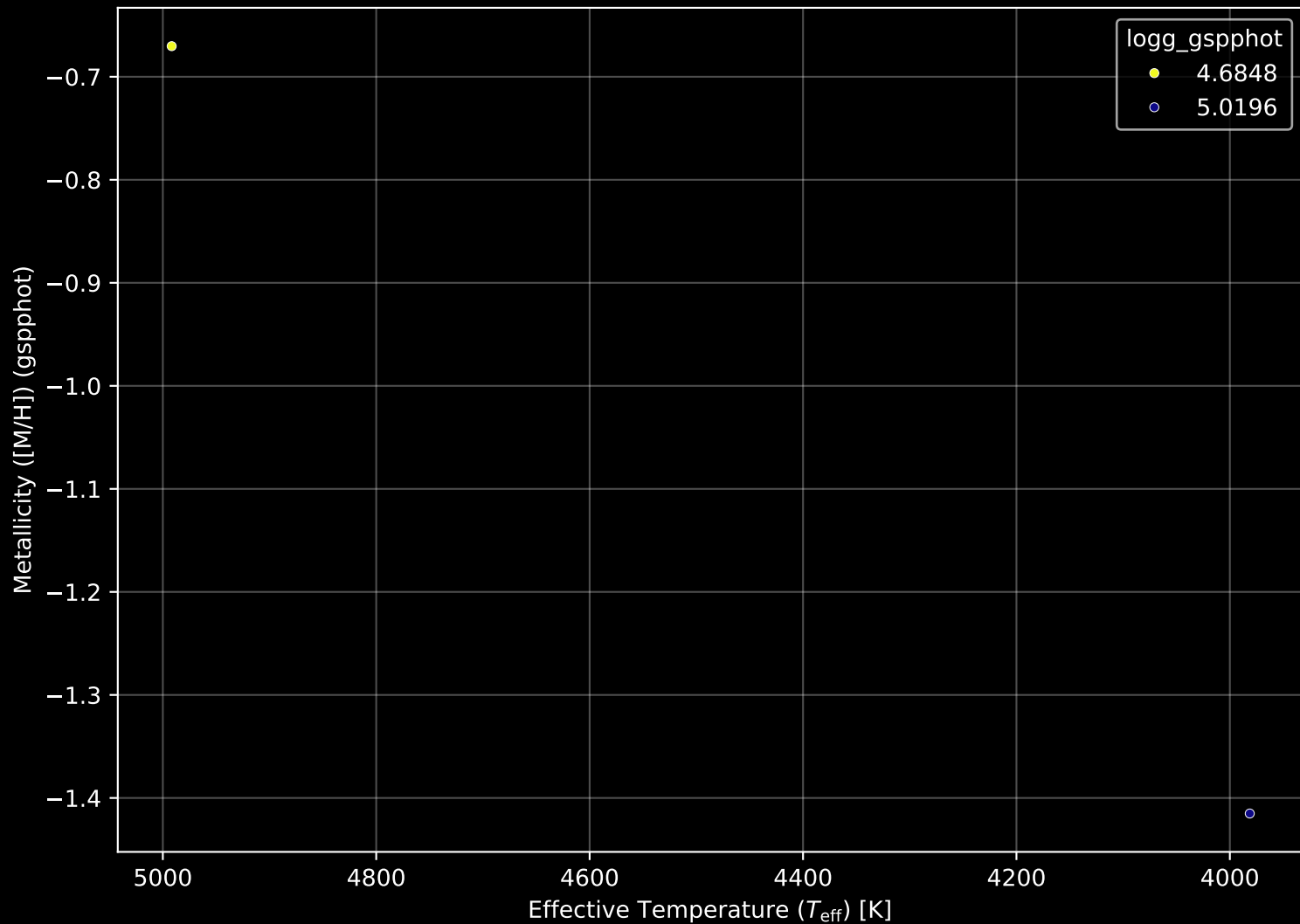
Gaia Stream: [New-8] Stellar Population Parameters (n= 2)
