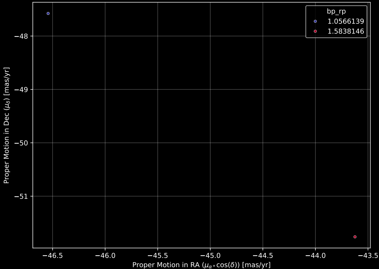
Gaia Stream: [New-8] Proper Motion Diagram (n= 2)
