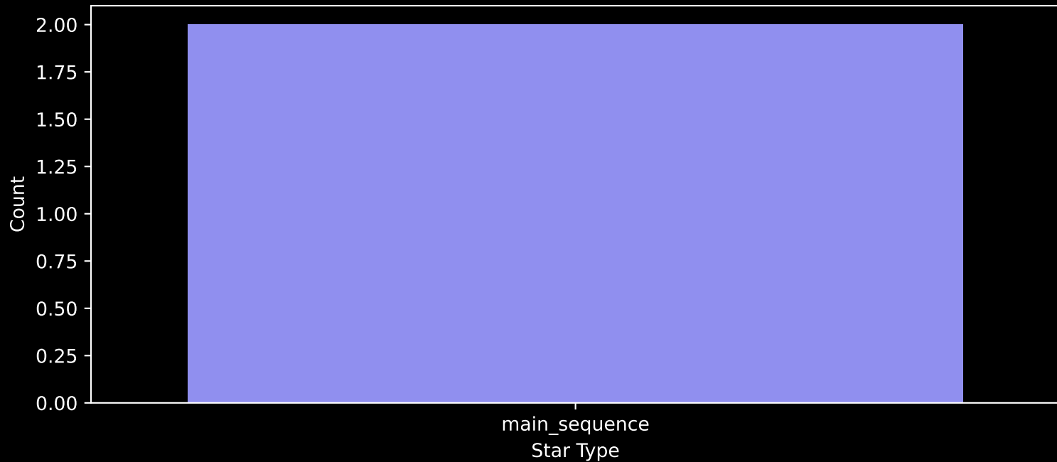
Gaia Stream: [New-8] Count plot of Star Type
