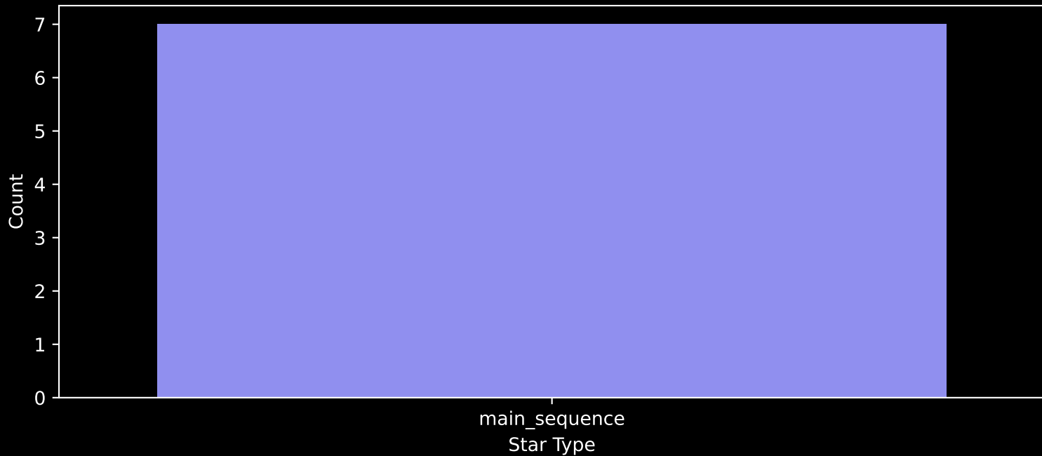
Gaia Stream: [Ophiuchus] Count plot of Star Type
