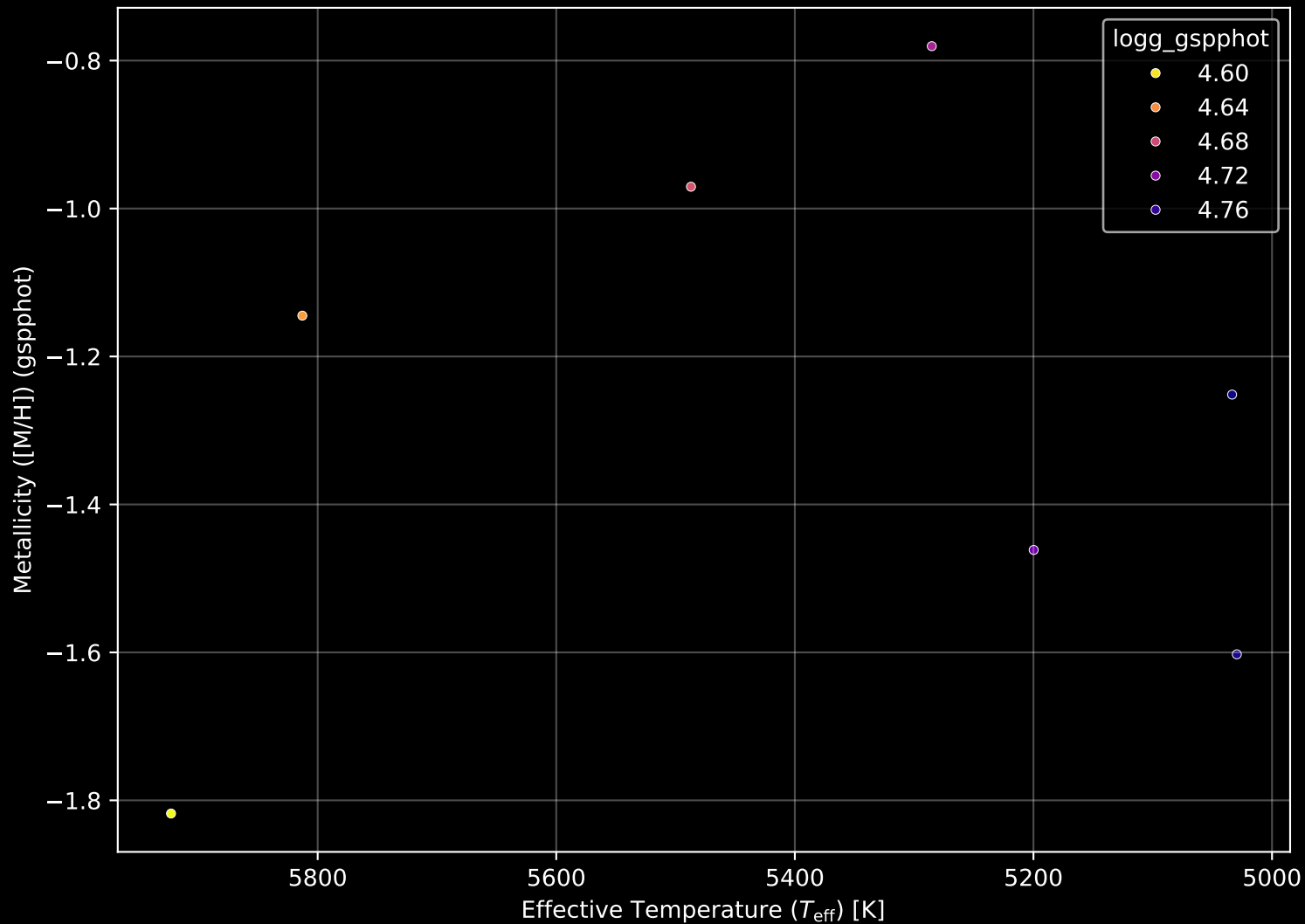
Gaia Stream: [Ophiuchus] Stellar Population Parameters (n= 7)
