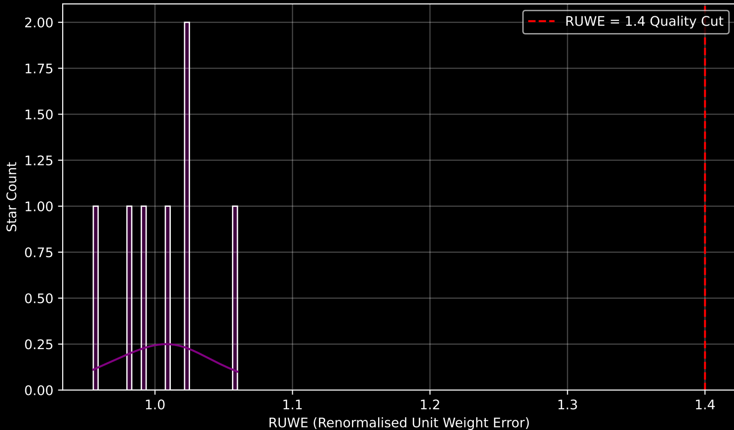
Gaia Stream: [Ophiuchus] RUWE Distribution (n= 7)
