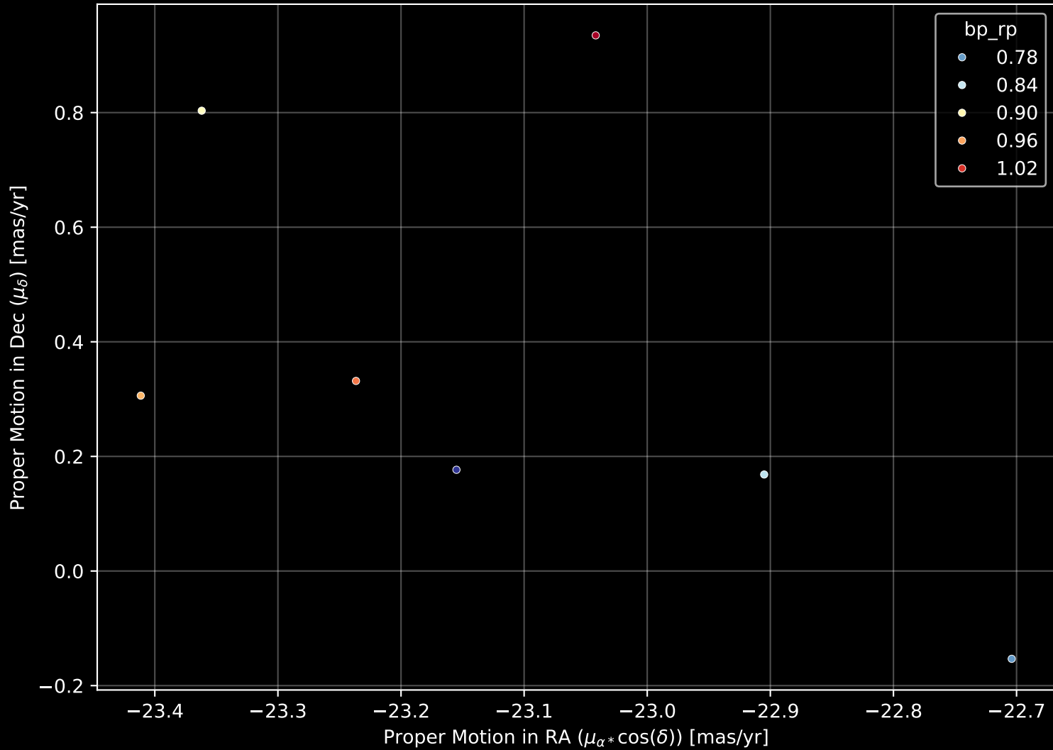
Gaia Stream: [Ophiuchus] Proper Motion Diagram (n= 7)
