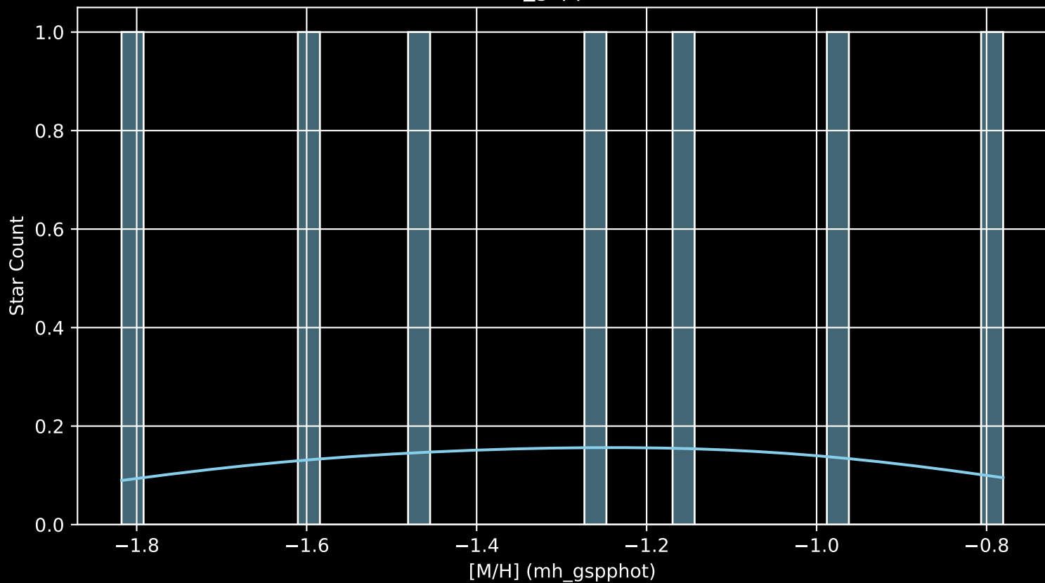
Gaia Stream: [Ophiuchus [M/H] (mh_gspphot) (n= 7)
