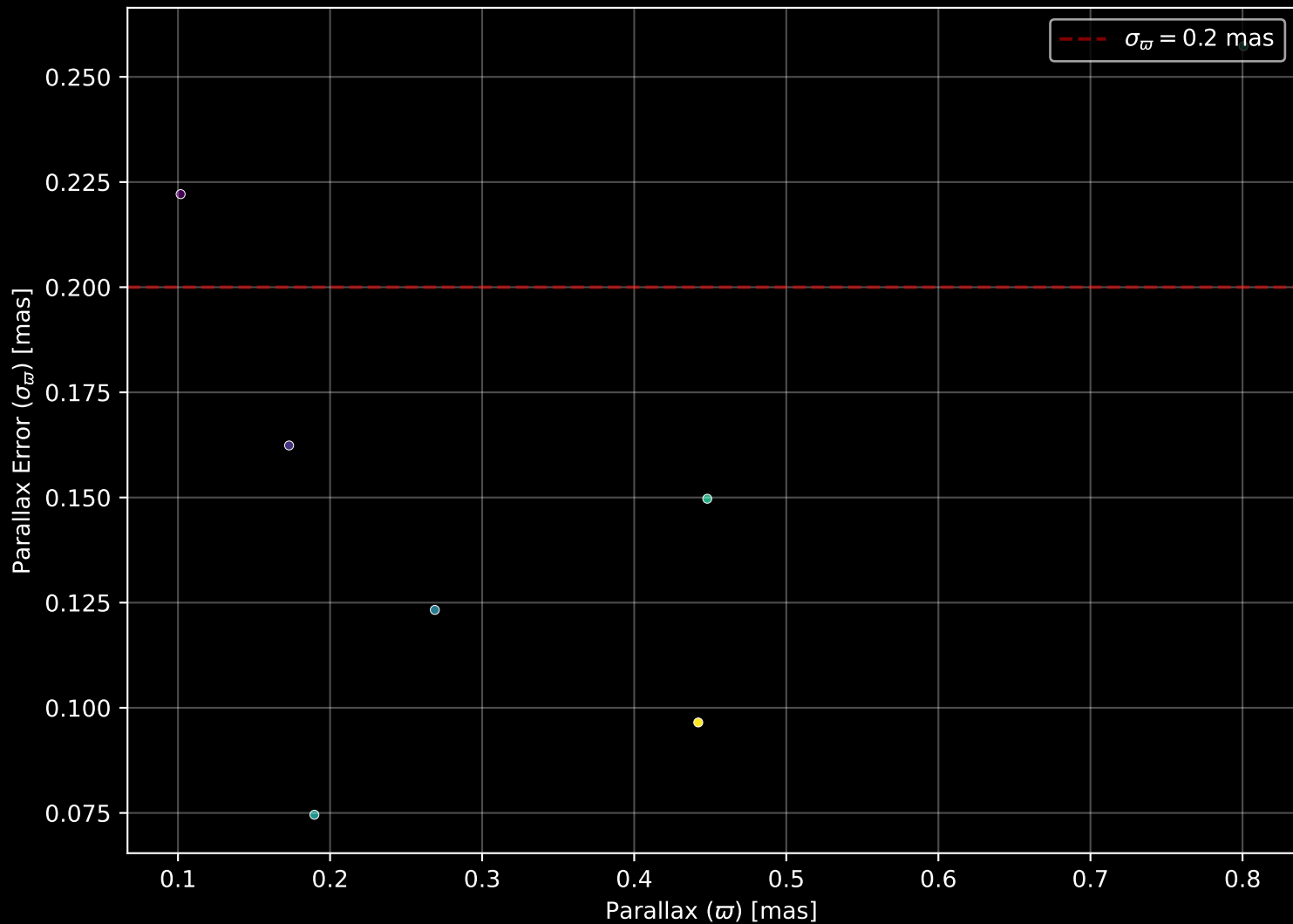
Gaia Stream: [Ophiuchus] Parallax Quality (n= 7)
