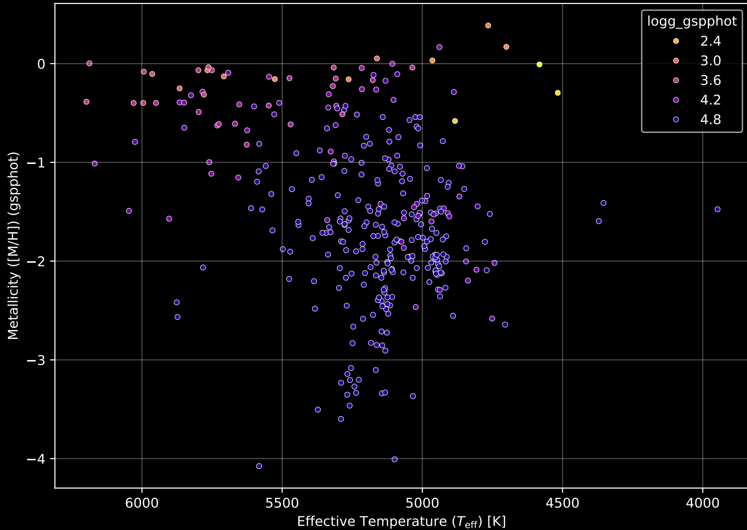
Gaia Stream: [Orphan] Stellar Population Parameters (n= 331)
