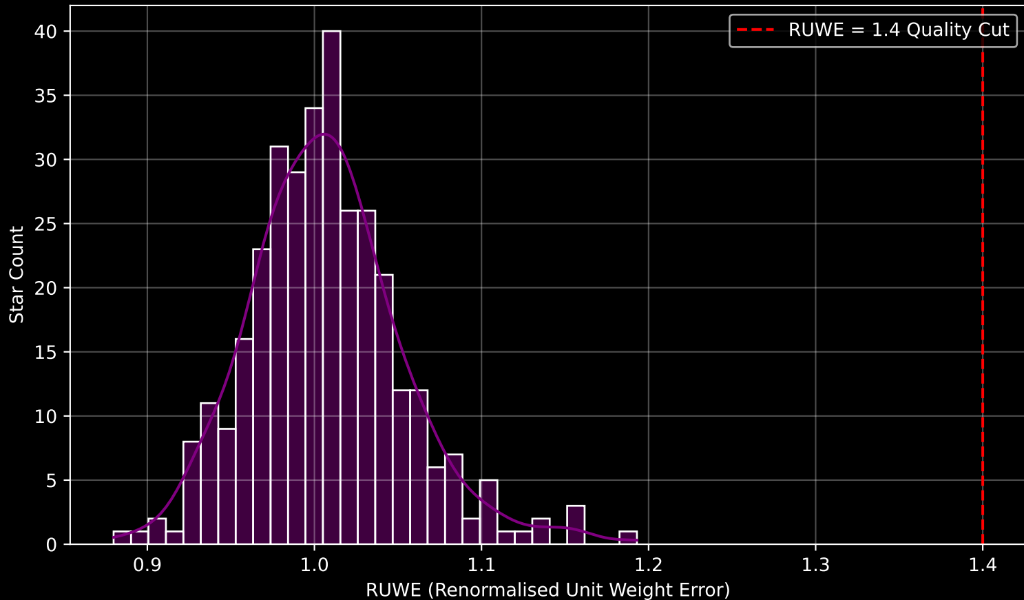
Gaia Stream: [Orphan] RUWE Distribution (n= 331)
