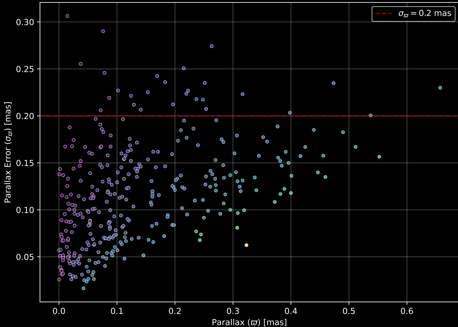
Gaia Stream: [Orphan] Parallax Quality (n= 331)
