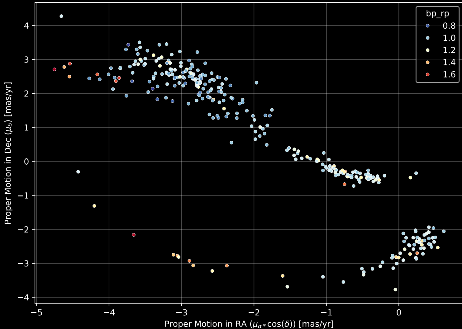
Gaia Stream: [Orphan] Proper Motion Diagram (n= 331)
