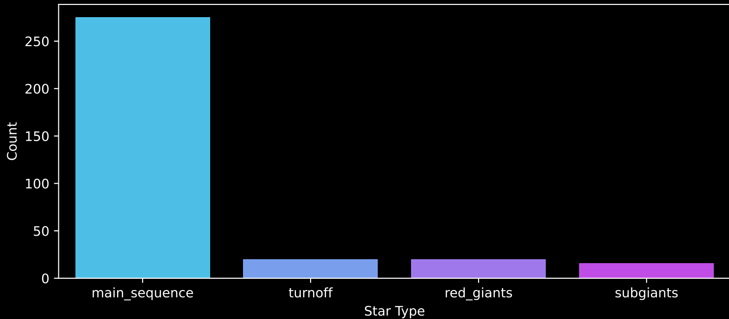
Gaia Stream: [Orphan] Count plot of Star Type
