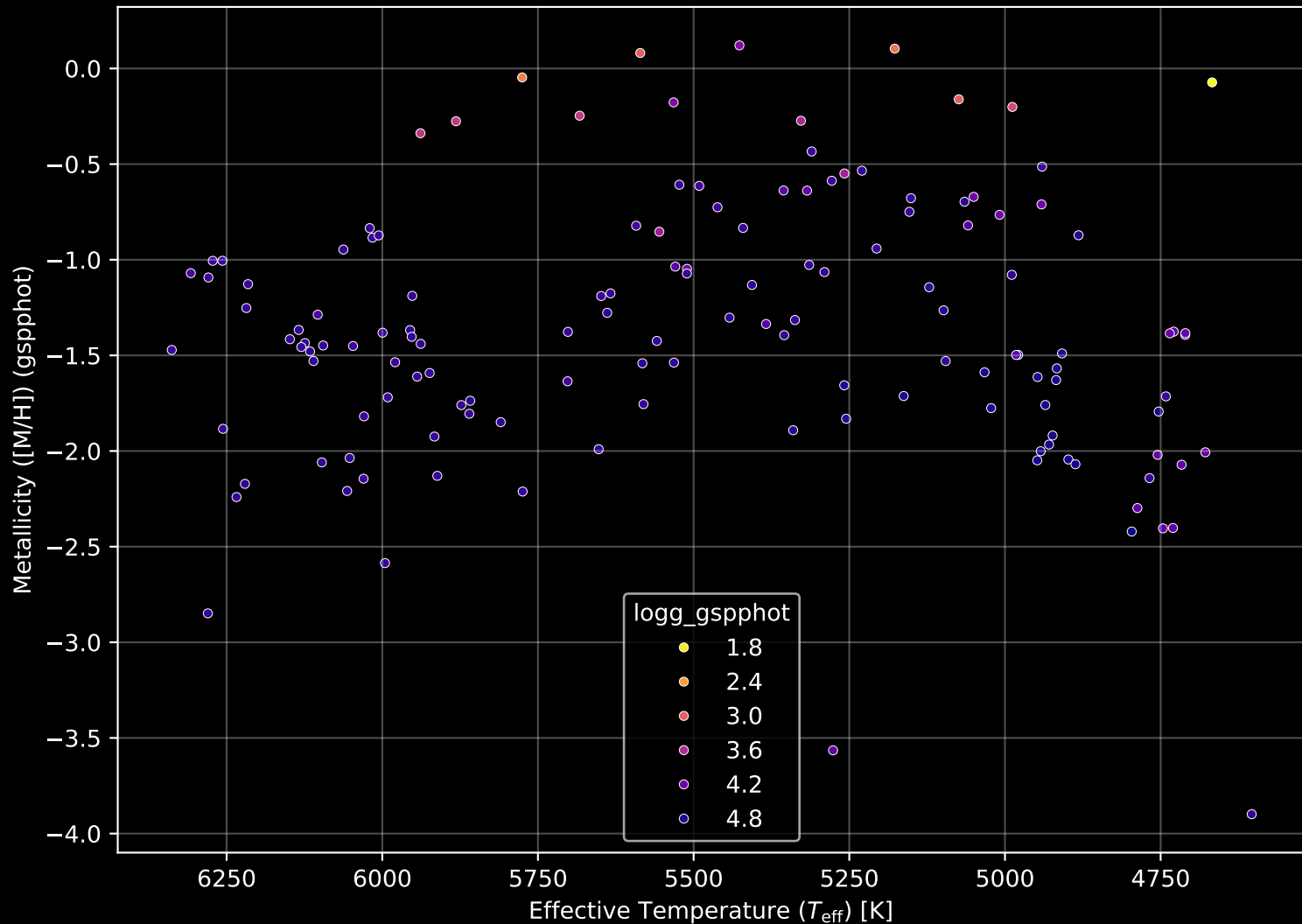
Gaia Stream: [Pal_5] Stellar Population Parameters (n= 139)
