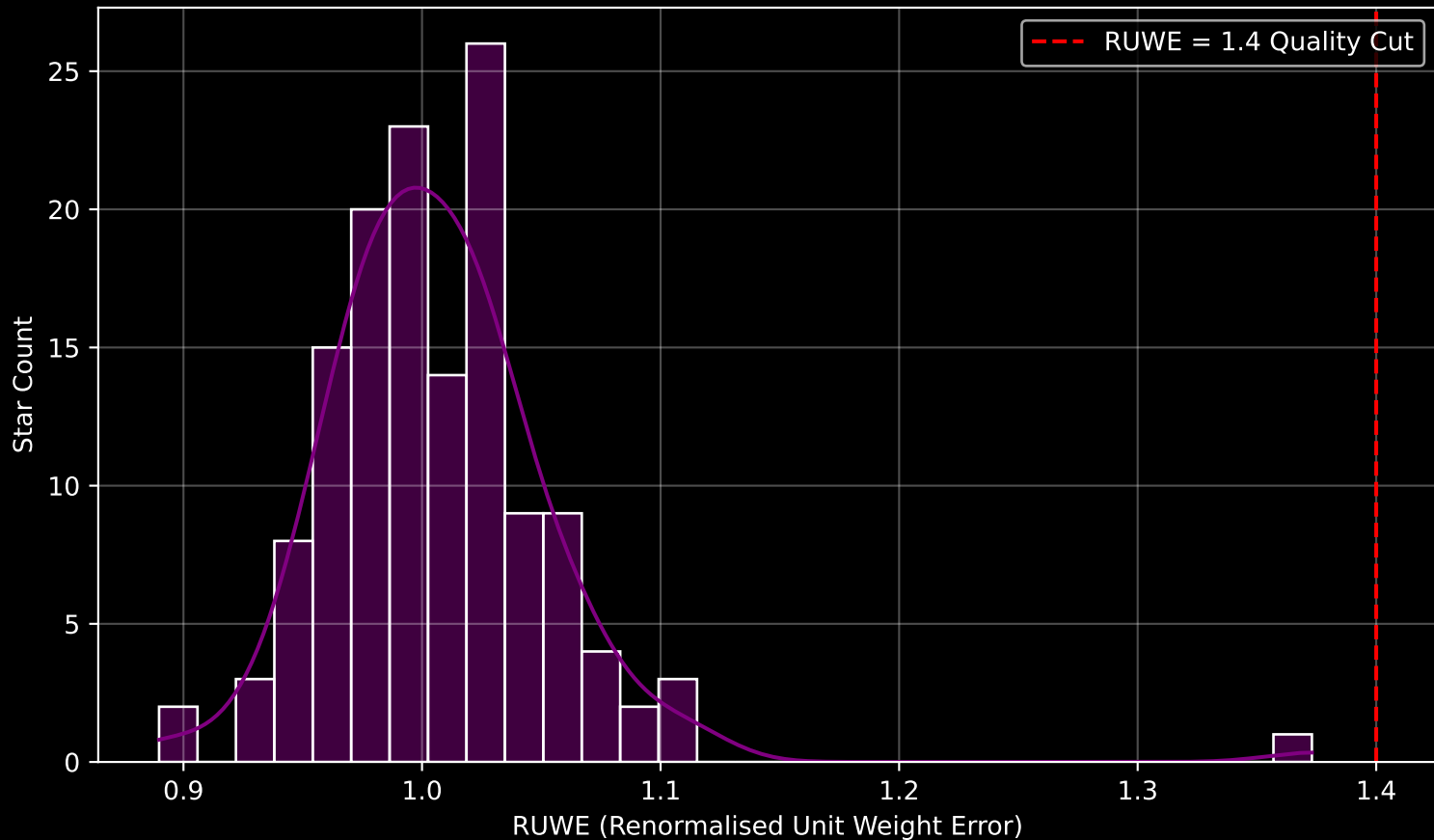
Gaia Stream: [Pal_5] RUWE Distribution (n= 139)
