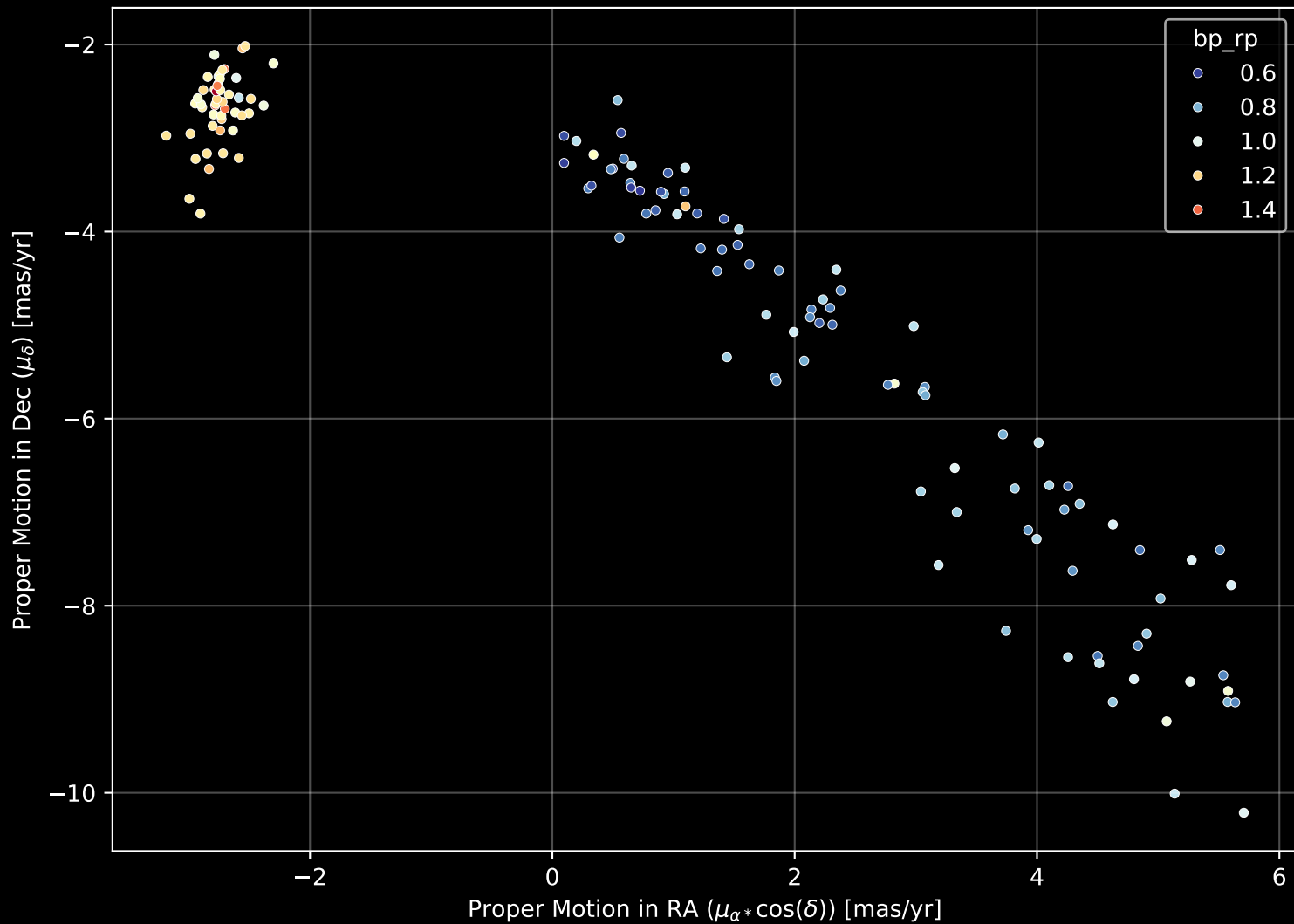
Gaia Stream: [Pal_5] Proper Motion Diagram (n= 139)
