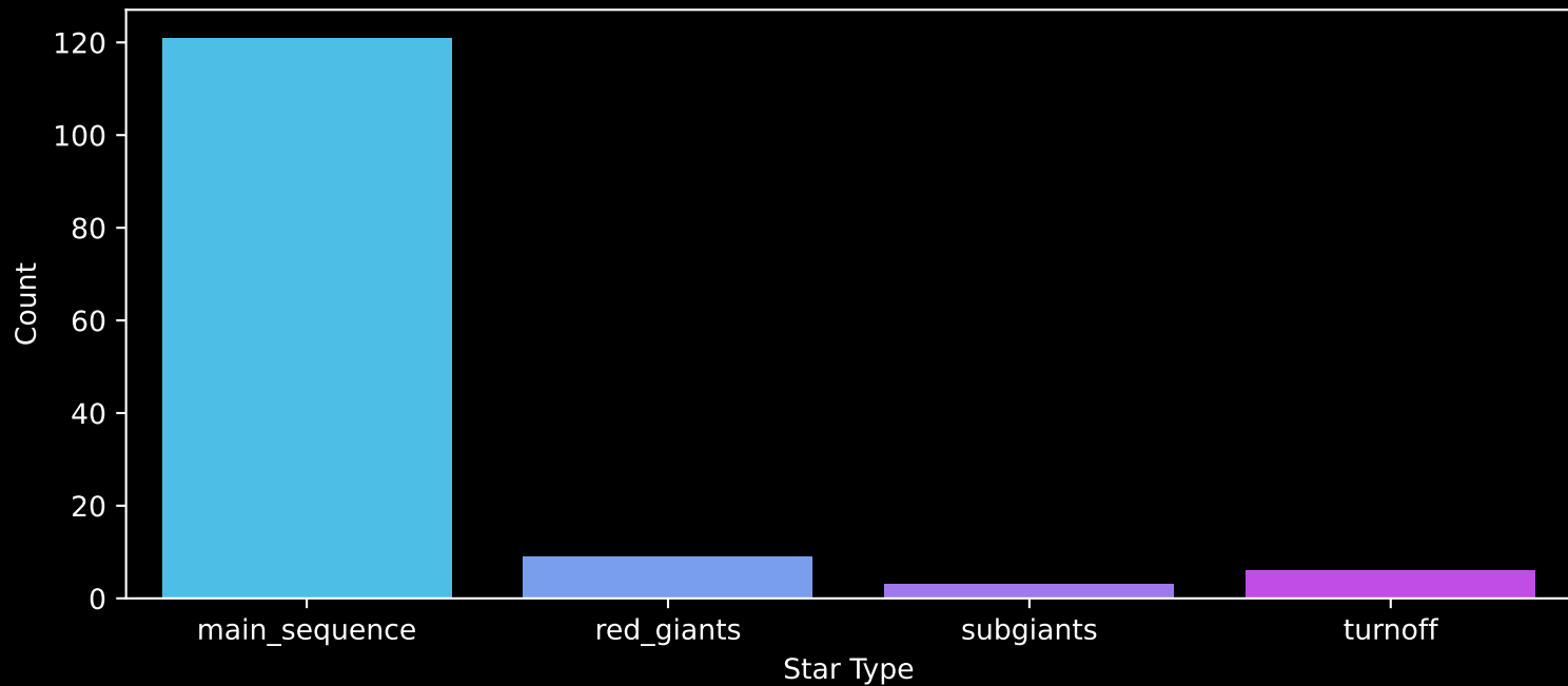
Gaia Stream: [Pal_5] Count plot of Star Type
