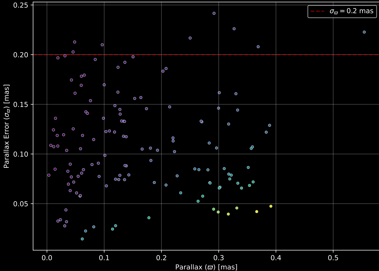
Gaia Stream: [Pal_5] Parallax Quality (n= 139)
