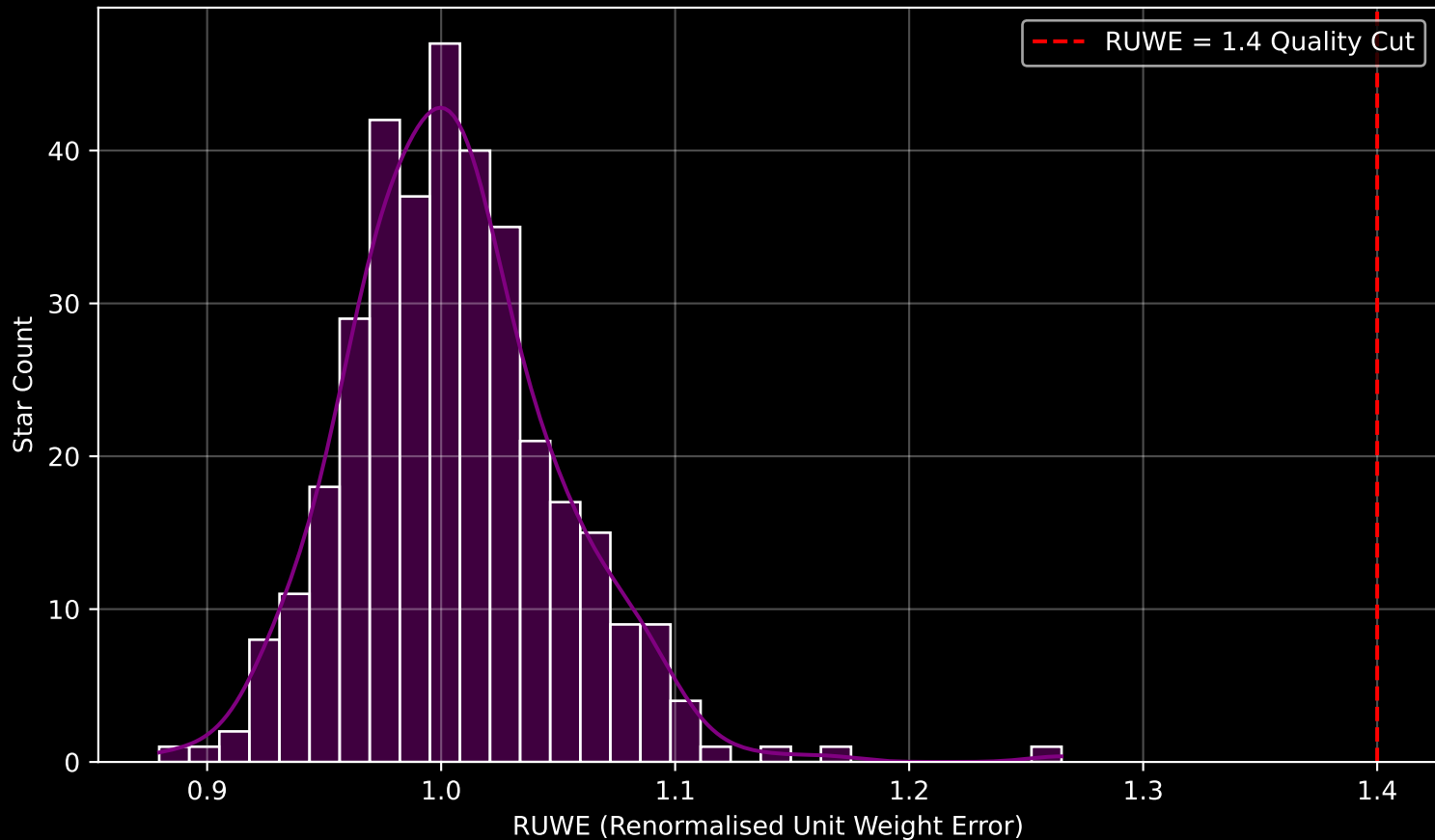
Gaia Stream: [Phlegethon] RUWE Distribution (n= 350)
