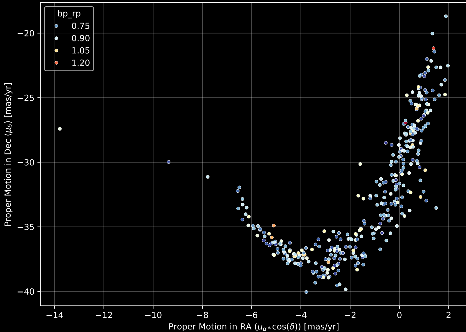
Gaia Stream: [Phlegethon] Proper Motion Diagram (n= 350)
