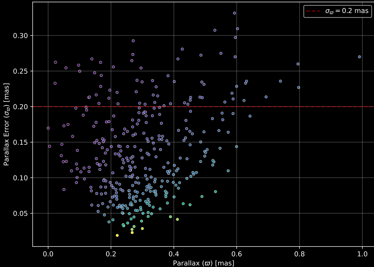
Gaia Stream: [Phlegethon] Parallax Quality (n= 350)
