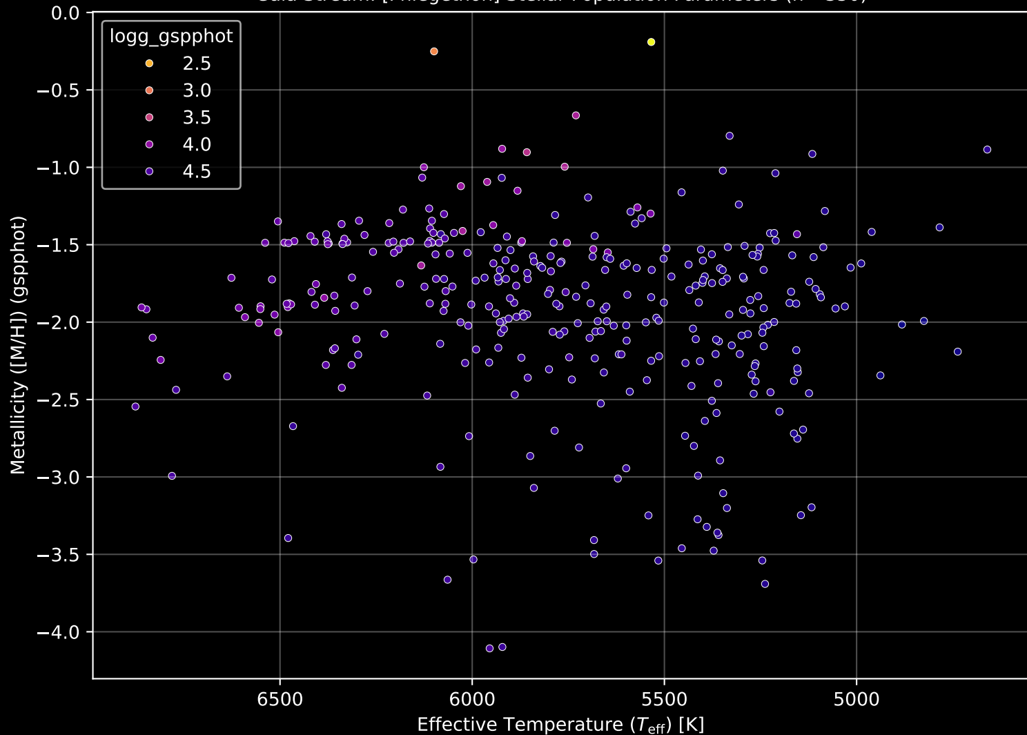
Gaia Stream: [Phlegethon] Stellar Population Parameters (n= 350)
