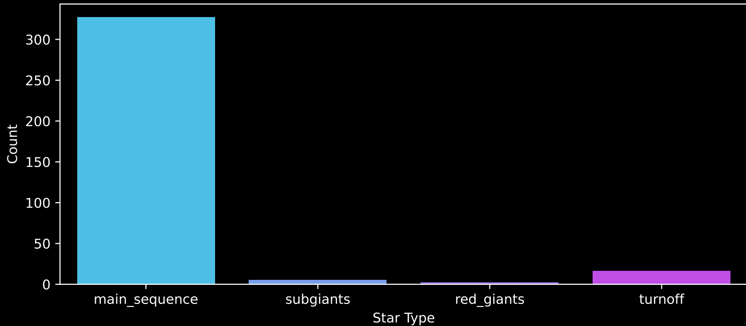
Gaia Stream: [Phlegethon] Count plot of Star Type
