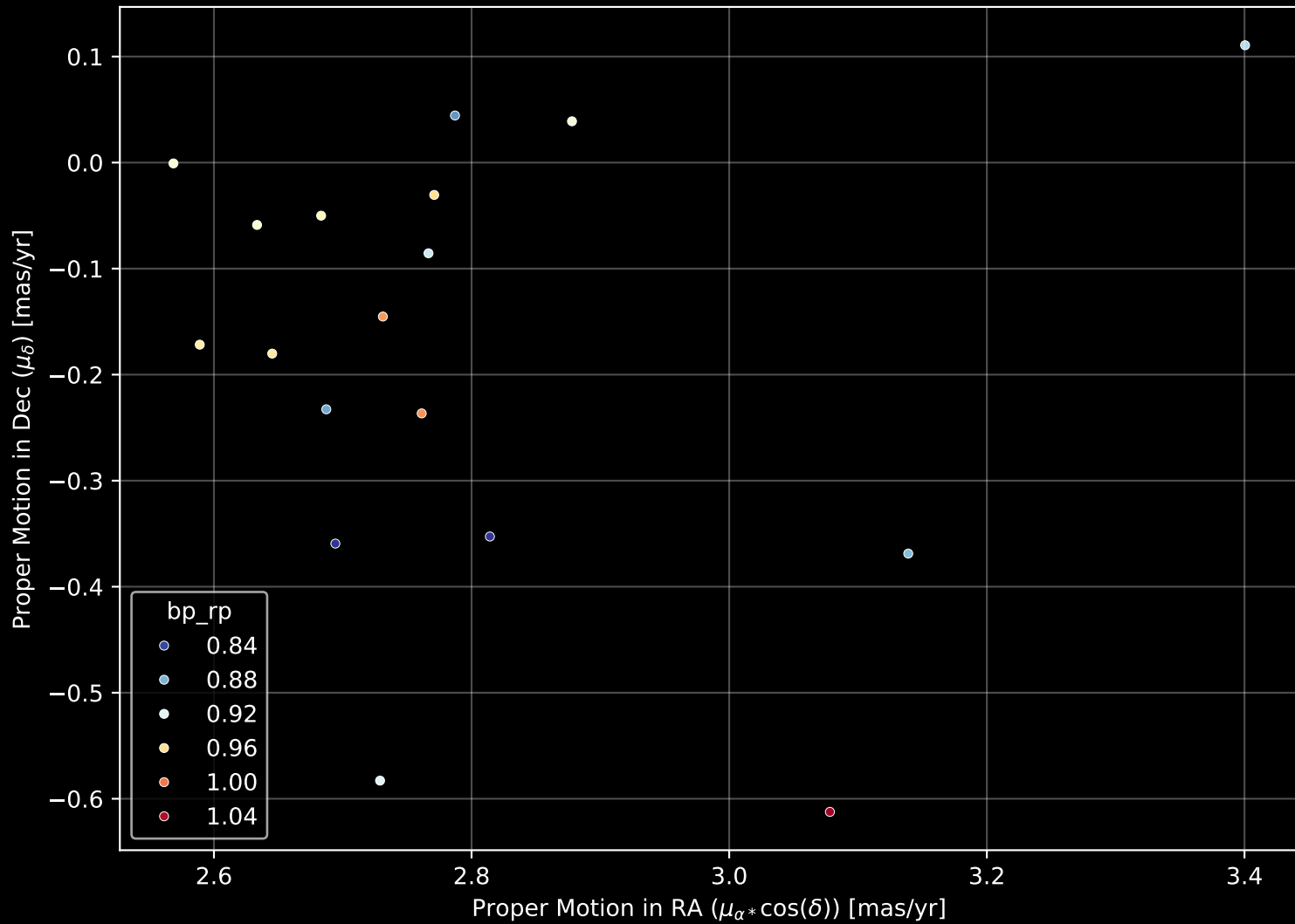
Gaia Stream: [Phoenix] Proper Motion Diagram (n= 18)
