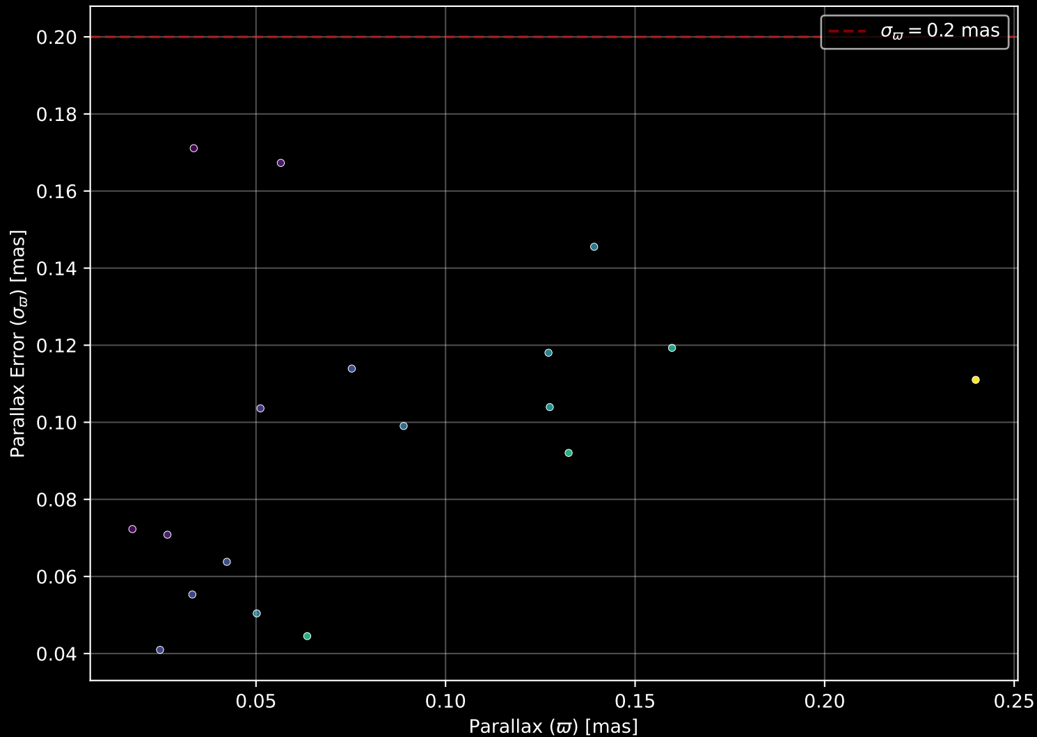
Gaia Stream: [Phoenix] Parallax Quality (n= 18)
