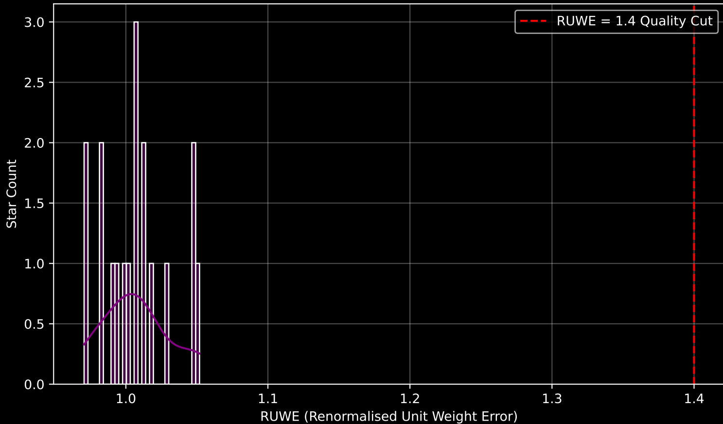
Gaia Stream: [Phoenix] RUWE Distribution (n= 18)
