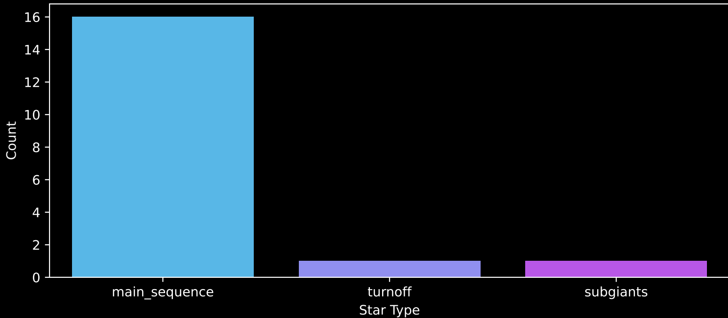
Gaia Stream: [Phoenix] Count plot of Star Type
