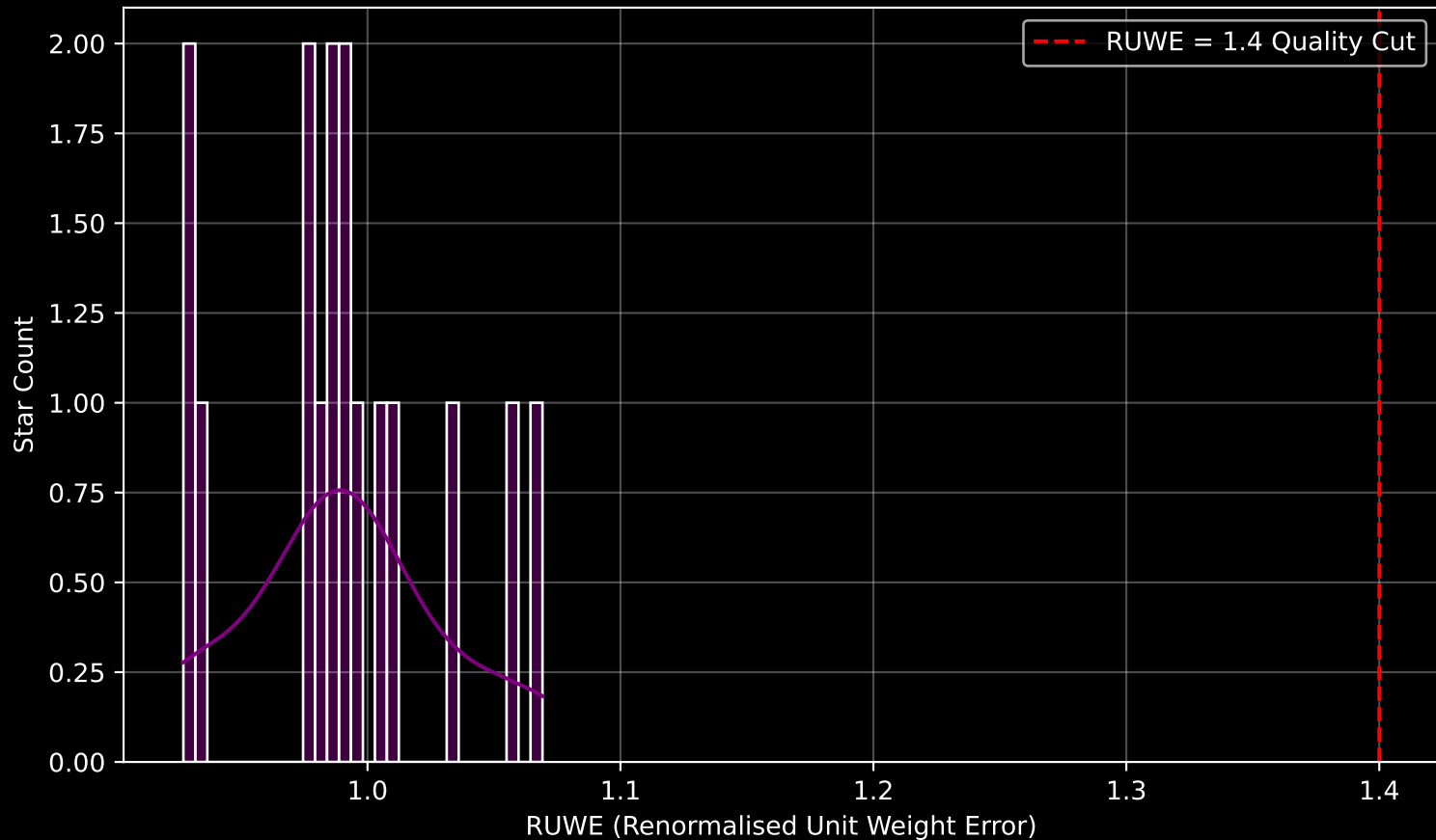
Gaia Stream: [SCP-S] RUWE Distribution (n= 16)
