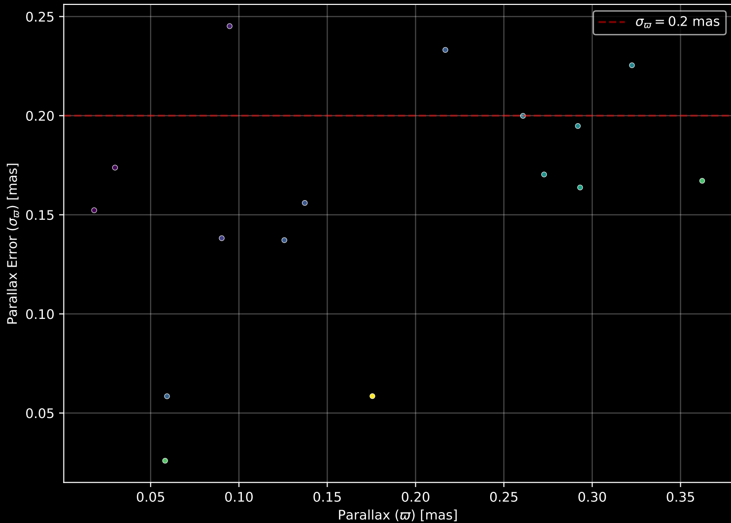
Gaia Stream: [SCP-S] Parallax Quality (n= 16)
