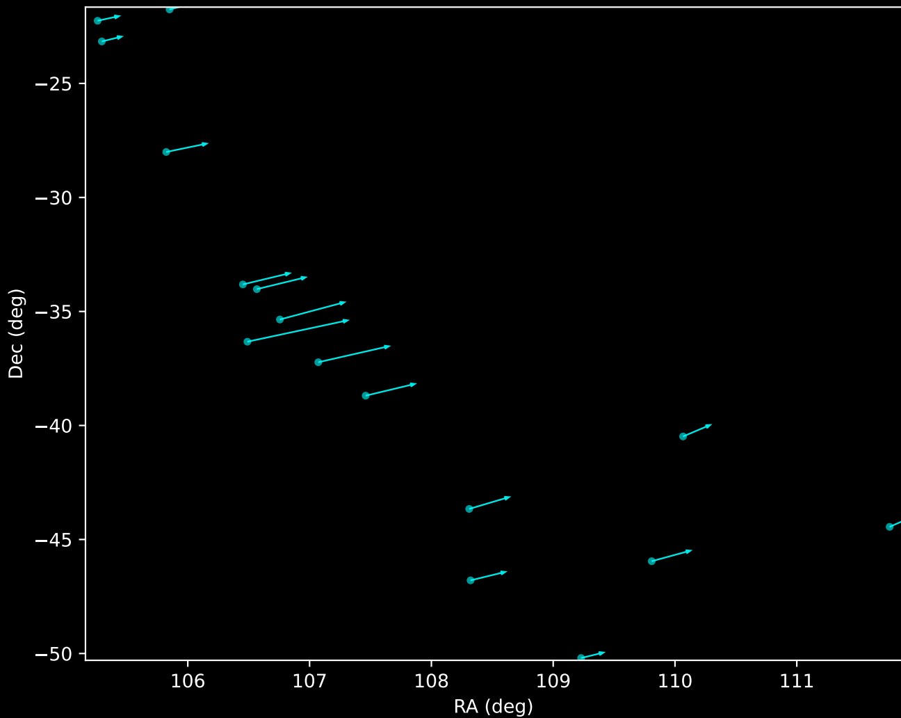
Gaia DR3 Noise Stream Proper Motion Vectors (n=16)
