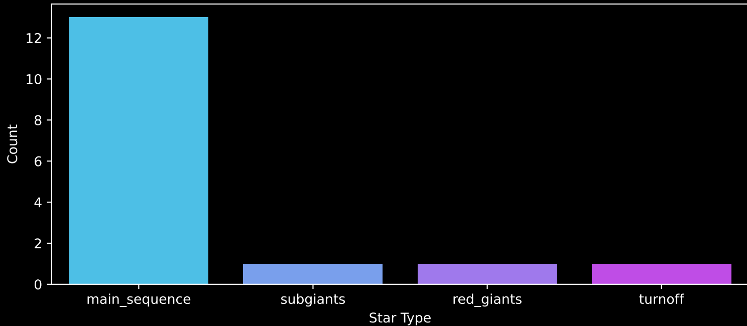
Gaia Stream: [SCP-S] Count plot of Star Type
