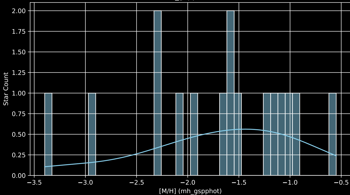
Gaia Stream: [SCP-S [M/H] (mh_gspphot) (n= 16)
