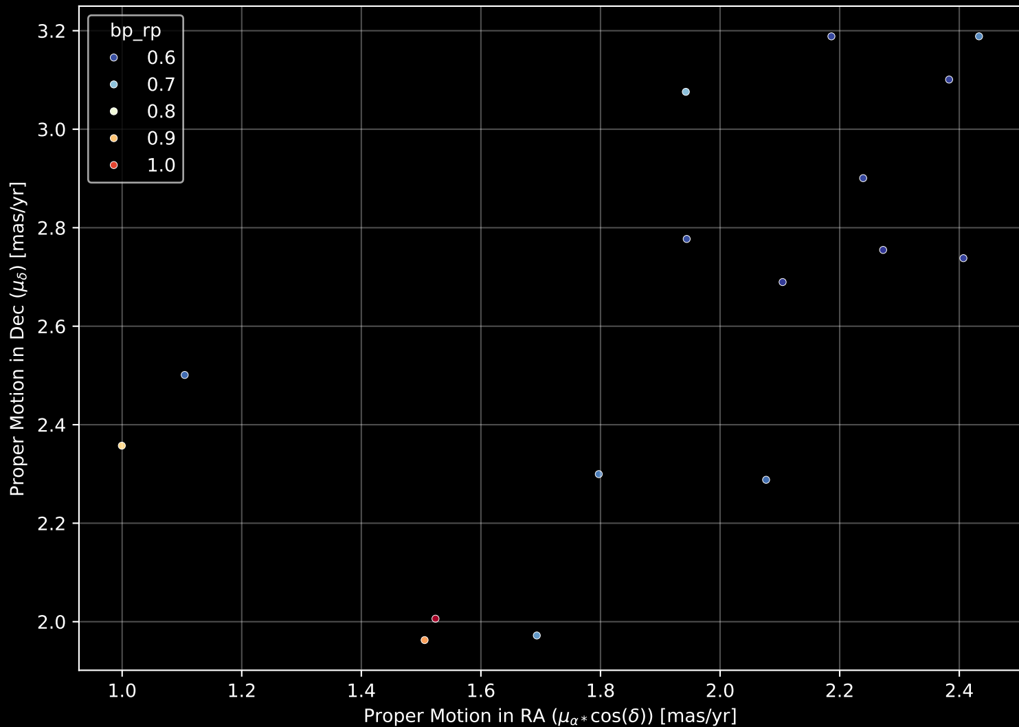
Gaia Stream: [SCP-S] Proper Motion Diagram (n= 16)
