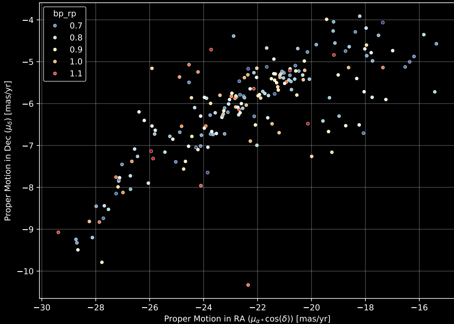
Gaia Stream: [Slidr] Proper Motion Diagram (n= 199)
