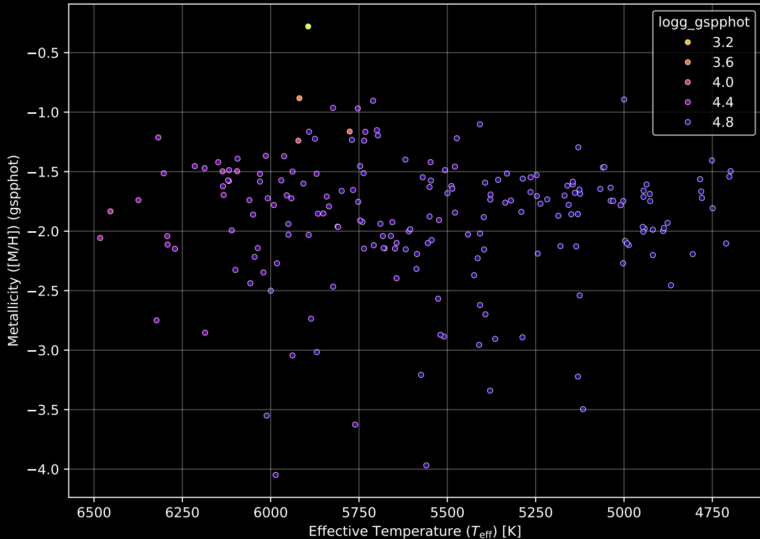
Gaia Stream: [Slidr] Stellar Population Parameters (n= 199)
