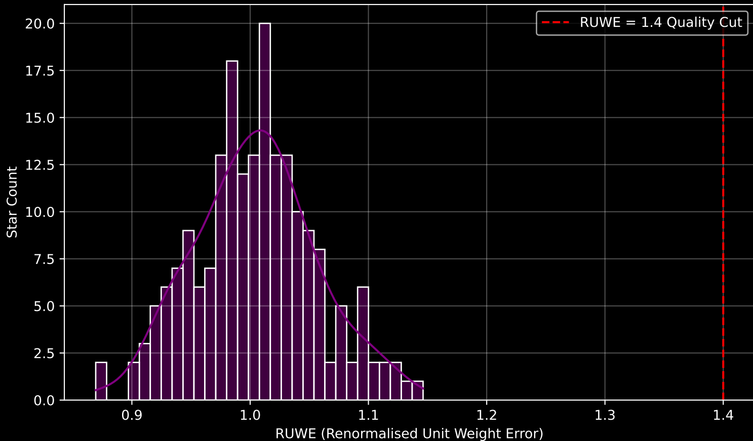
Gaia Stream: [Slidr] RUWE Distribution (n= 199)
