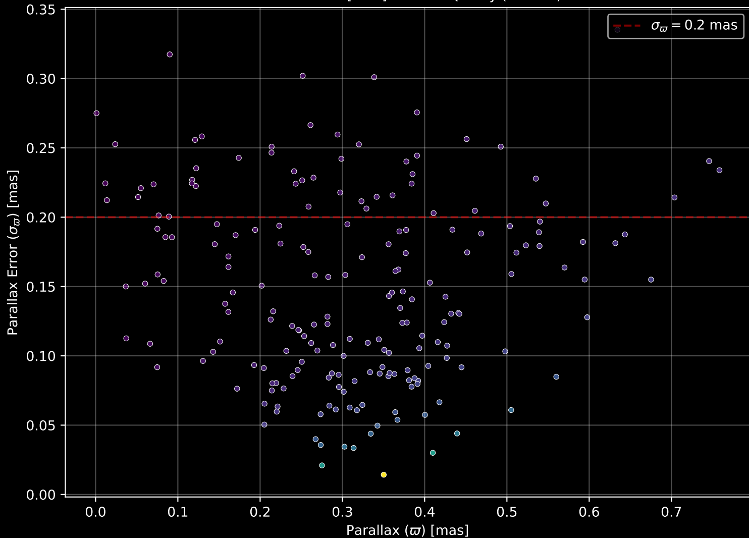
Gaia Stream: [Slidr] Parallax Quality (n = 199)
