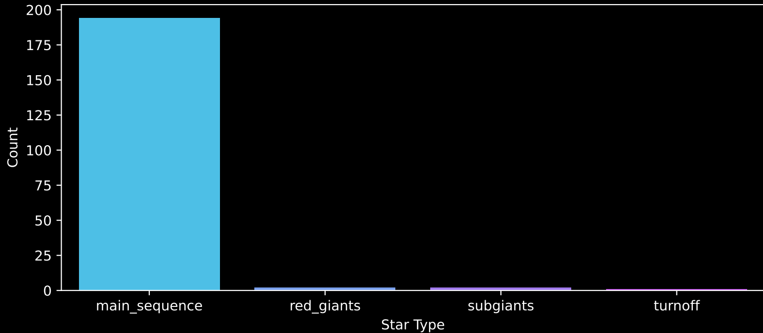
Gaia Stream: [Slidr] Count plot of Star Type
