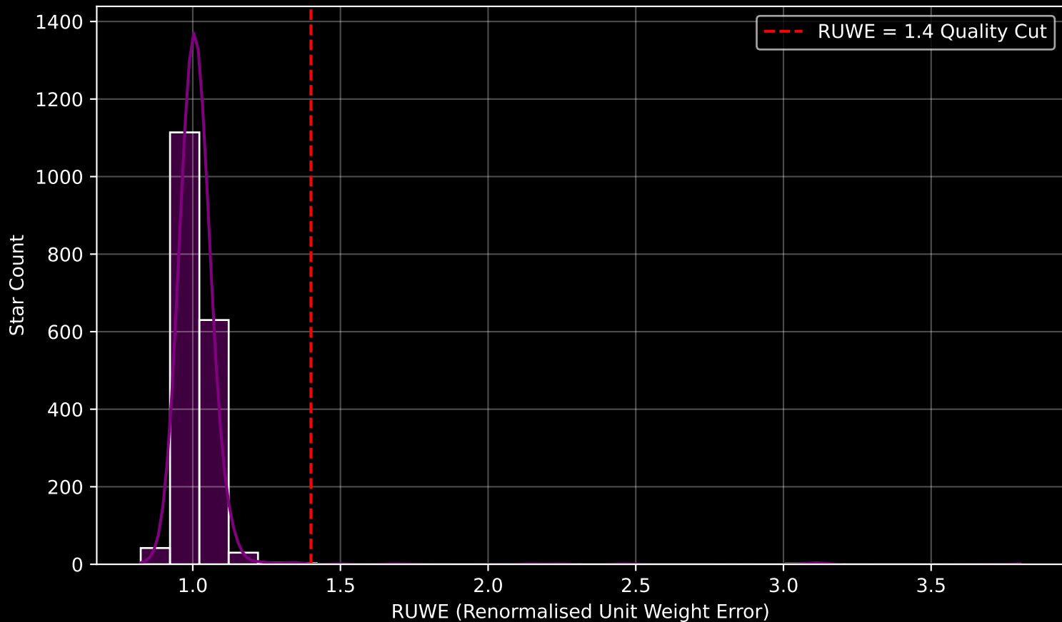
Gaia Stream: [Svol] RUWE Distribution (n= 1832)
