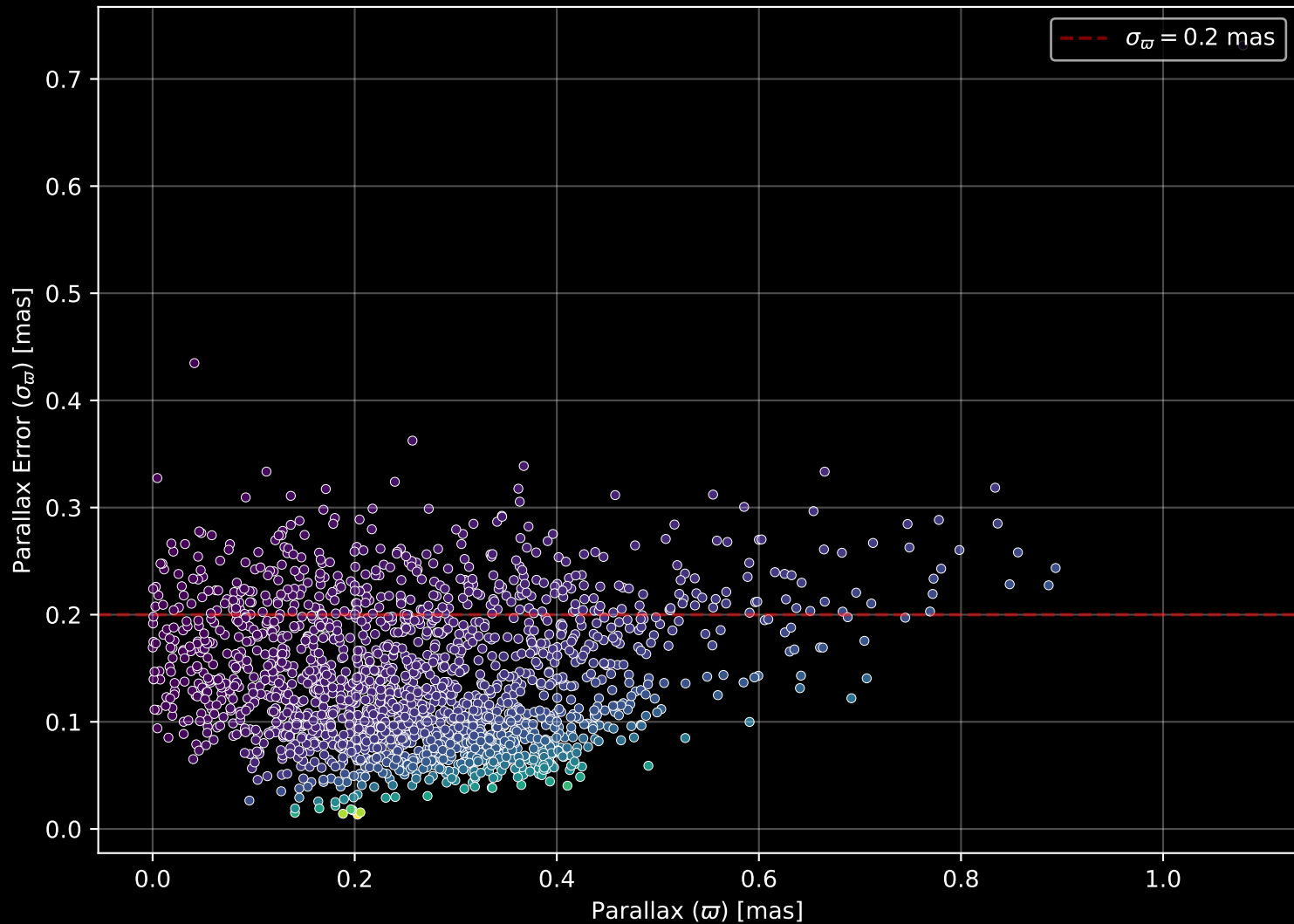
Gaia Stream: [Svol] Parallax Quality (n= 1838)
