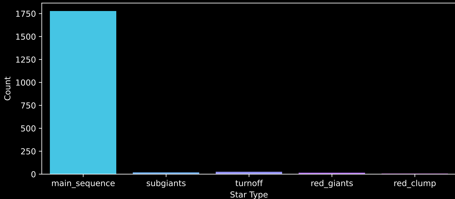
Gaia Stream: [Svol] Count plot of Star Type
