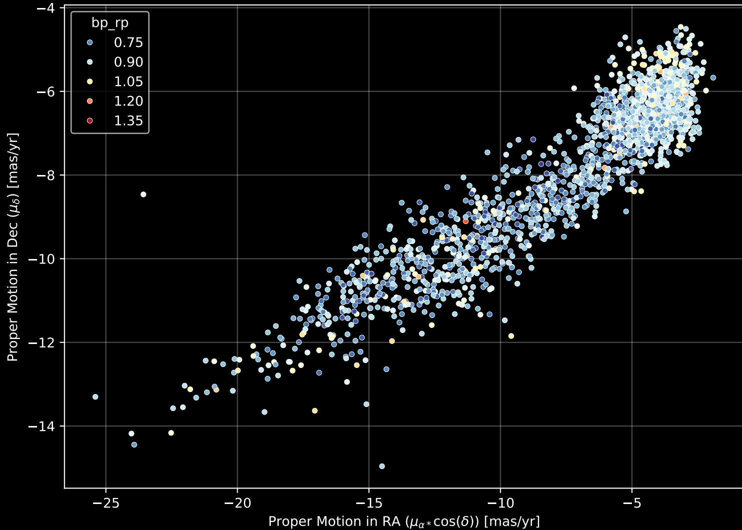
Gaia Stream: [Svol] Proper Motion Diagram (n= 1838)
