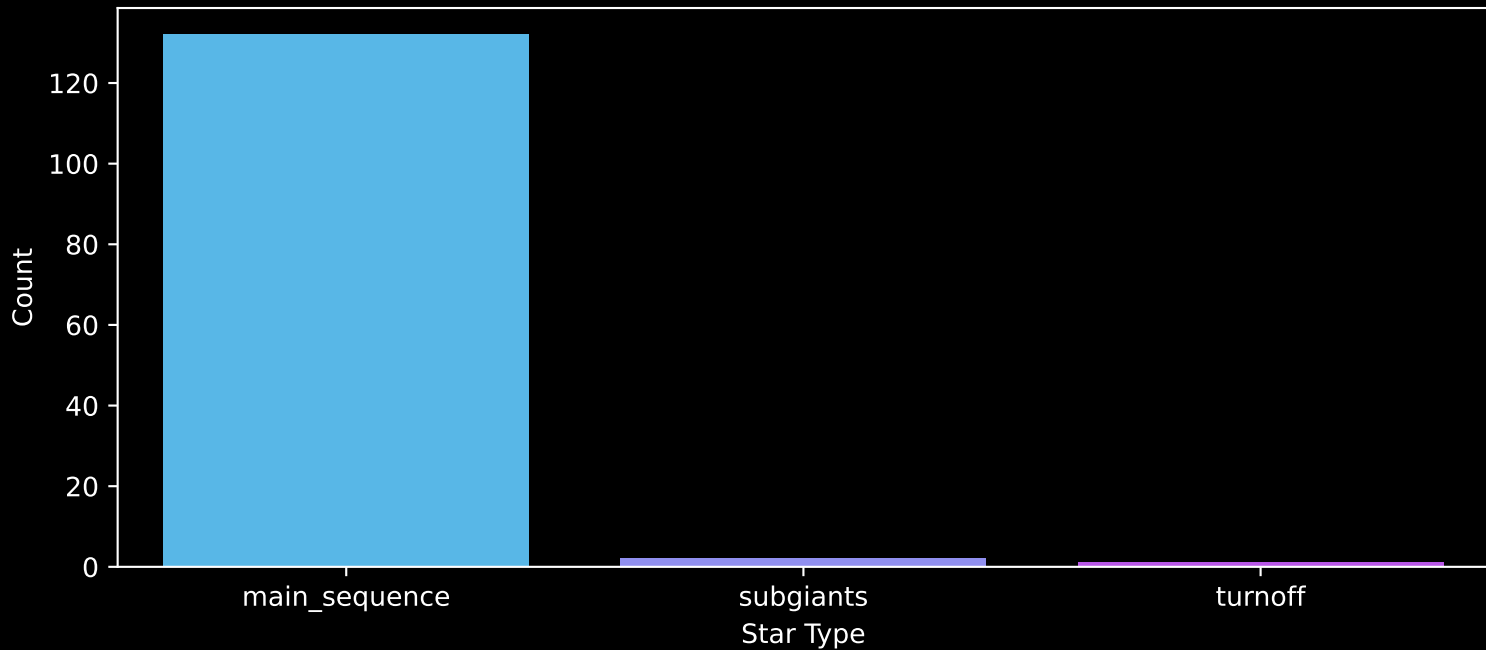
Gaia Stream: [Sylgr] Count plot of Star Type
