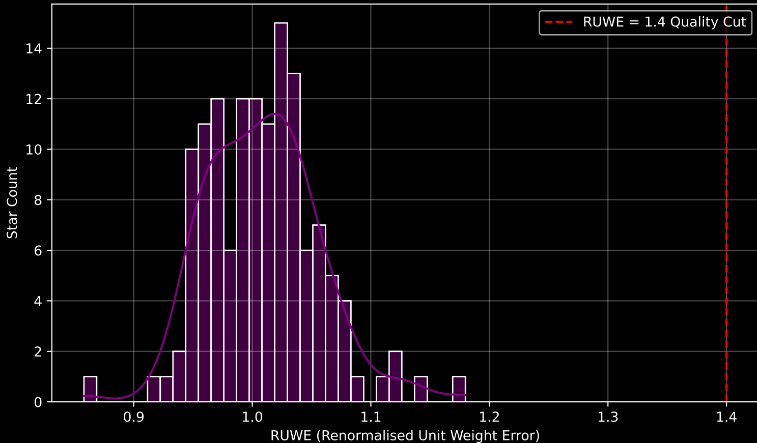
Gaia Stream: [Sylgr] RUWE Distribution (n= 135)
