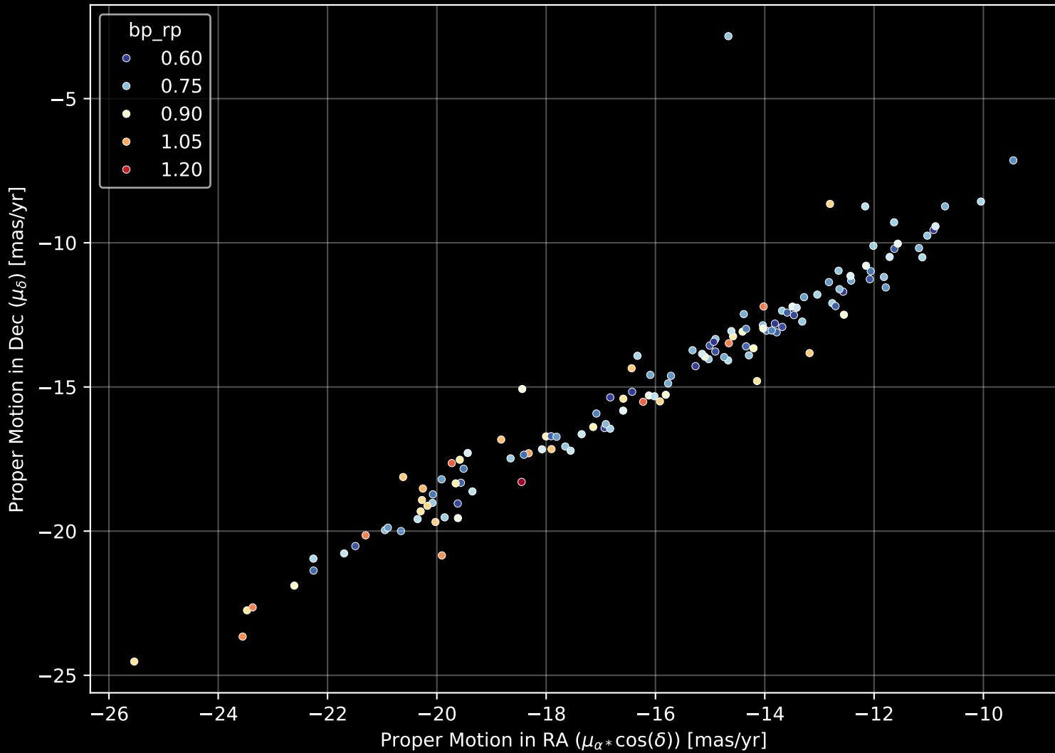
Gaia Stream: [Sylgr] Proper Motion Diagram (n= 135)
