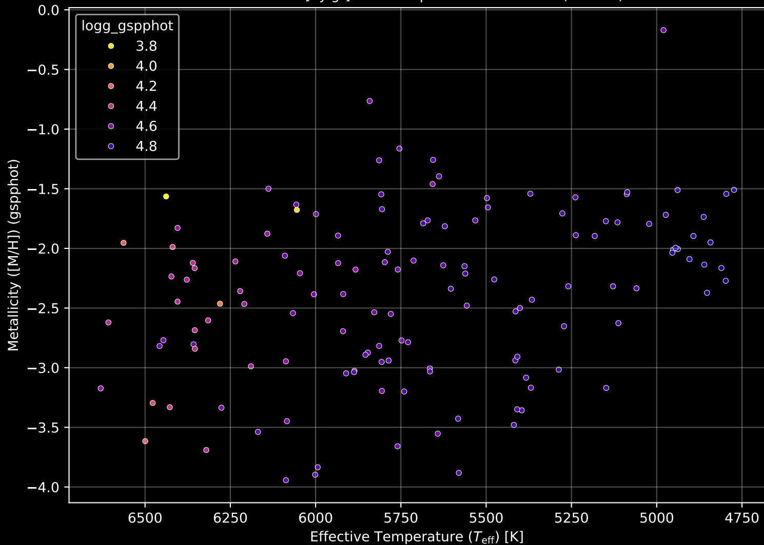
Gaia Stream: [Sylgr] Stellar Population Parameters (n= 135)
