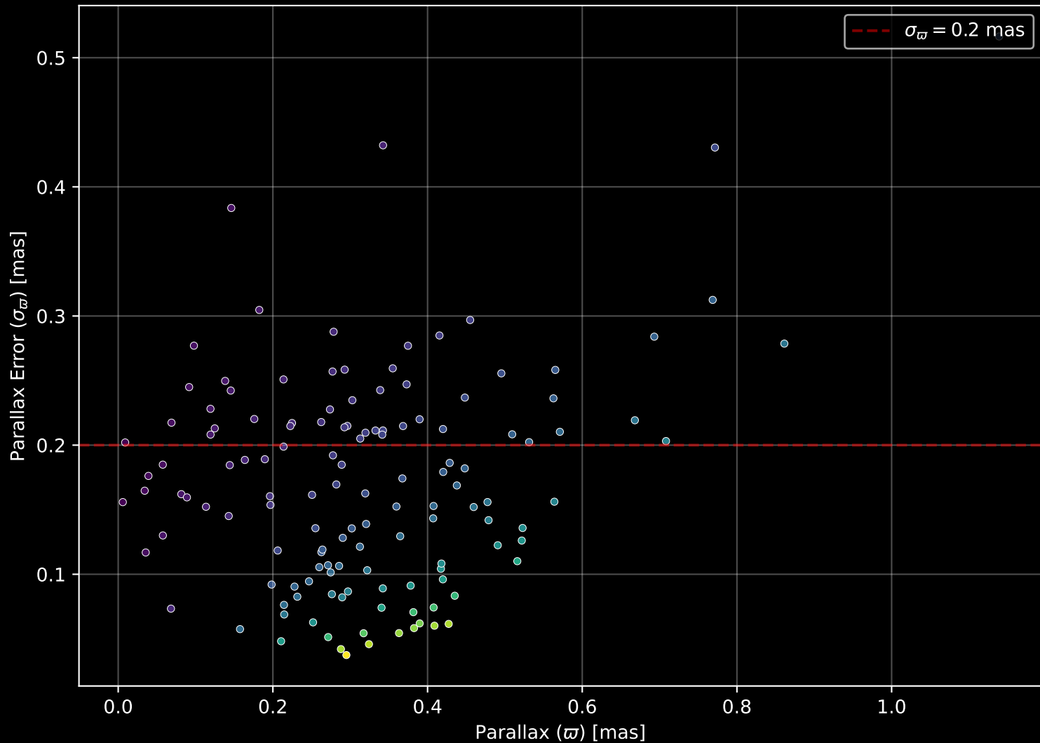
Gaia Stream: [Sylgr] Parallax Quality (n= 135)
