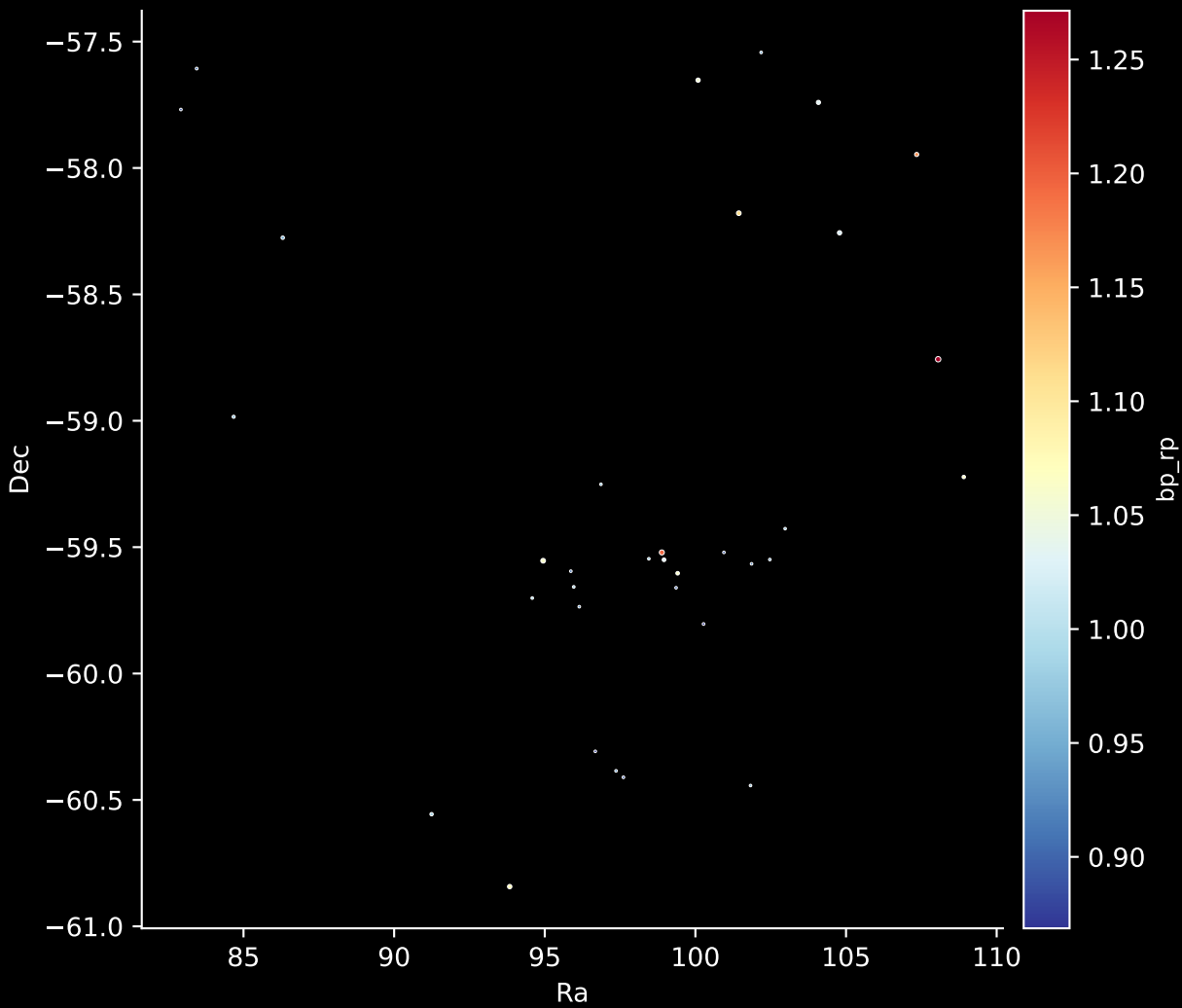
Gaia Stream: [Tuc-3] Stars: 34
