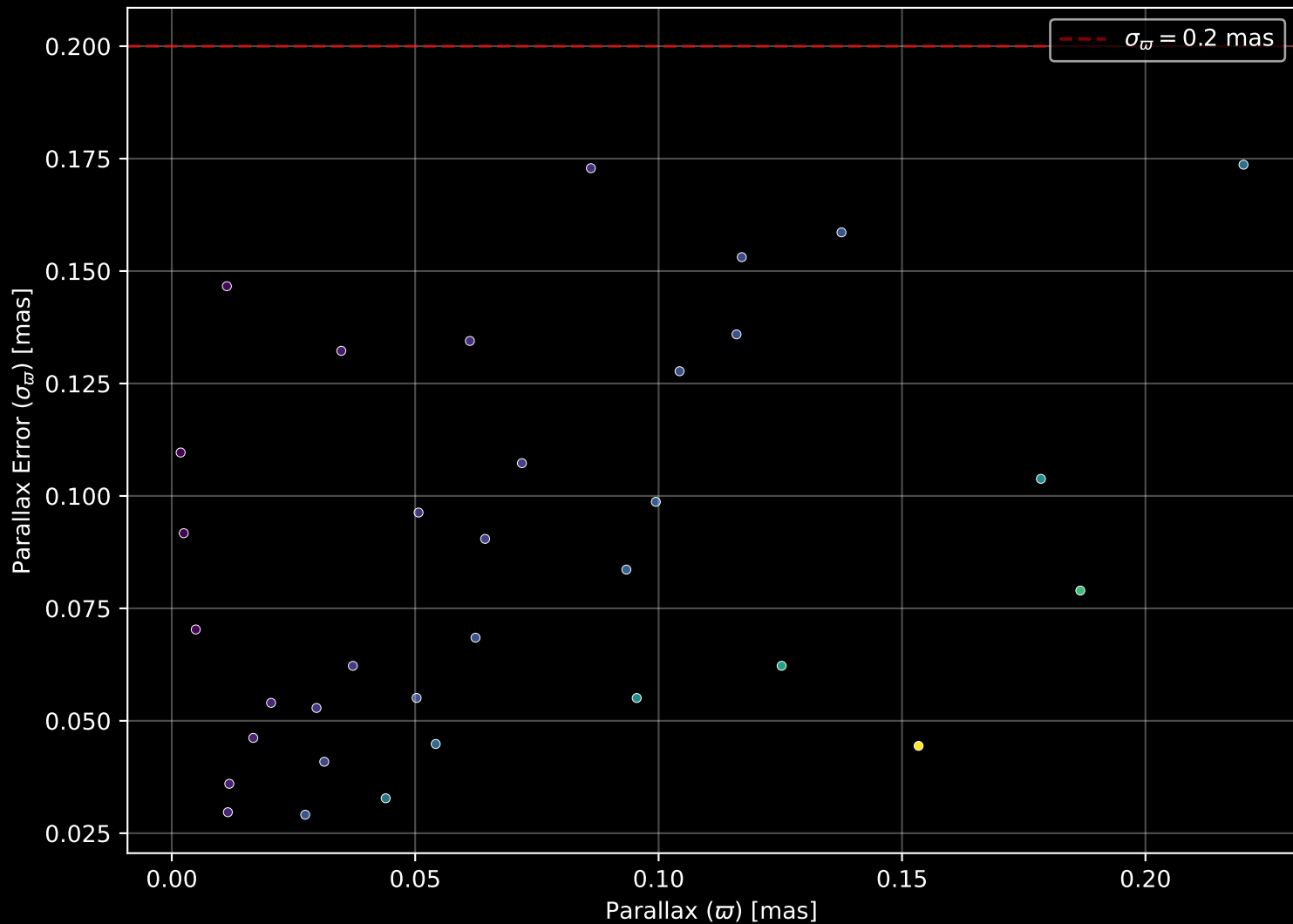
Gaia Stream: [Tuc-3] Parallax Quality (n= 34)
