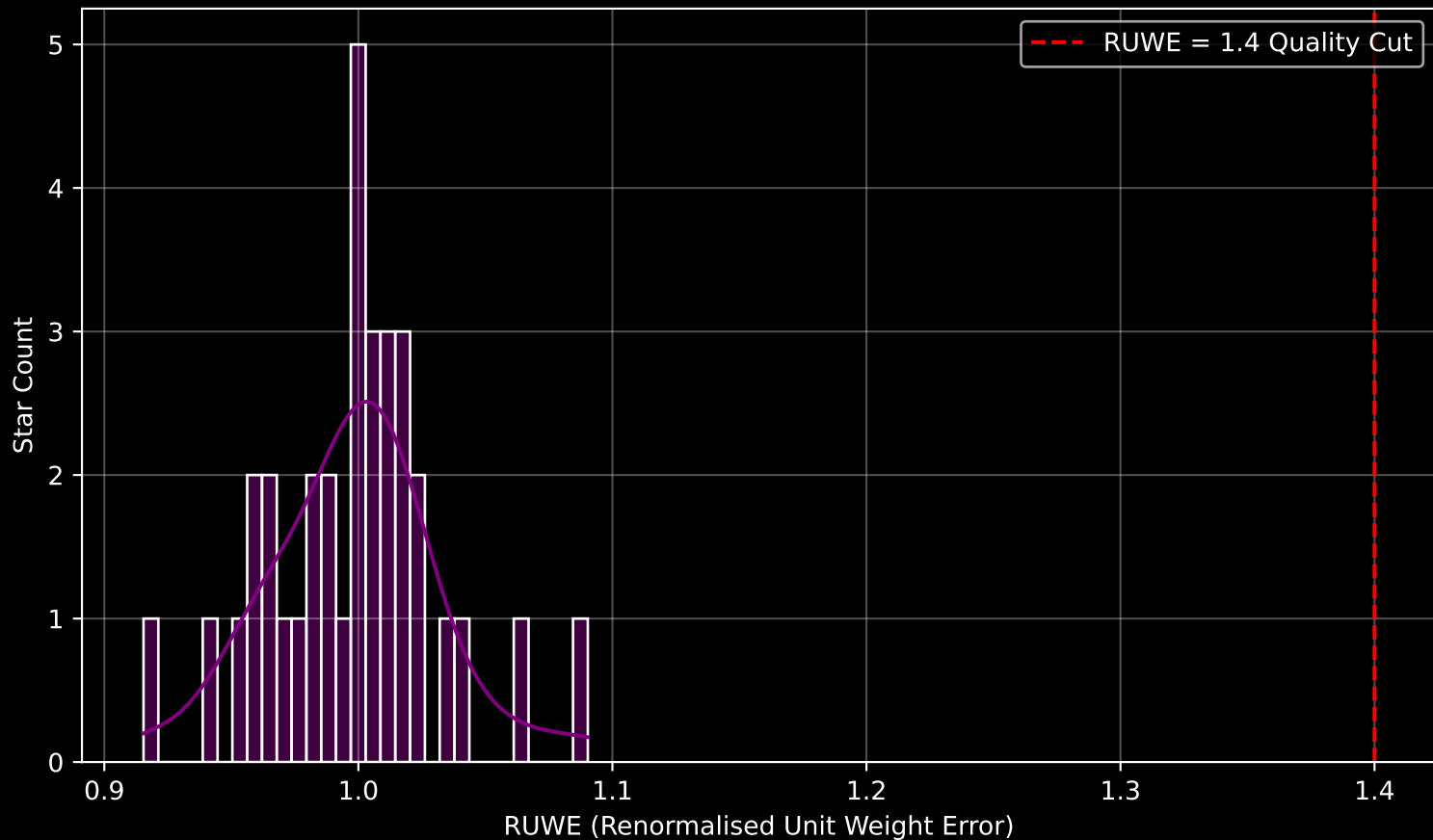
Gaia Stream: [Tuc-3] RUWE Distribution (n= 34)
