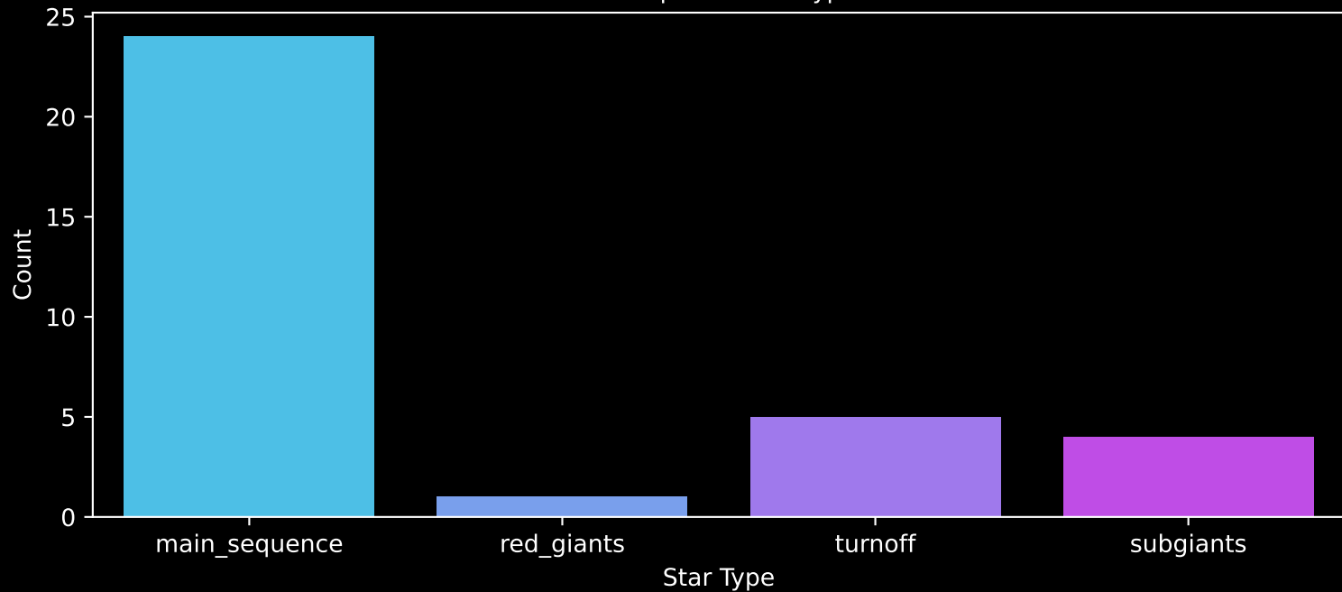
Gaia Stream: [Tuc-3] Count plot of Star Type
