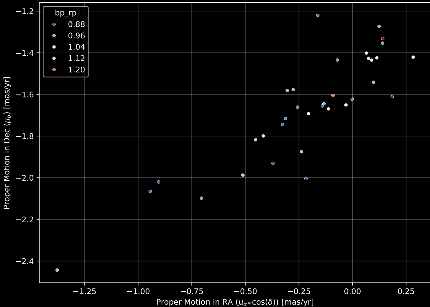
Gaia Stream: [Tuc-3] Proper Motion Diagram (n= 34)
