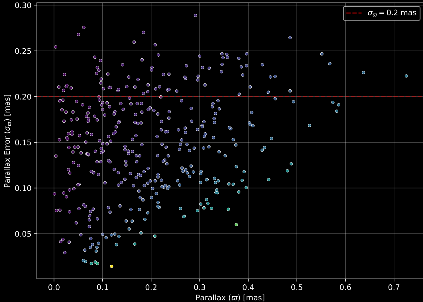
Gaia Stream: [Ylgr] Parallax Quality (n= 371)
