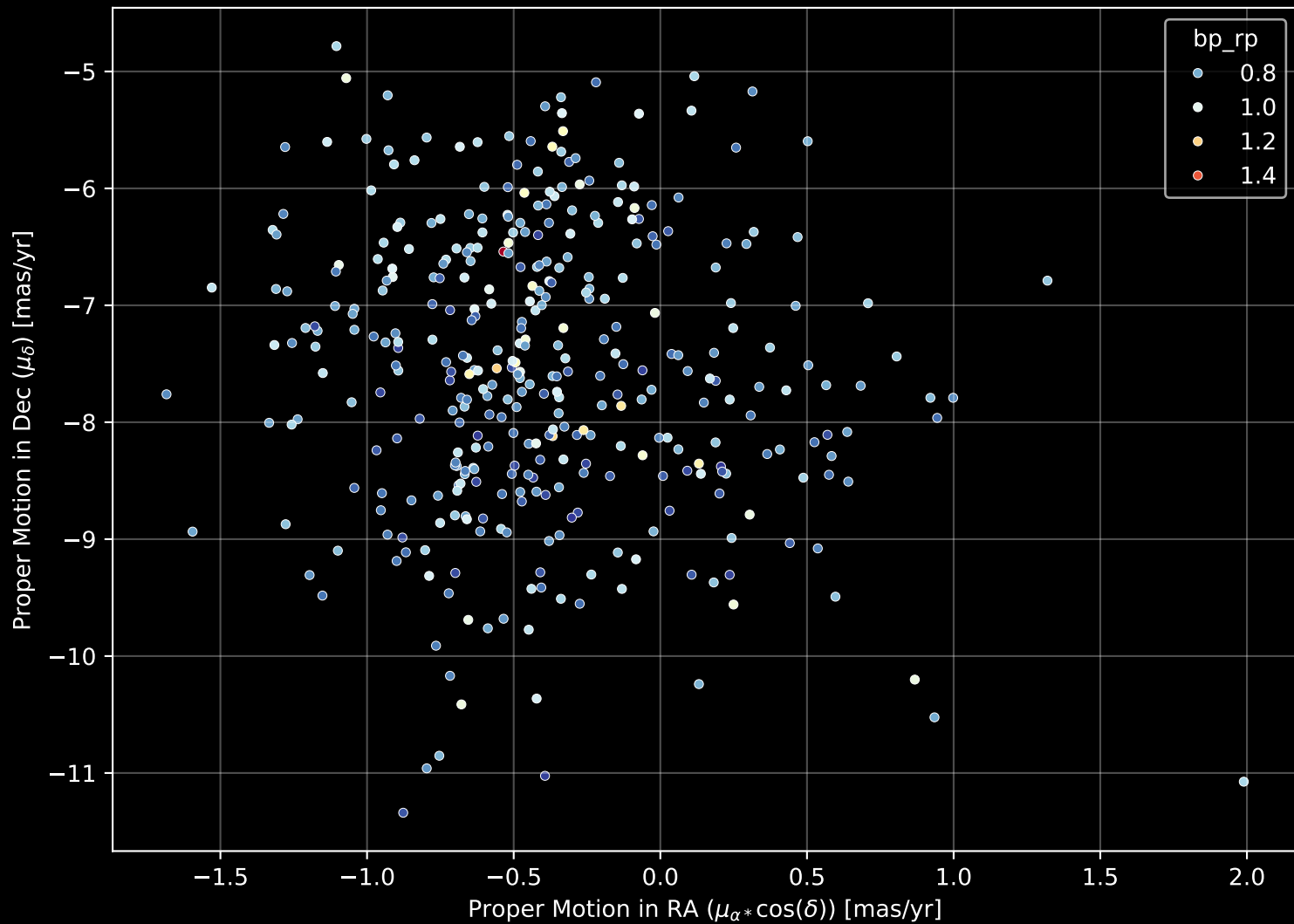
Gaia Stream: [Ylgr] Proper Motion Diagram (n= 371)
