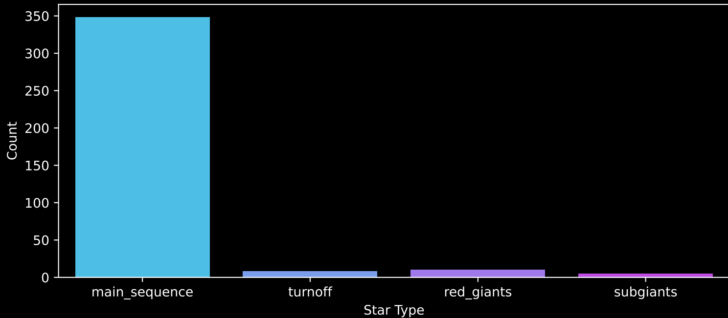
Gaia Stream: [Ylgr] Count plot of Star Type
