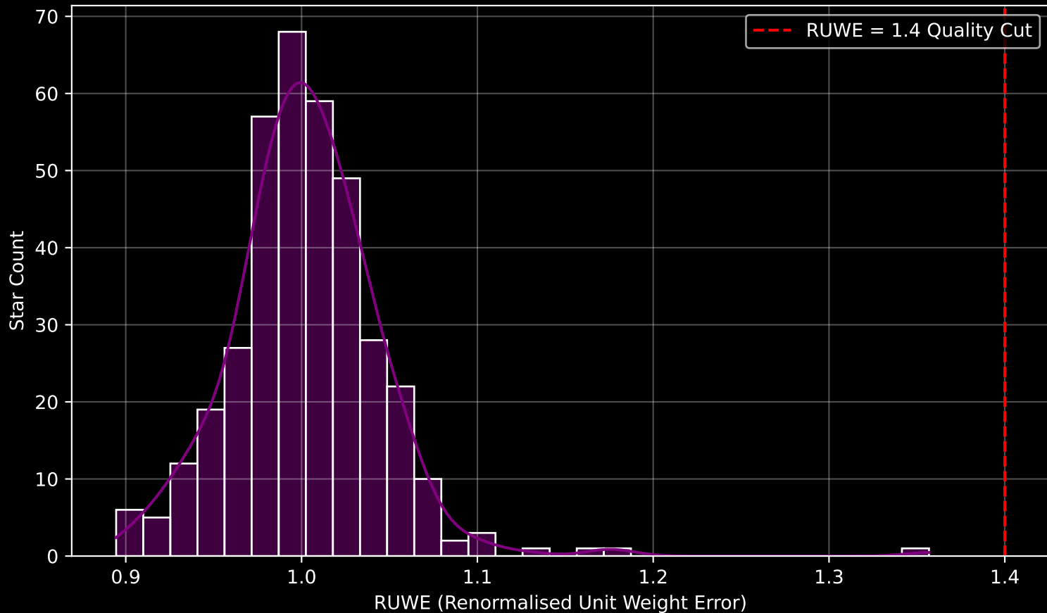
Gaia Stream: [Ylgr] RUWE Distribution (n= 371)
