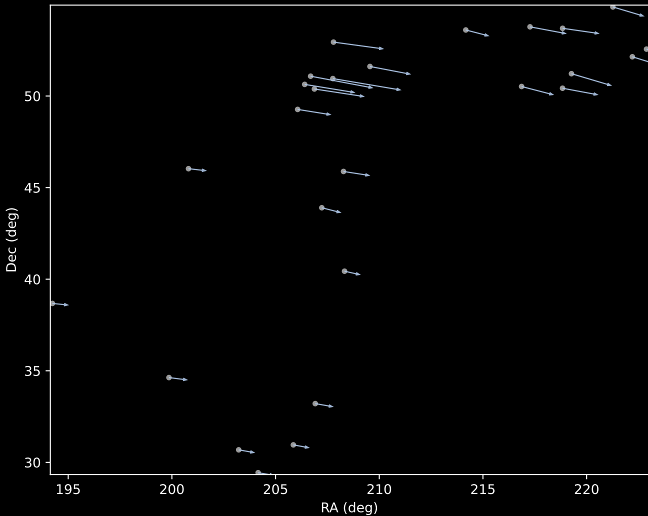
Gaia DR3 Cluster 1 Proper Motion Vectors (n=26)
