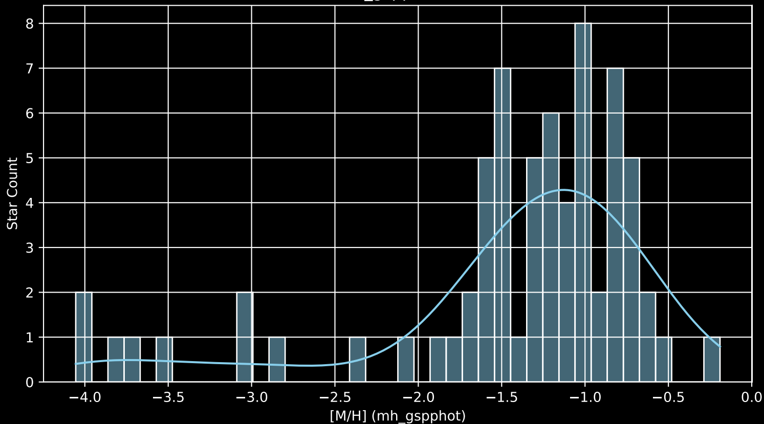
Gaia Stream: [C-13 [M/H] (mh_gspphot) (n= 68)
