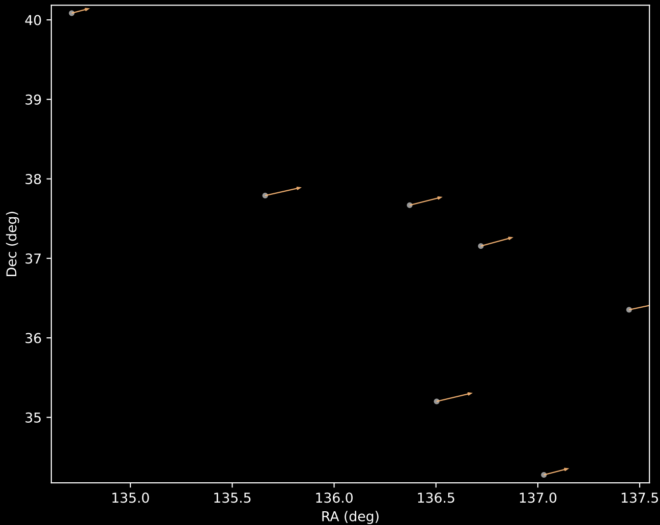
Gaia DR3 Cluster 3 Proper Motion Vectors (n=7)
