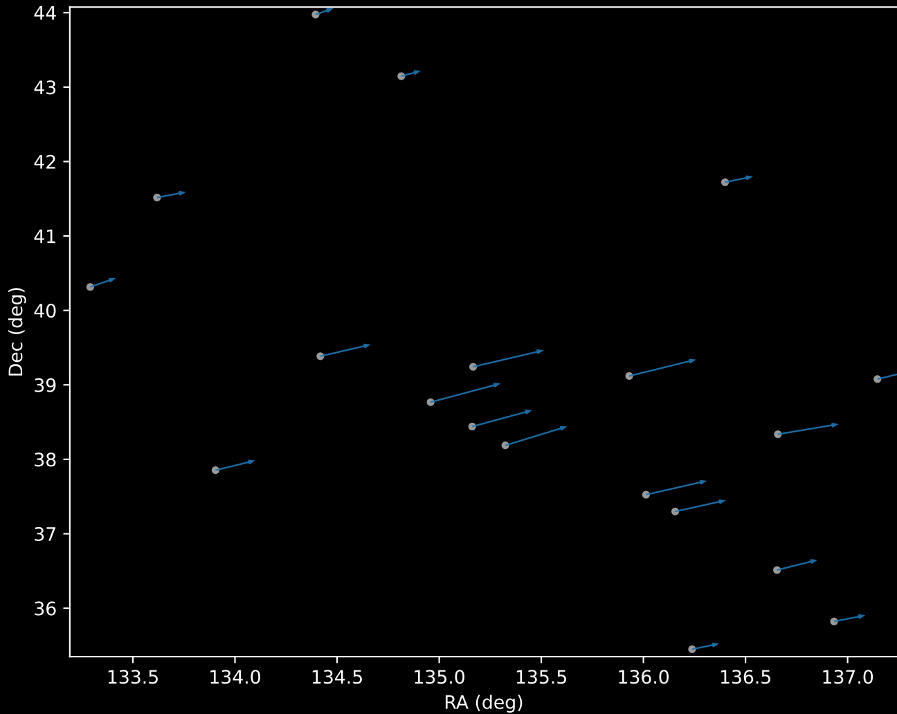
Gaia DR3 Cluster 0 Proper Motion Vectors (n=19)
