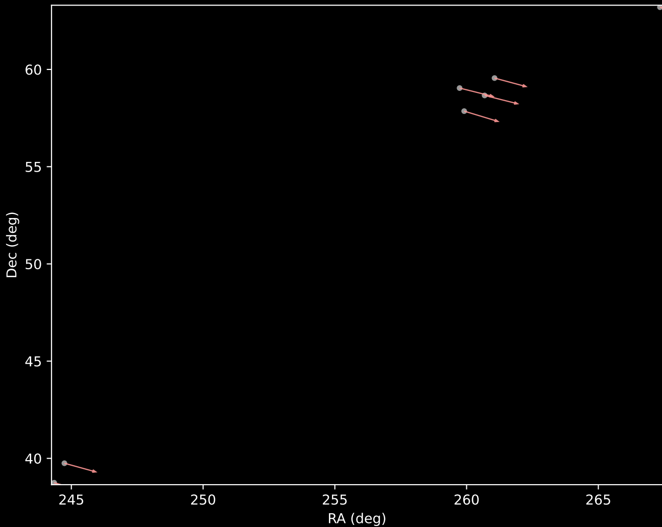
Gaia DR3 Cluster 7 Proper Motion Vectors (n=7)
