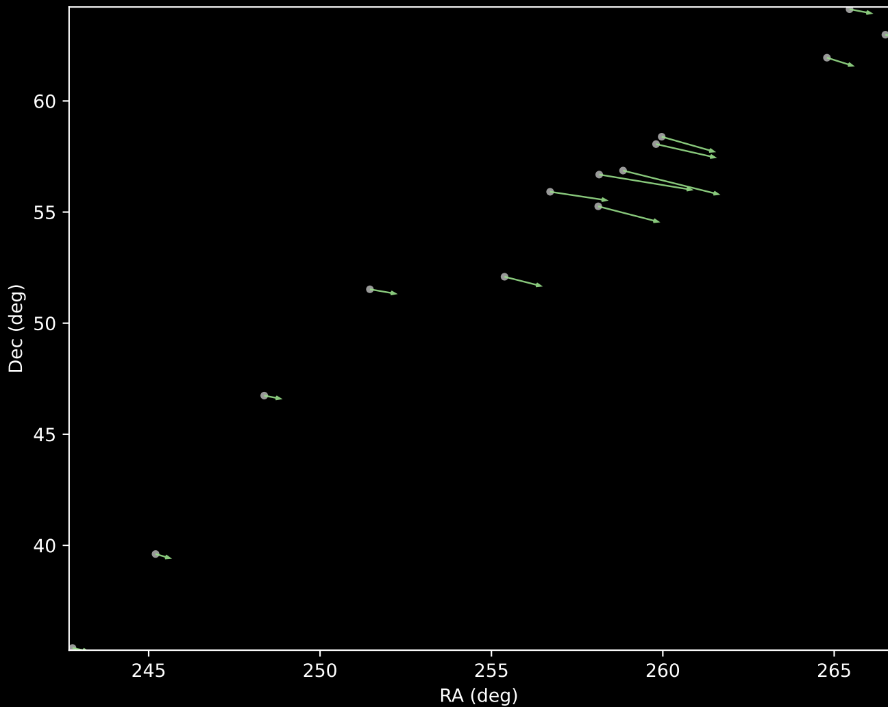
Gaia DR3 Cluster 5 Proper Motion Vectors (n=14)
