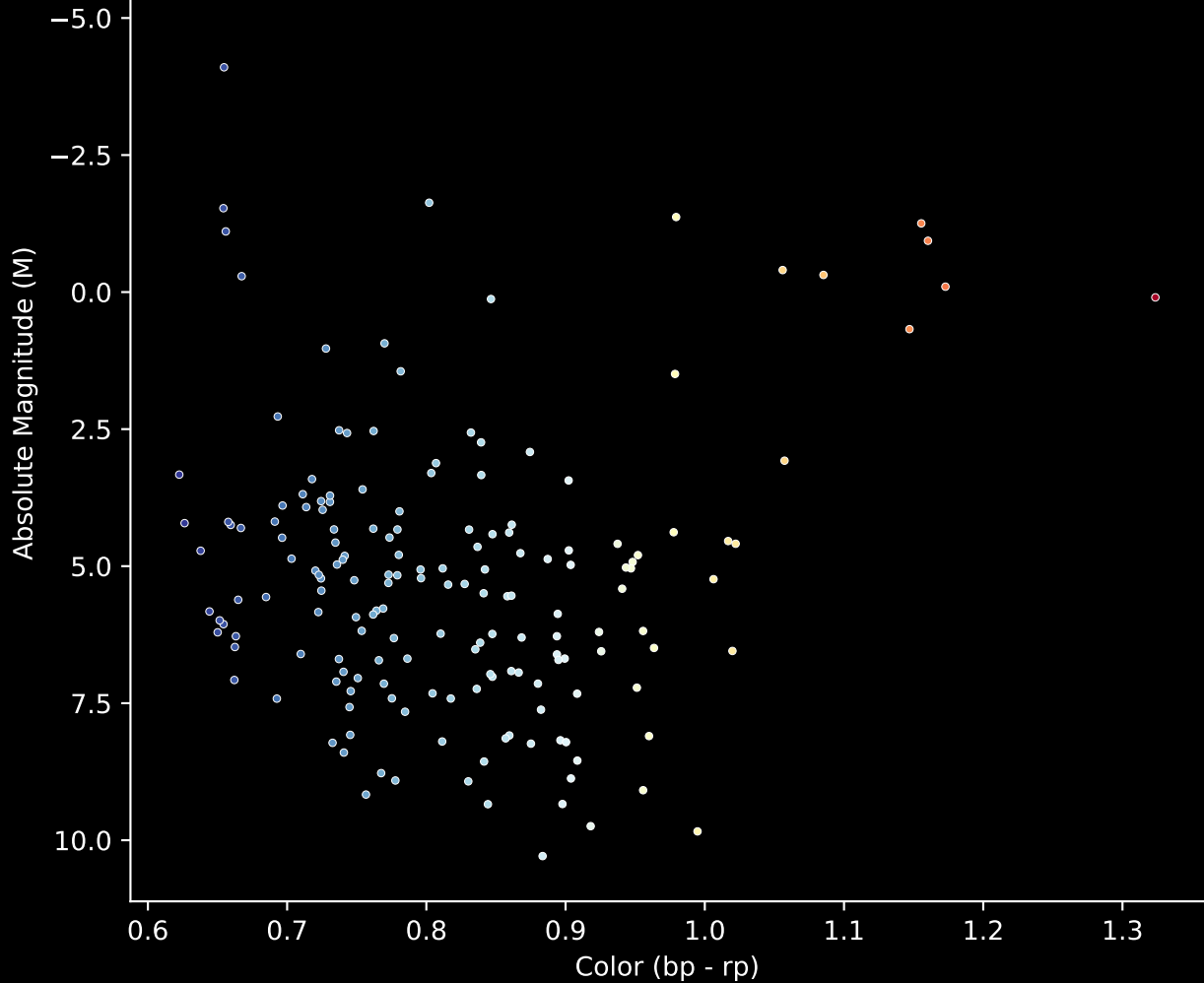
Gaia Stream: [C-7] Stream (n= 173) Hertzsprung-Russel Diagram
