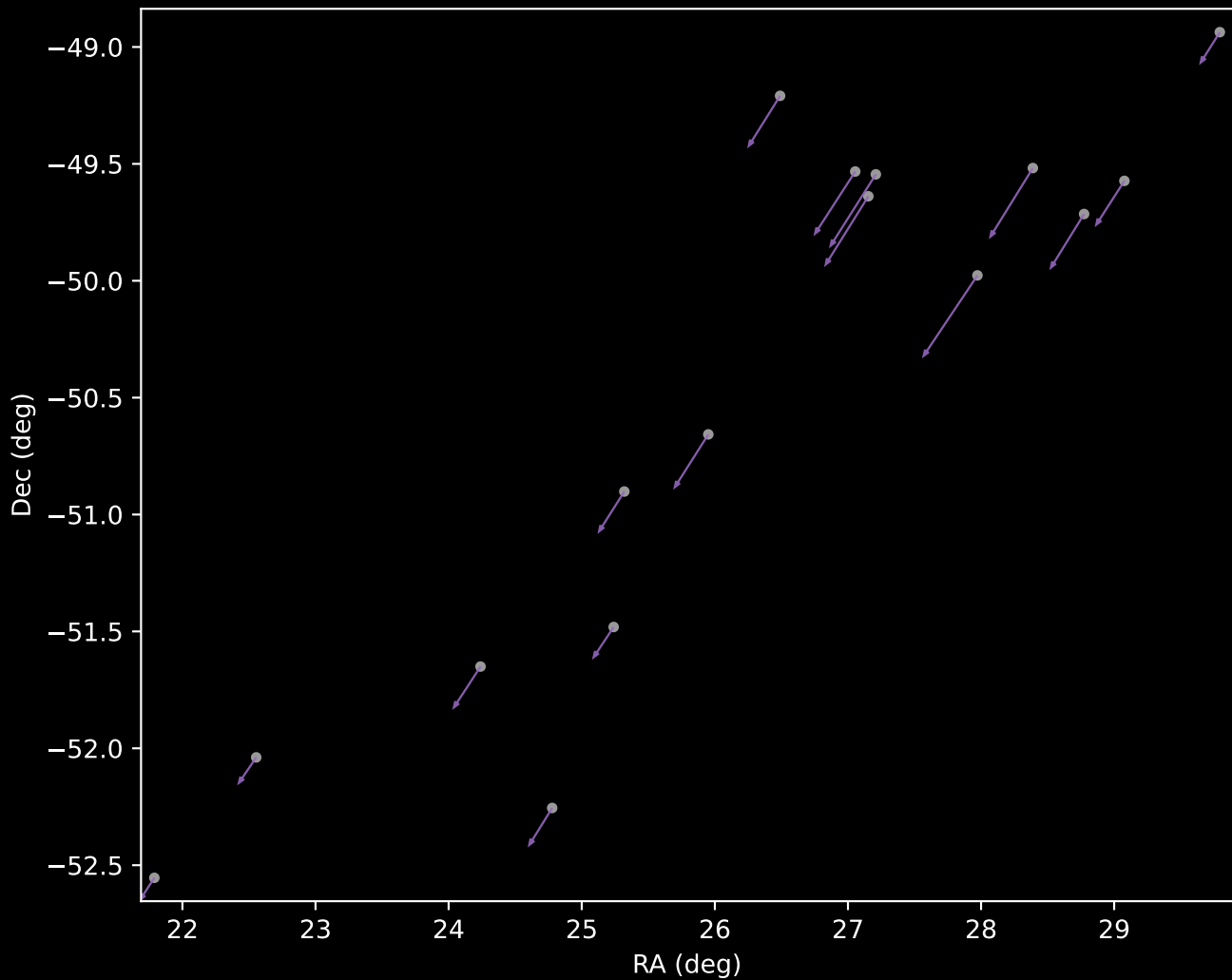
Gaia DR3 Cluster 8 Proper Motion Vectors (n=16)
