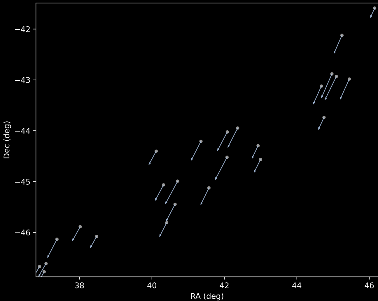
Gaia DR3 Cluster 1 Proper Motion Vectors (n=25)
