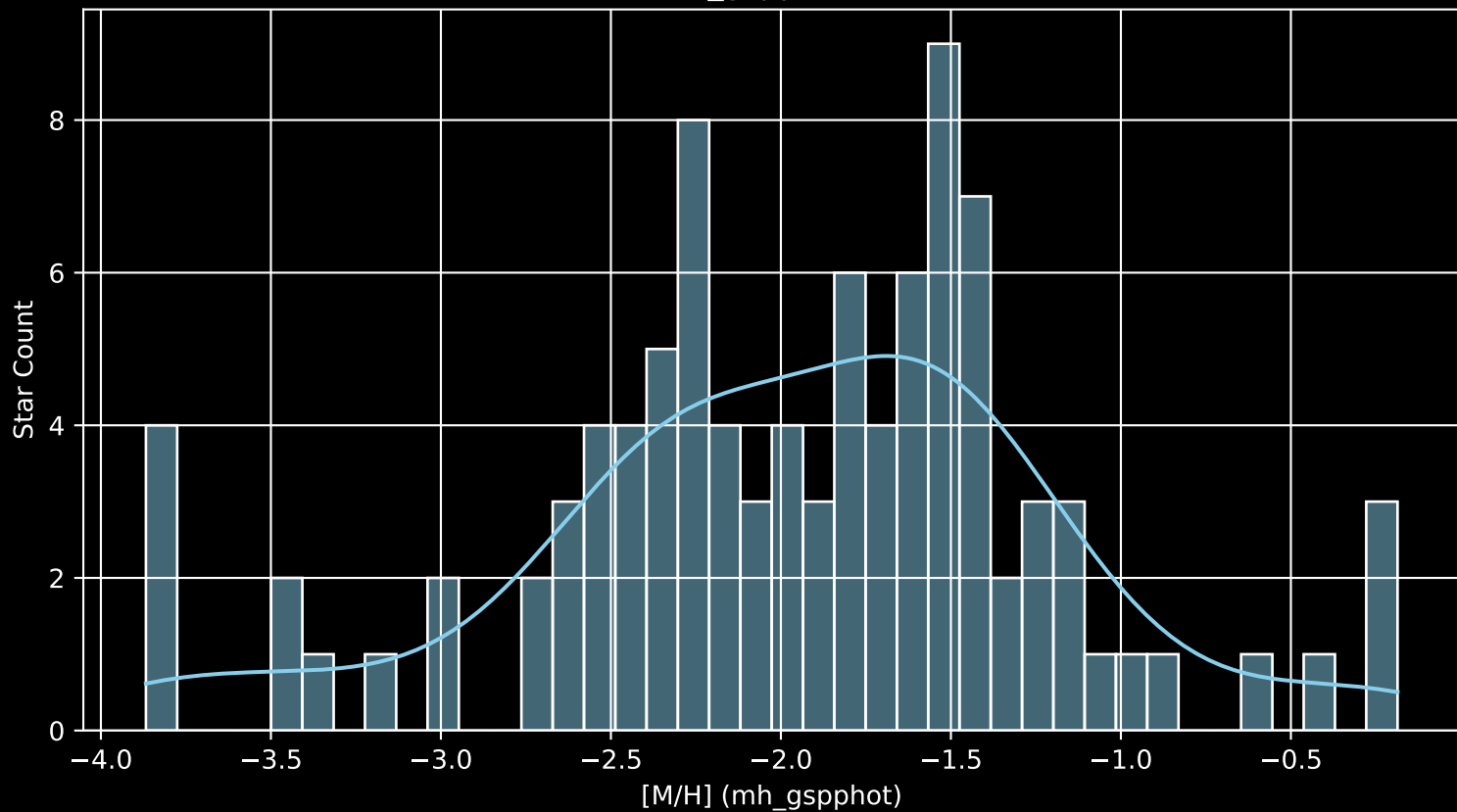
Gaia Stream: [C-7 [M/H] (mh_gspphot) (n= 98)
