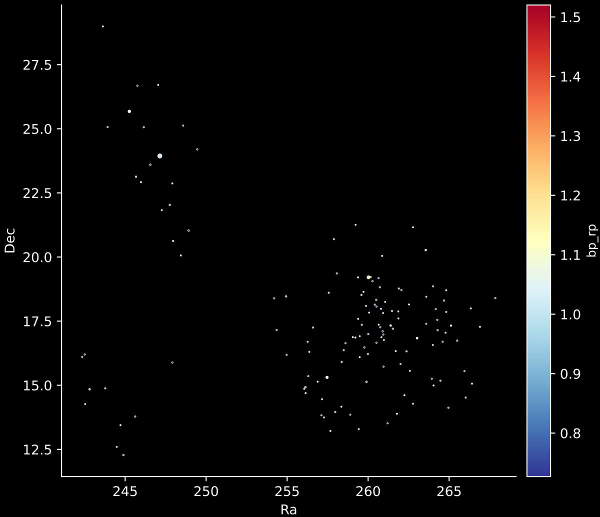
Gaia Stream: [C-9] Stars: 166
