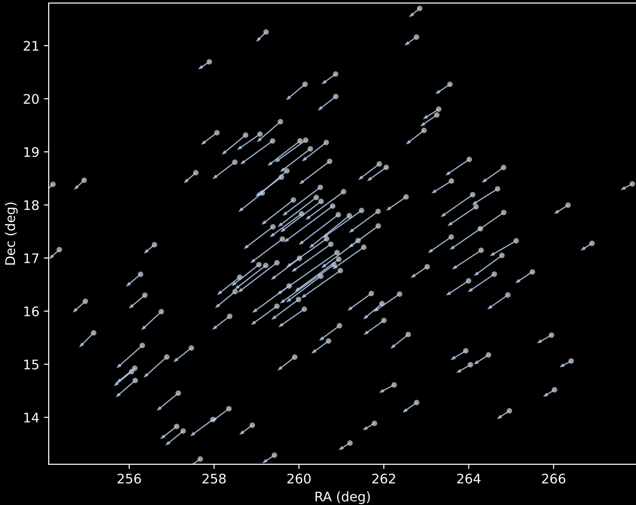
Gaia DR3 Cluster 1 Proper Motion Vectors (n=125)
