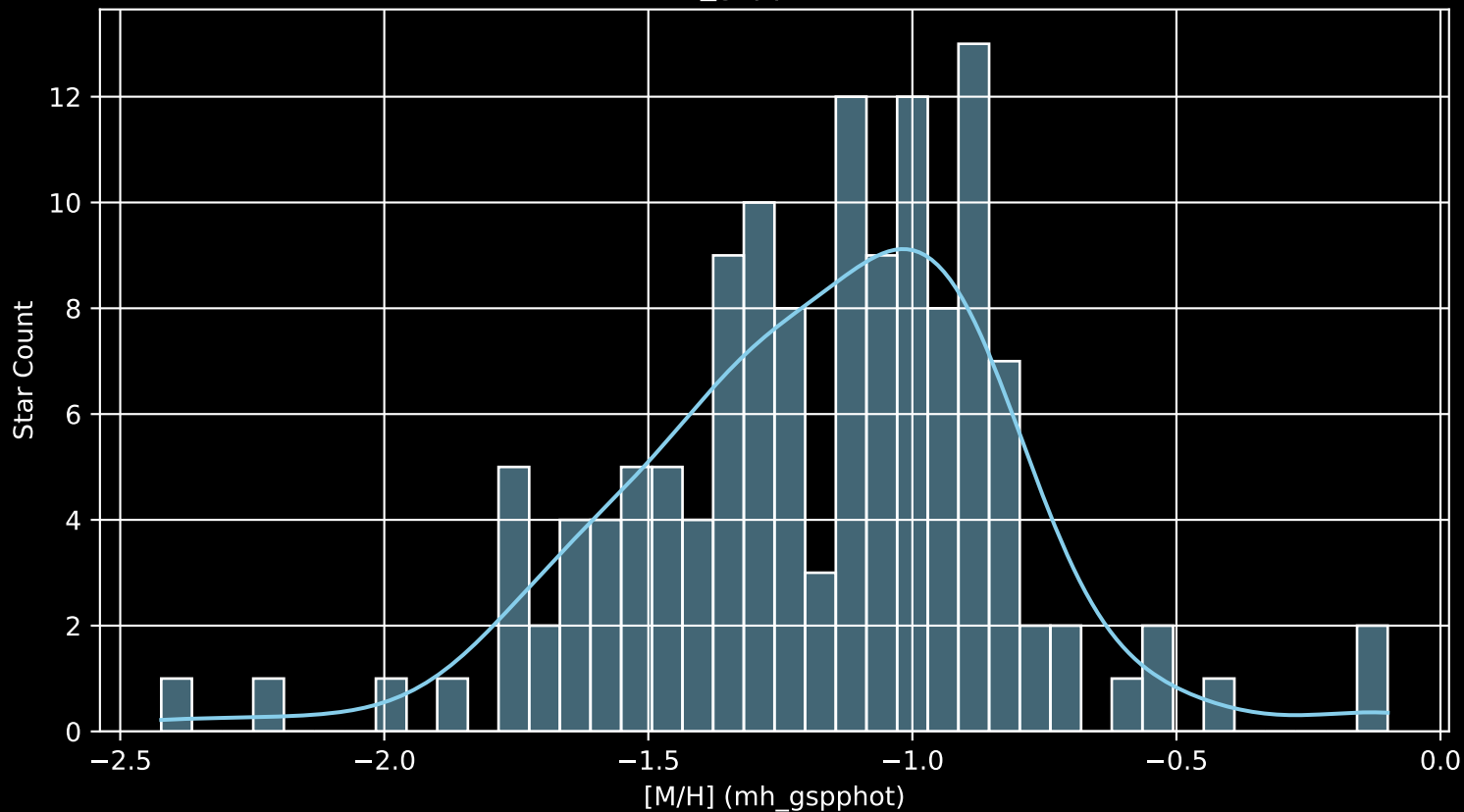
Gaia Stream: [C-9 [M/H] (mh_gspphot) (n= 134)
