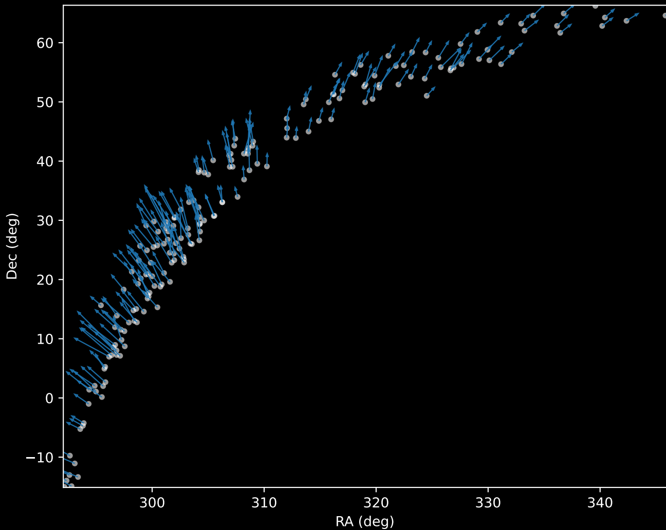
Gaia DR3 Cluster 0 Proper Motion Vectors (n=184)
