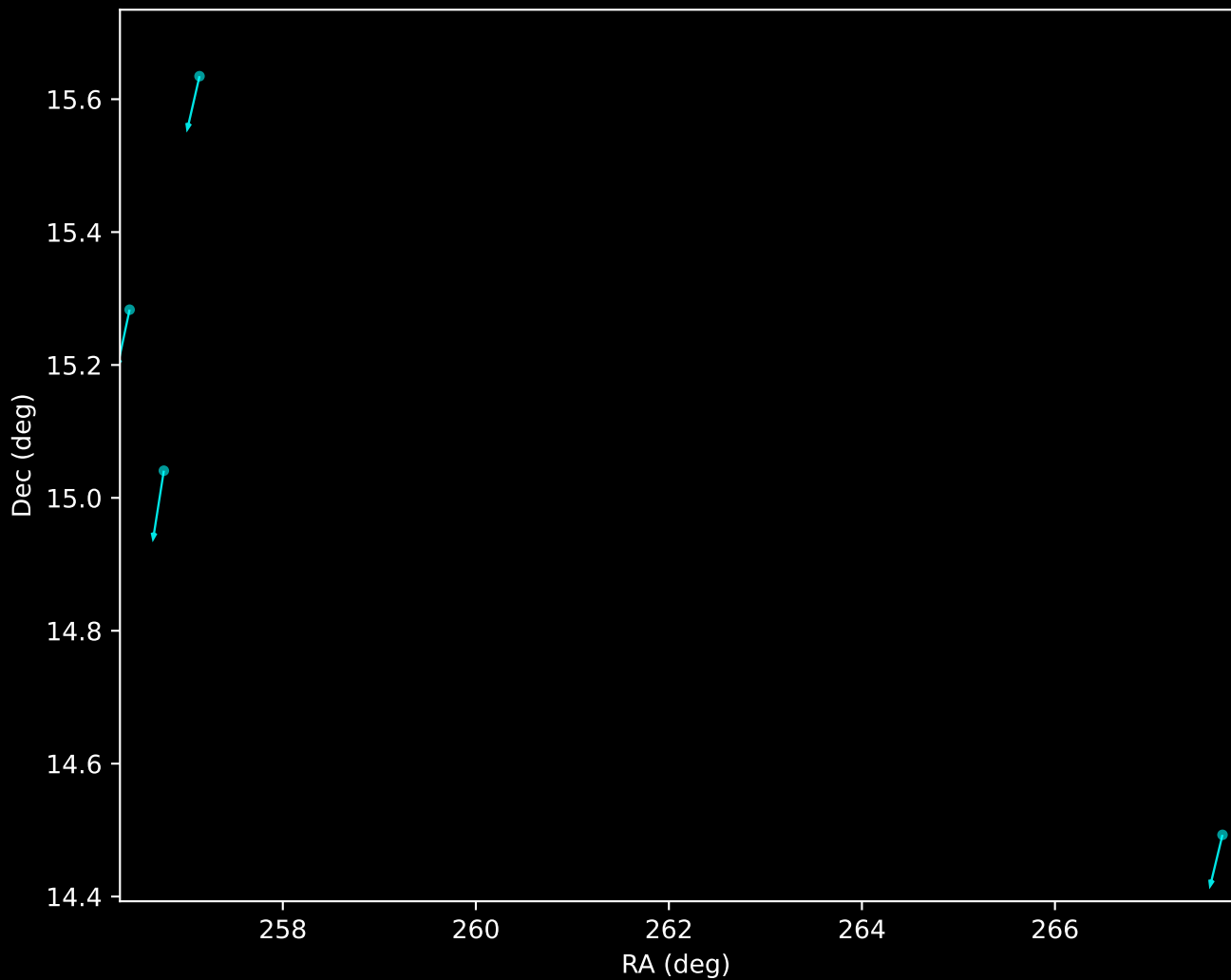
Gaia DR3 Noise Stream Proper Motion Vectors (n=4)
