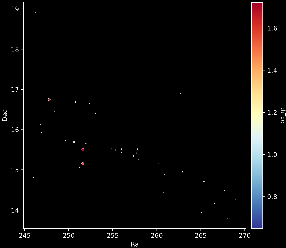
Gaia Stream: [Gaia-10] Stars: 83
