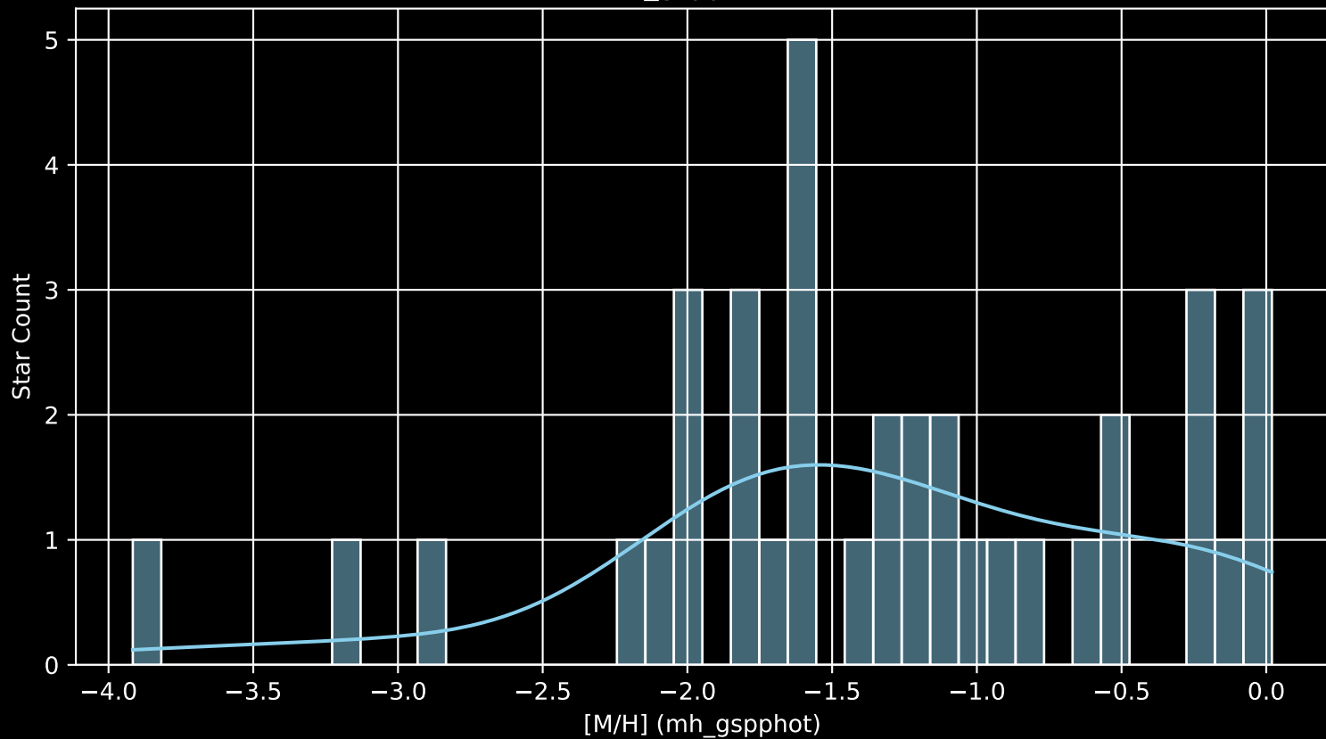
Gaia Stream: [Gaia-10 [M/H] (mh_gspphot) (n= 37)
