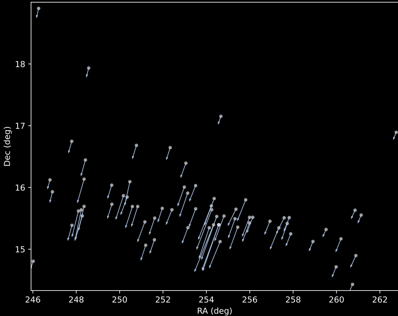
Gaia DR3 Cluster 1 Proper Motion Vectors (n=67)
