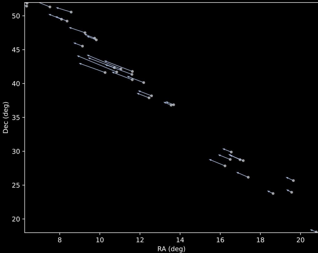
Gaia DR3 Cluster 1 Proper Motion Vectors (n=32)
