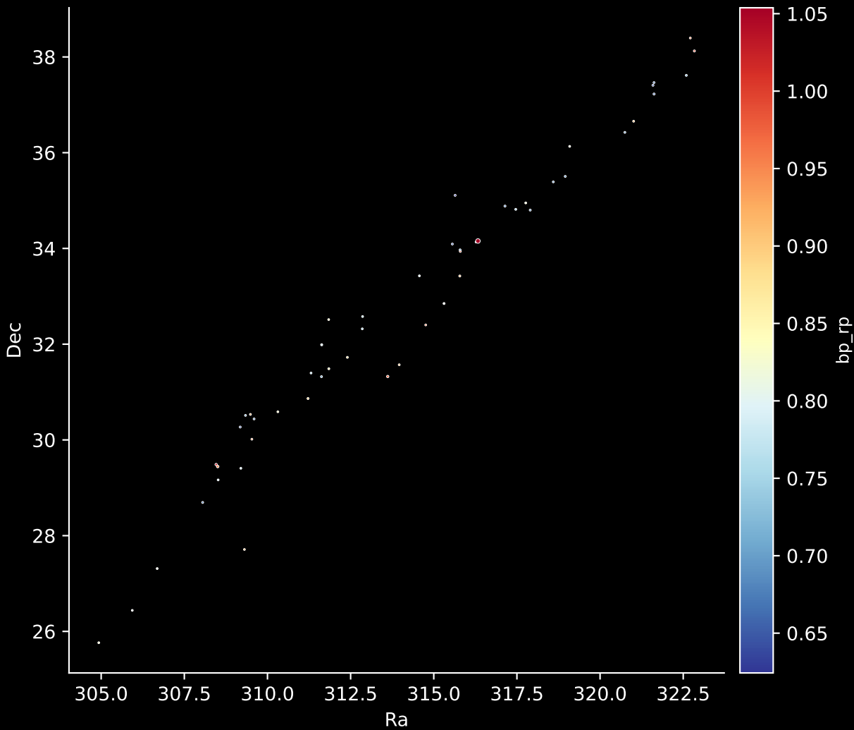
Gaia Stream: [Gaia-6] Stars: 88
