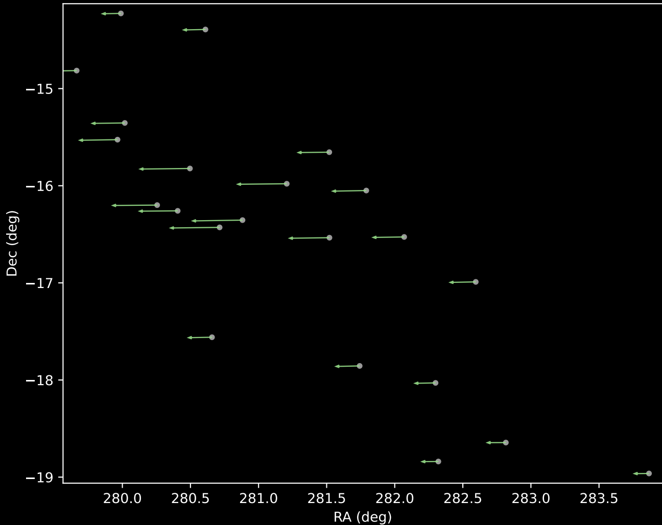
Gaia DR3 Cluster 5 Proper Motion Vectors (n=22)
