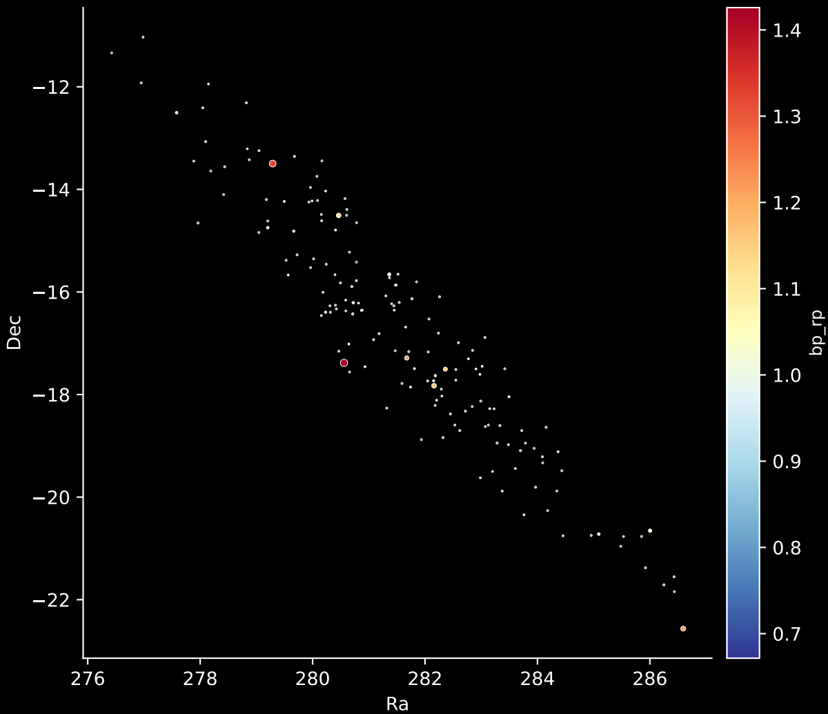
Gaia Stream: [Gaia-7] Stars: 216
