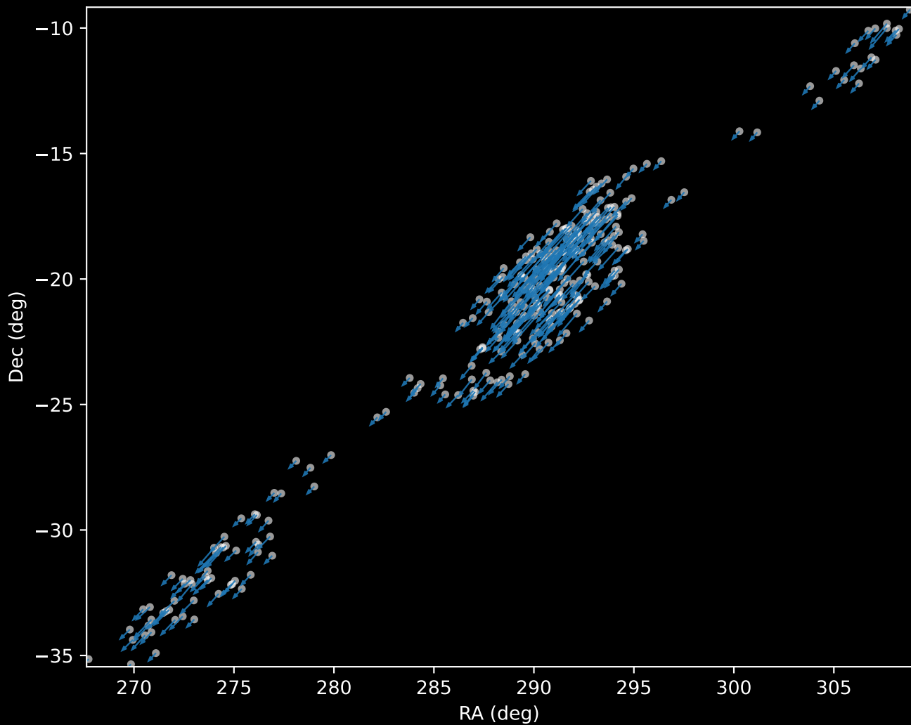
Gaia DR3 Cluster 0 Proper Motion Vectors (n=288)
