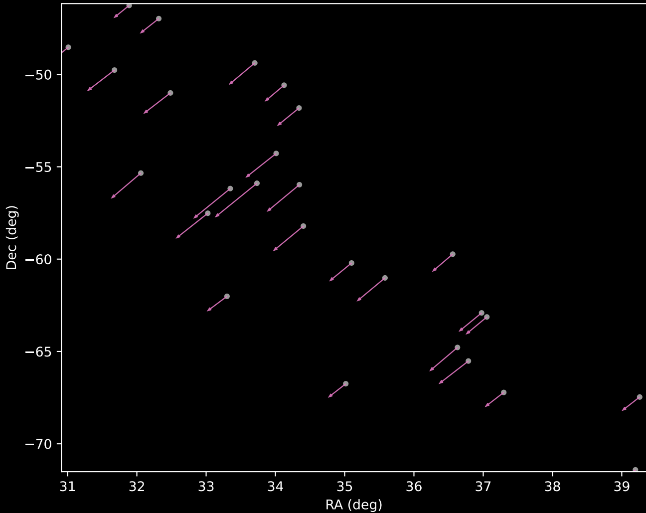
Gaia DR3 Cluster 32 Proper Motion Vectors (n=27)
