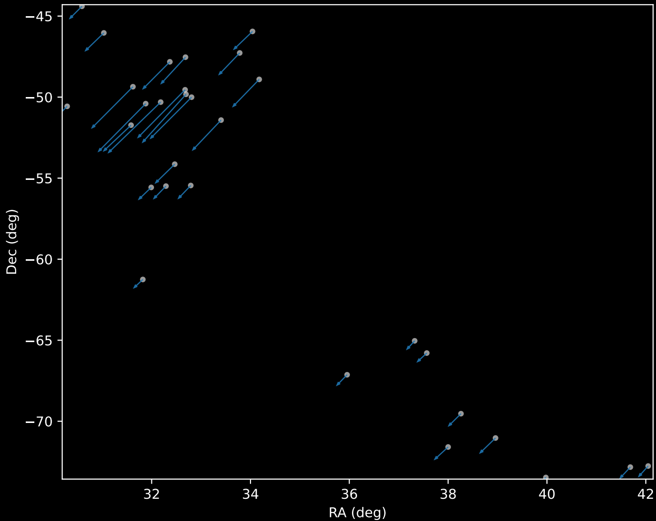
Gaia DR3 Cluster 40 Proper Motion Vectors (n=30)
