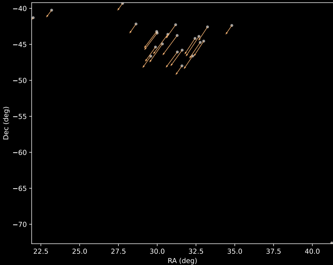
Gaia DR3 Cluster 23 Proper Motion Vectors (n=23)
