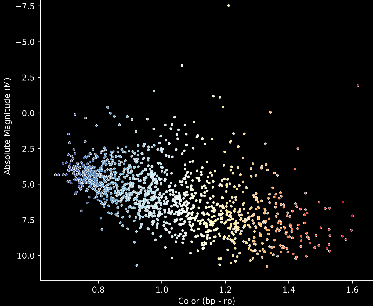
Gaia Stream: [Gaia-9] Stream (n= 1384) Hertzprung-Russel Diagram
