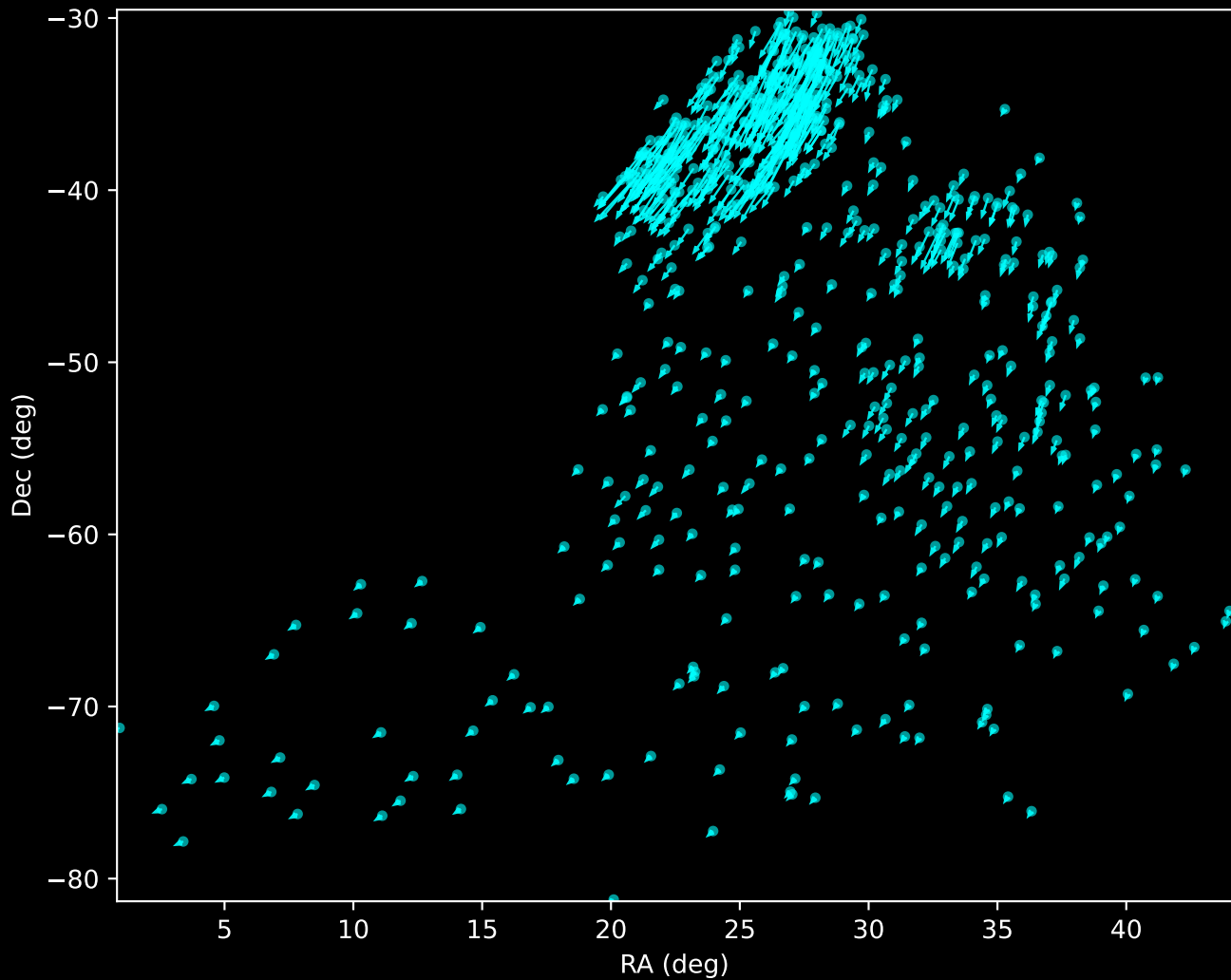
Gaia DR3 Noise Stream Proper Motion Vectors (n=626)
