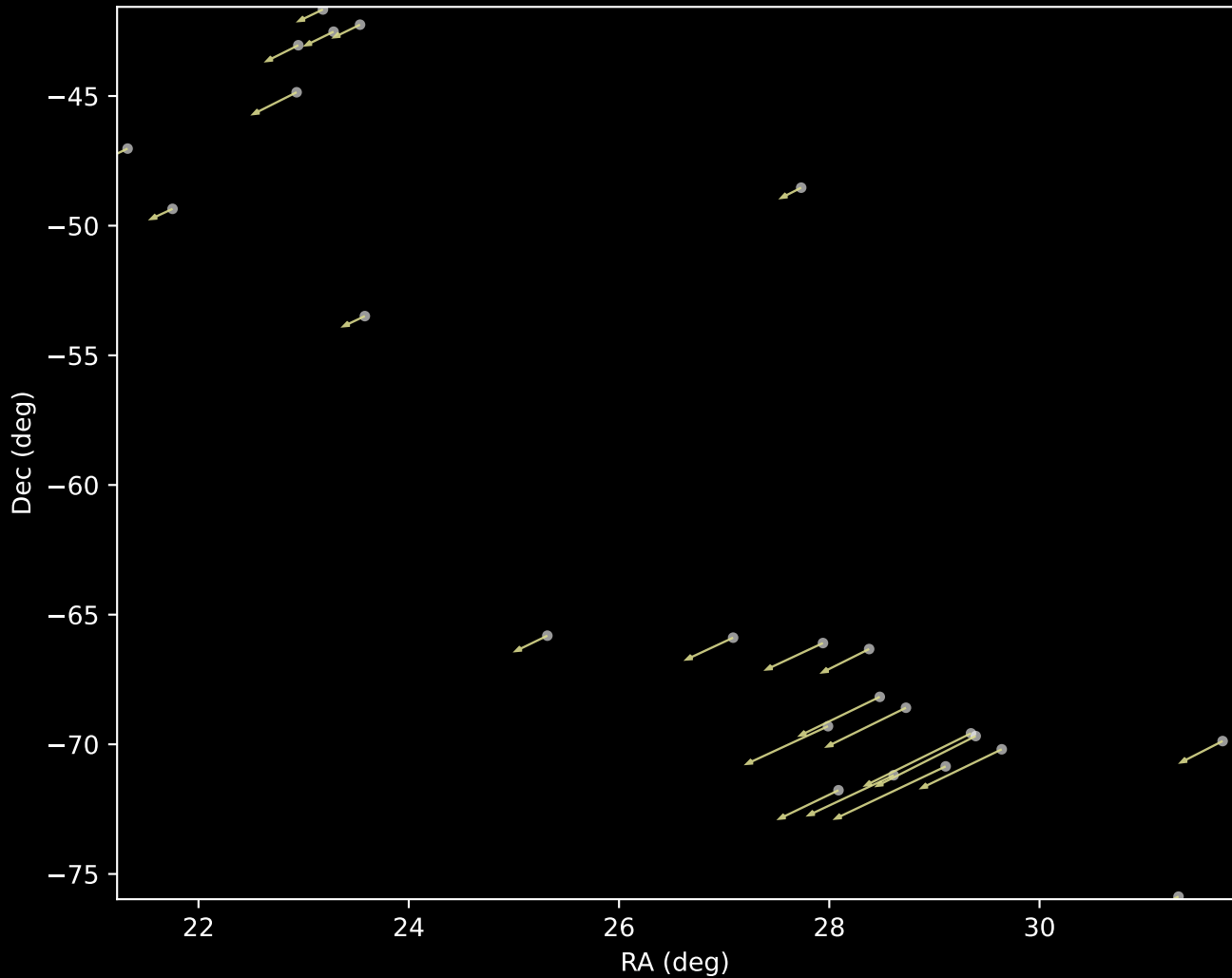
Gaia DR3 Cluster 37 Proper Motion Vectors (n=24)
