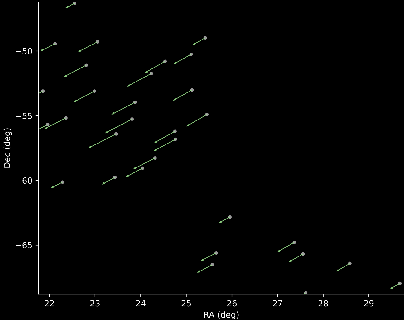
Gaia DR3 Cluster 25 Proper Motion Vectors (n=31)
