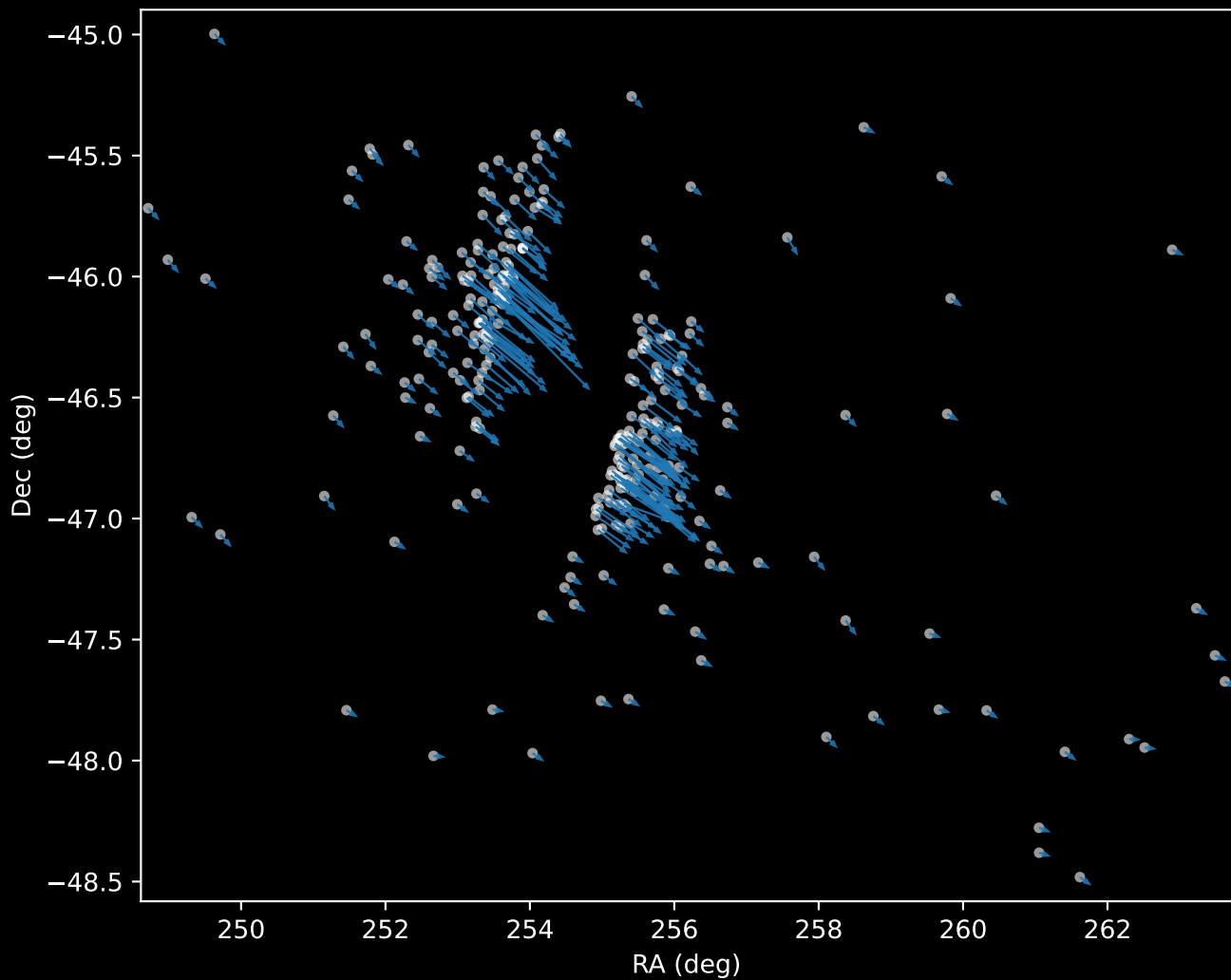
Gaia DR3 Cluster 0 Proper Motion Vectors (n=277)
