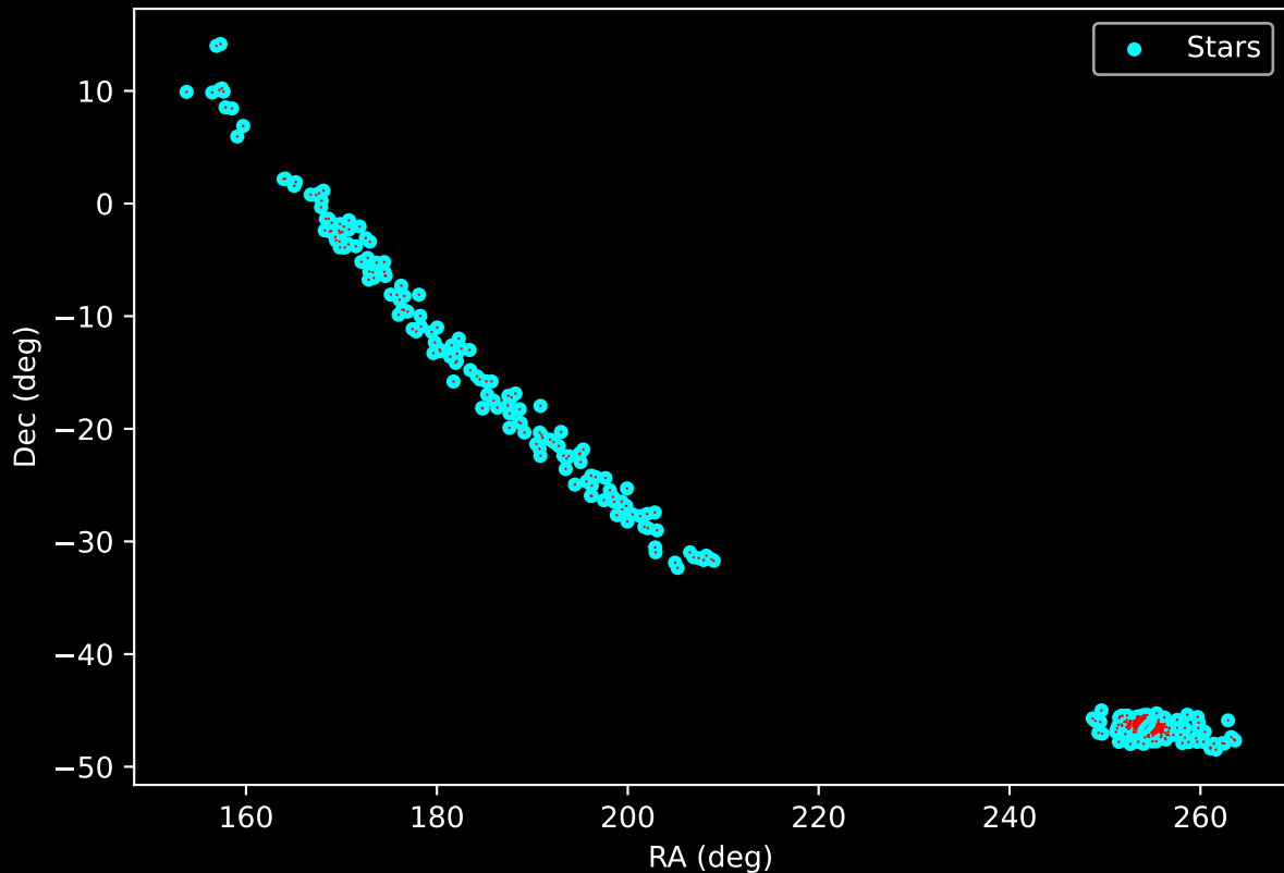
Gaia Stream: [Gjoll] Proper Motion Vectors for Gaia Star Field (n= 437)
