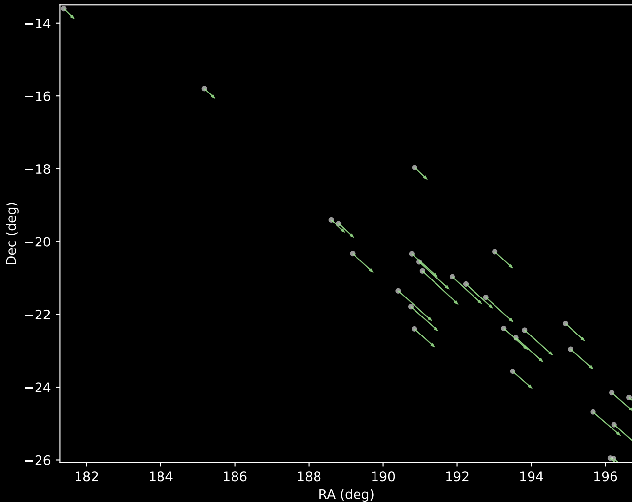
Gaia DR3 Cluster 5 Proper Motion Vectors (n=28)
