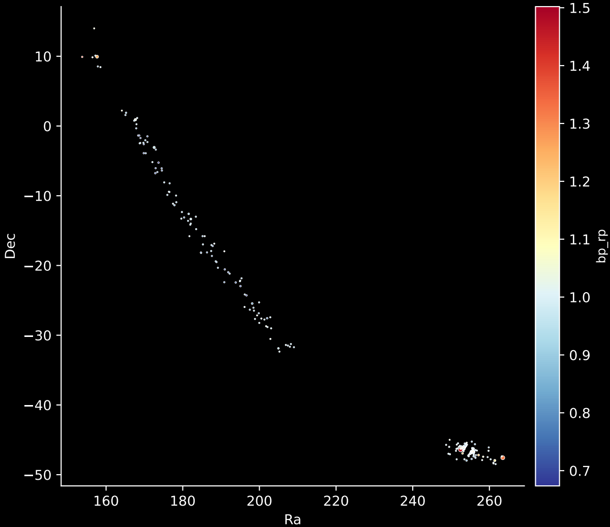
Gaia Stream: [Gjoll] Stars: 437
