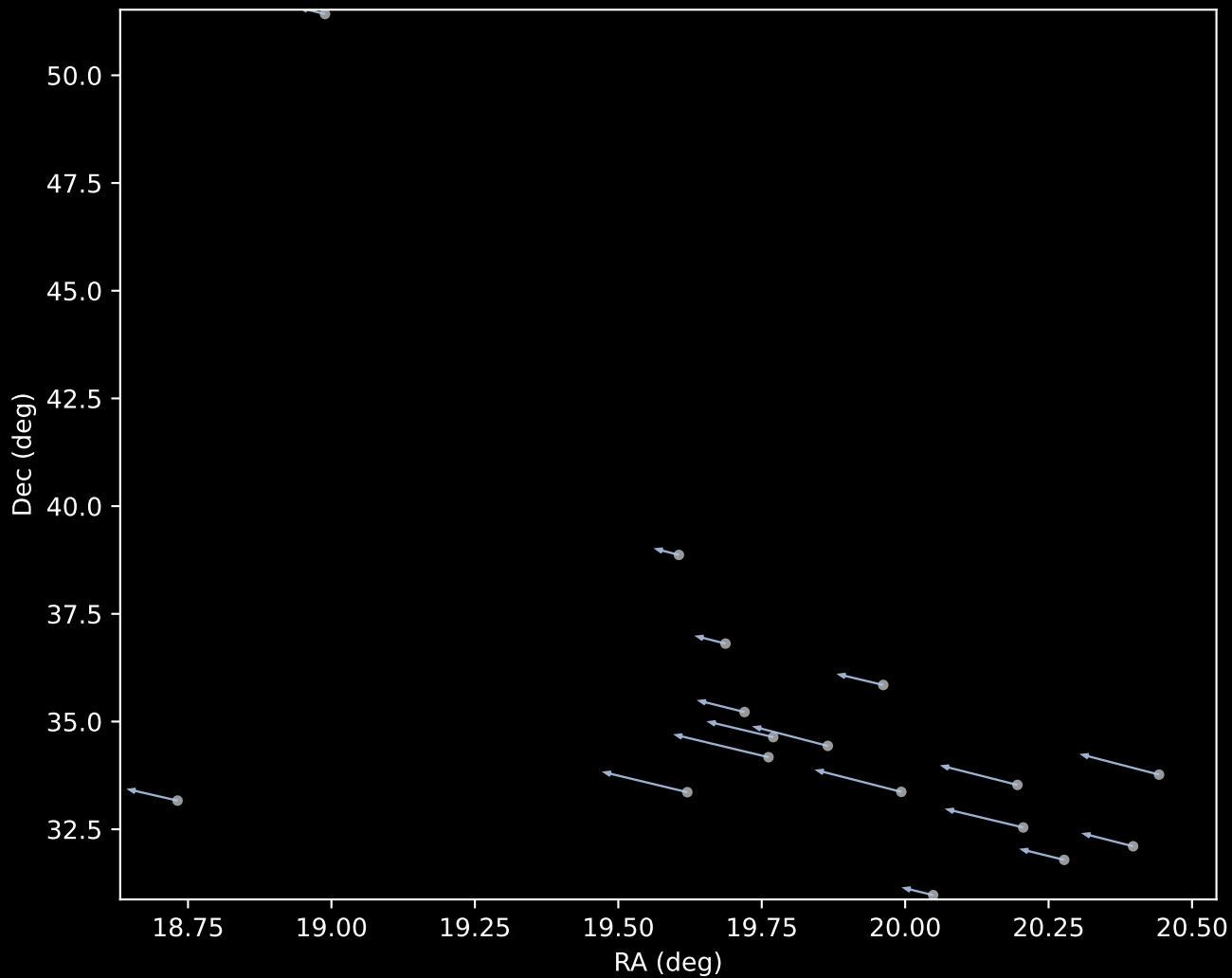
Gaia DR3 Cluster 21 Proper Motion Vectors (n=17)
