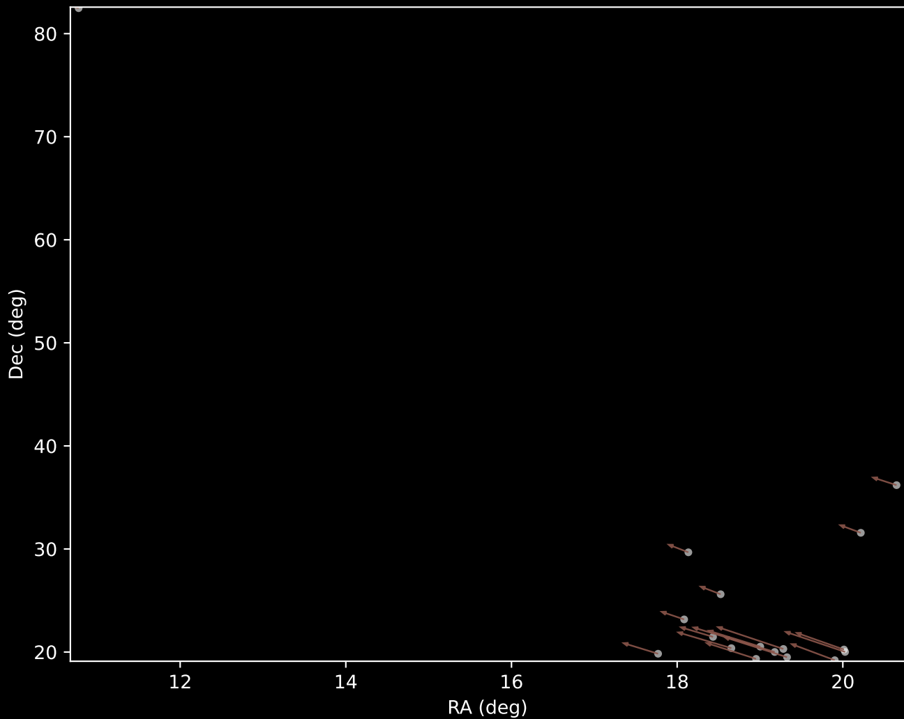
Gaia DR3 Cluster 10 Proper Motion Vectors (n=17)
