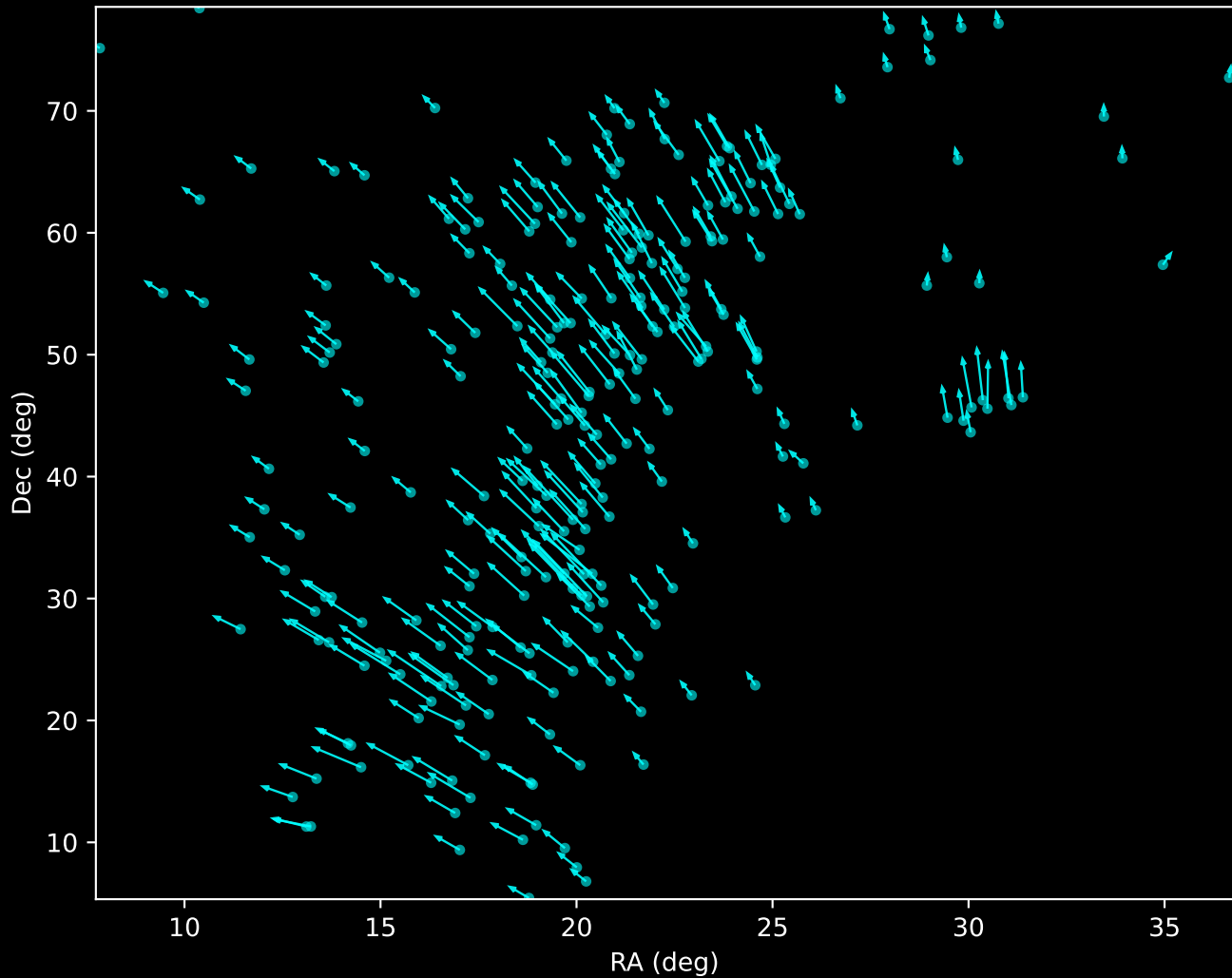
Gaia DR3 Noise Stream Proper Motion Vectors (n=270)
