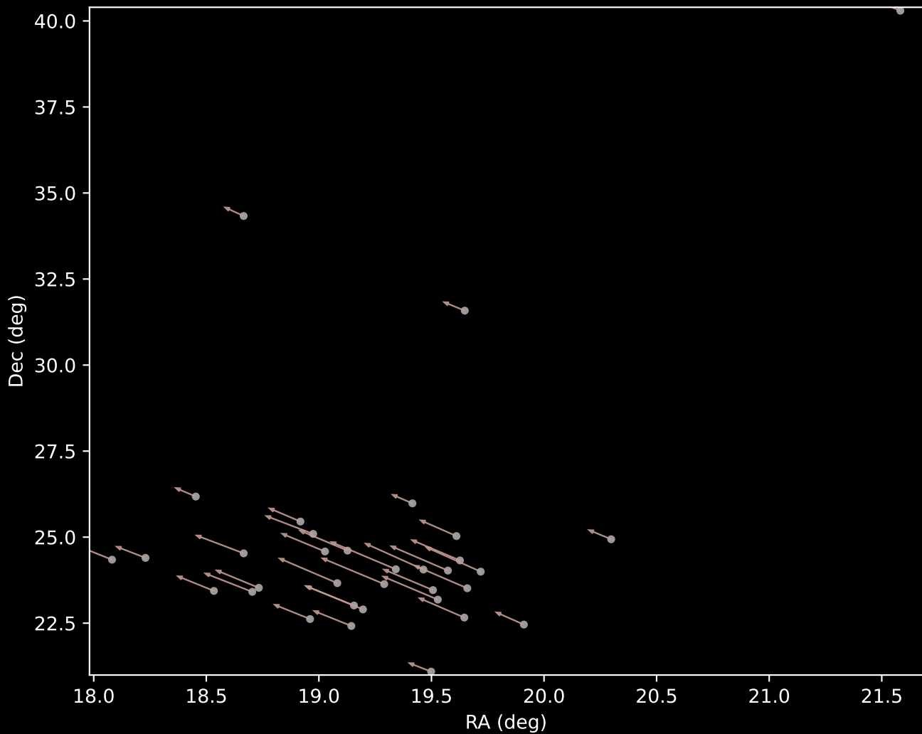
Gaia DR3 Cluster 11 Proper Motion Vectors (n=34)
