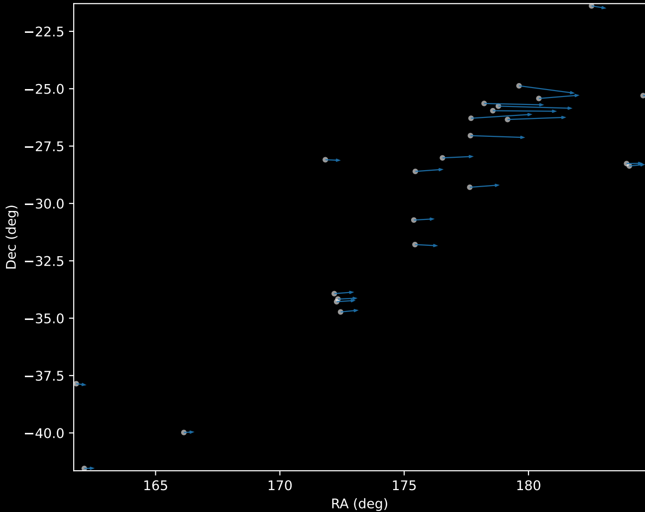
Gaia DR3 Cluster 0 Proper Motion Vectors (n=25)
