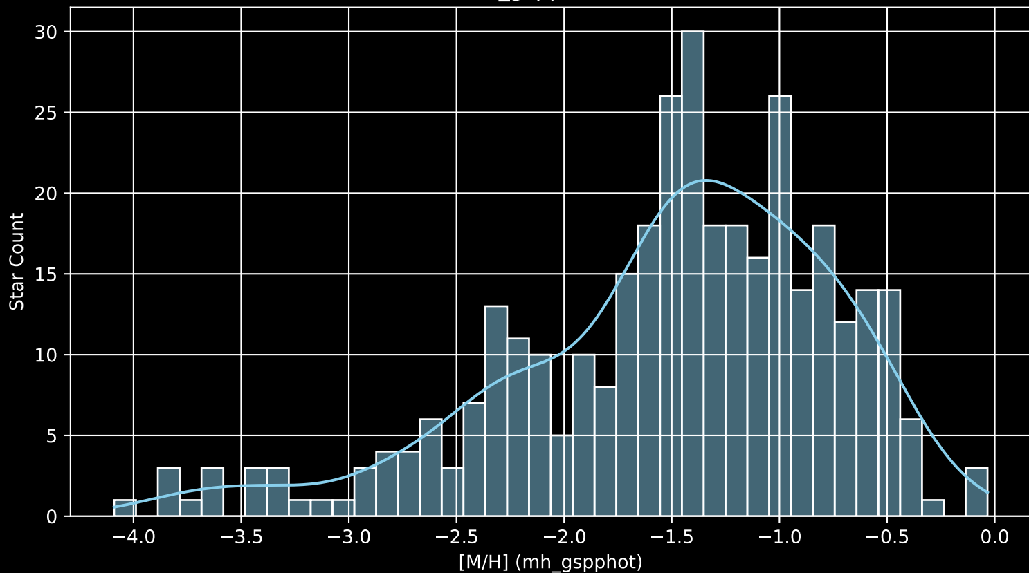
Gaia Stream: [Jhelum [M/H] (mh_gspphot) (n= 350)
