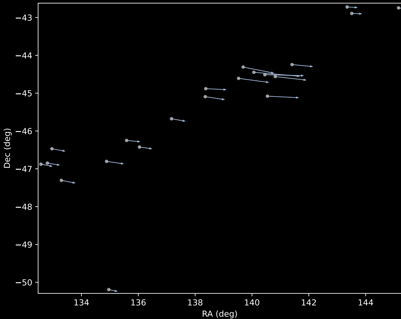
Gaia DR3 Cluster 1 Proper Motion Vectors (n=21)
