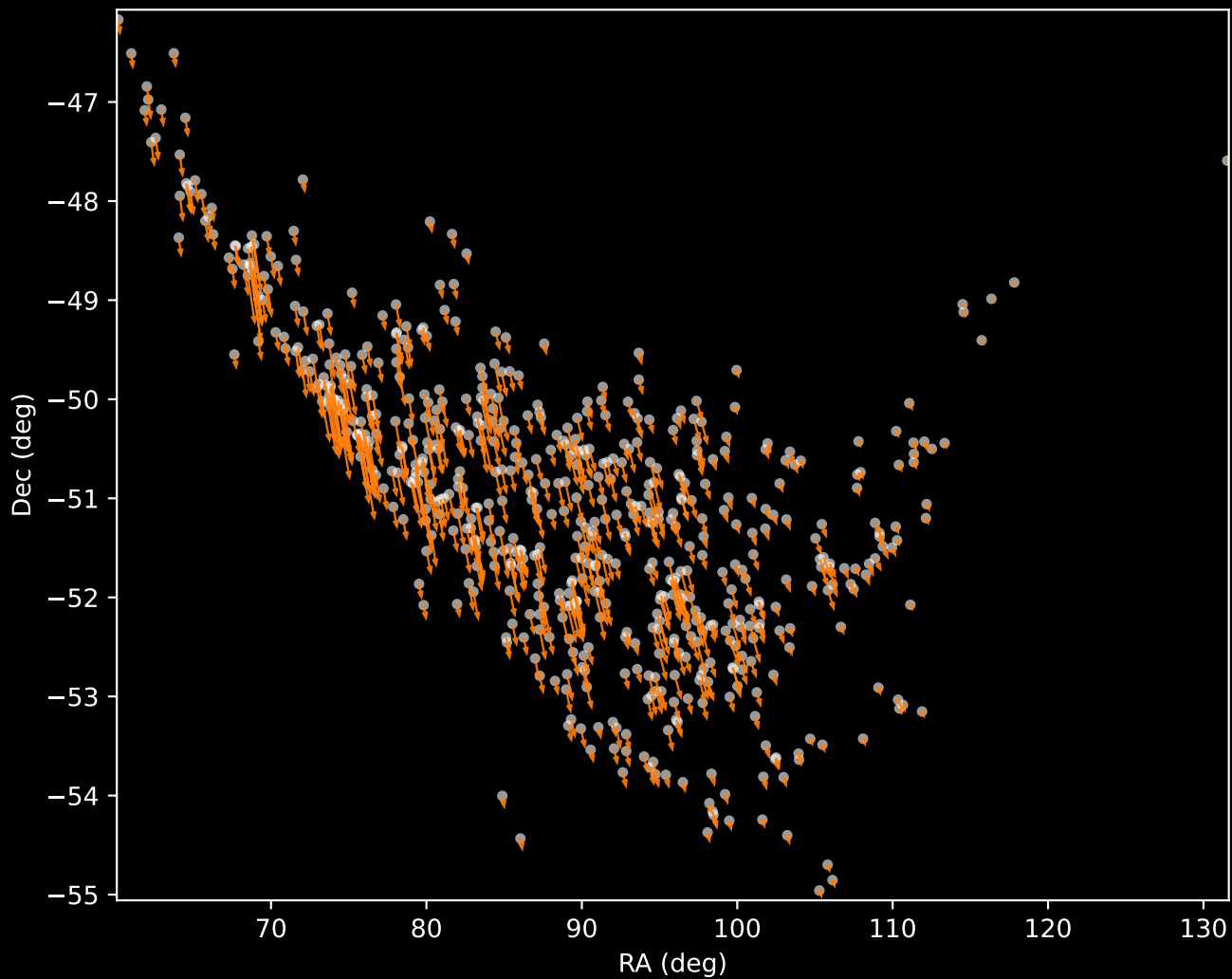
Gaia DR3 Cluster 2 Proper Motion Vectors (n=609)
