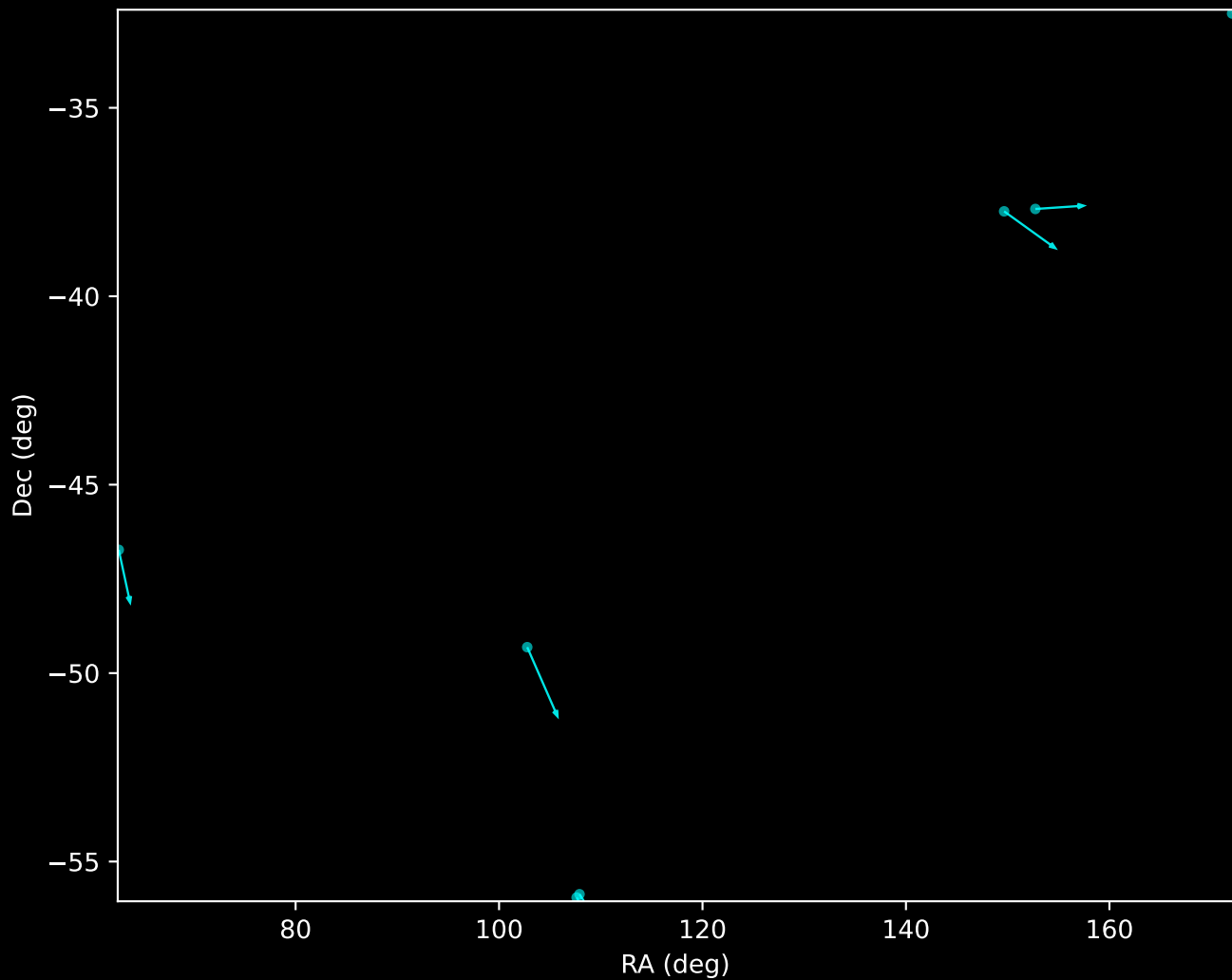
Gaia DR3 Noise Stream Proper Motion Vectors (n=7)
