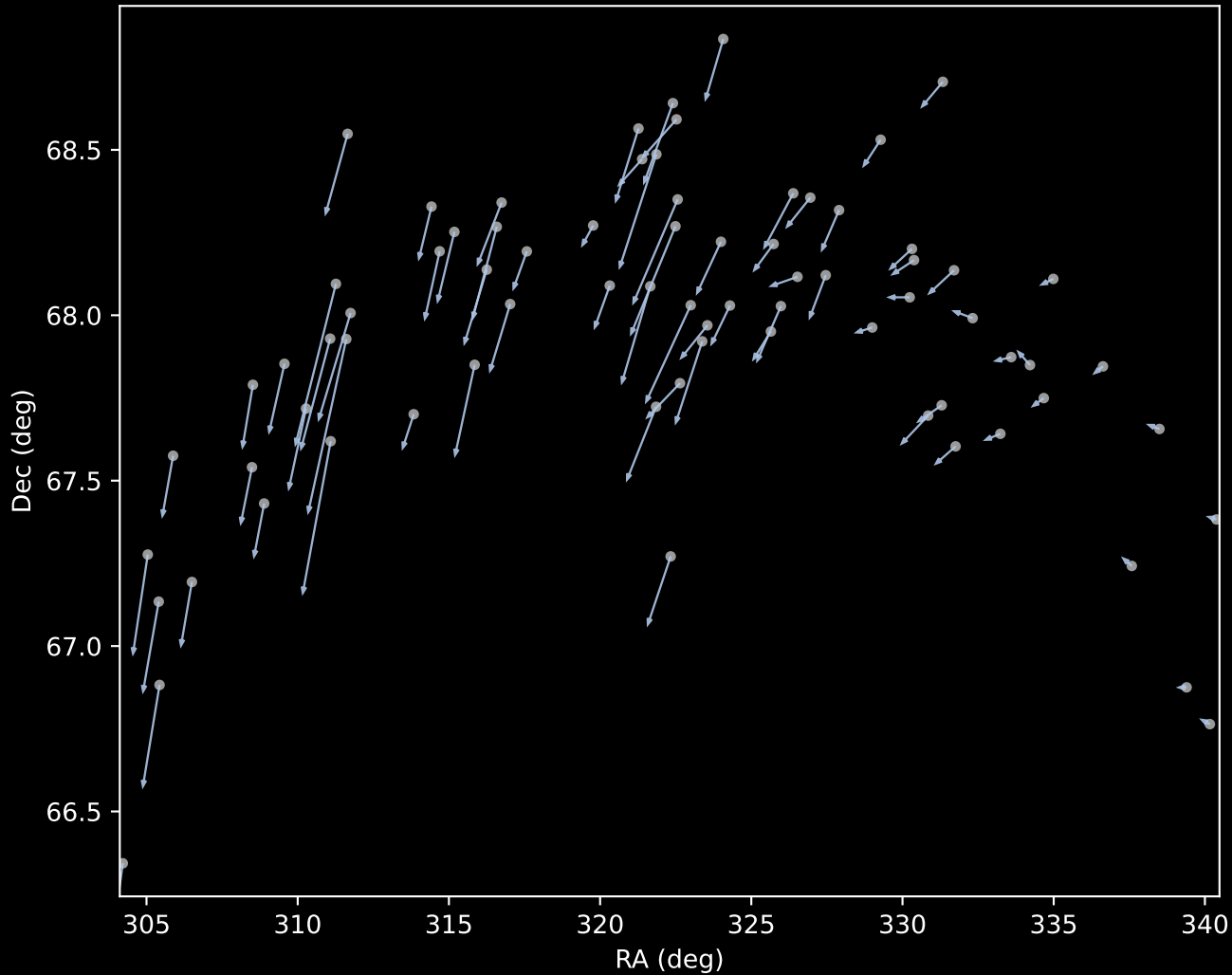
Gaia DR3 Cluster 1 Proper Motion Vectors (n=76)
