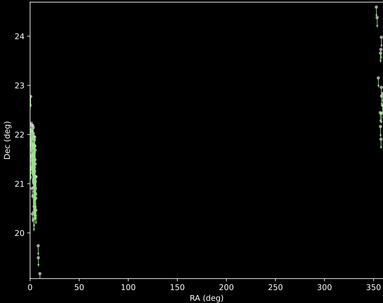
Gaia DR3 Cluster 5 Proper Motion Vectors (n=84)
