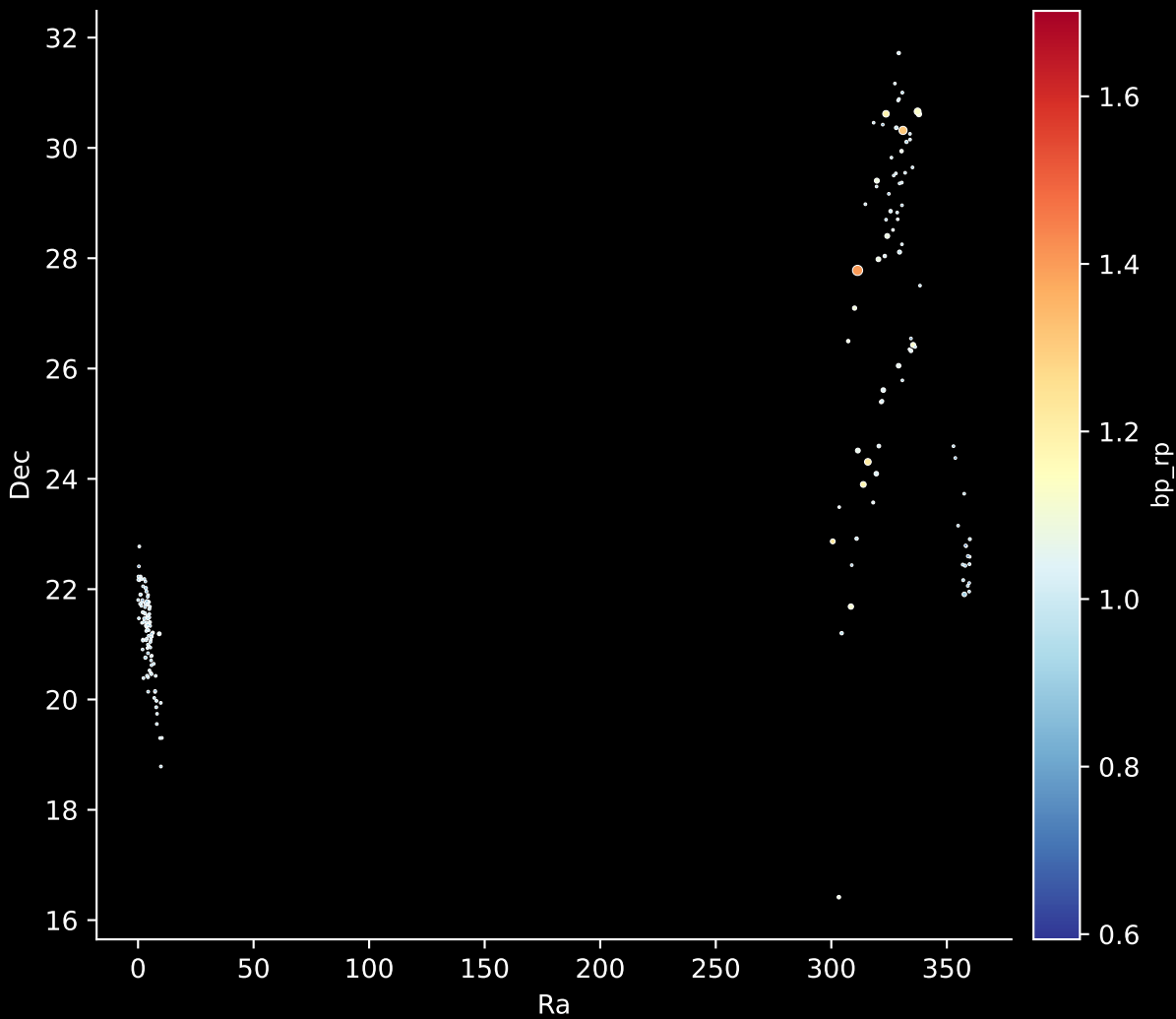
Gaia Stream: [LMS-1] Stars: 255
