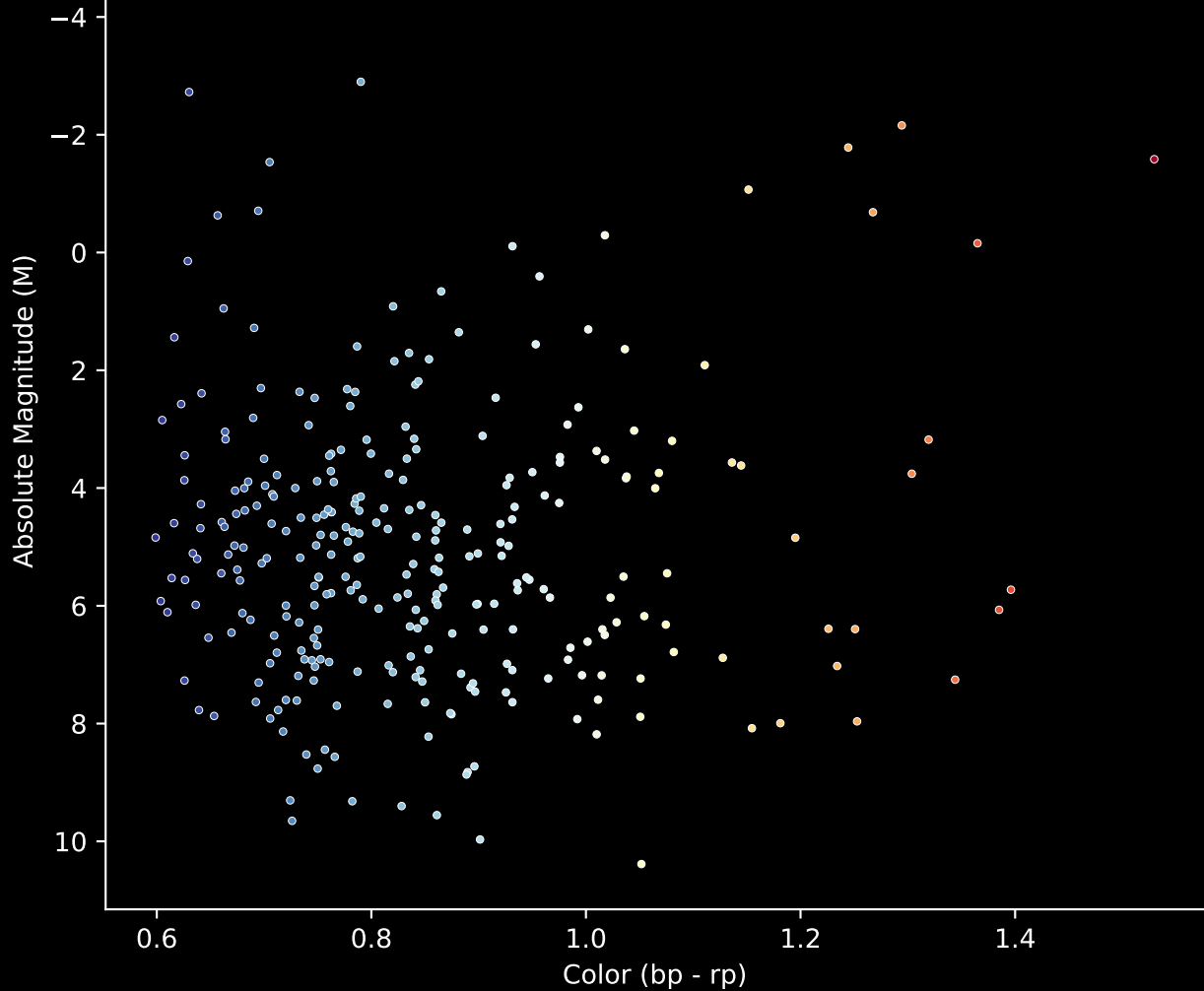
Gaia Stream: [Leiptr] Stream (n= 295) Hertzsprung-Russel Diagram
