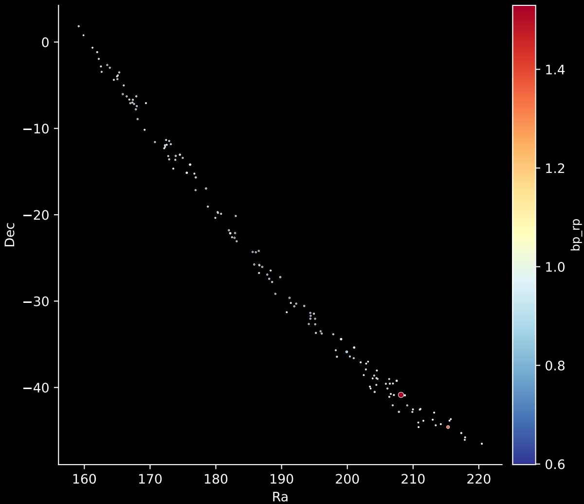
Gaia Stream: [Leiptr] Stars: 295
