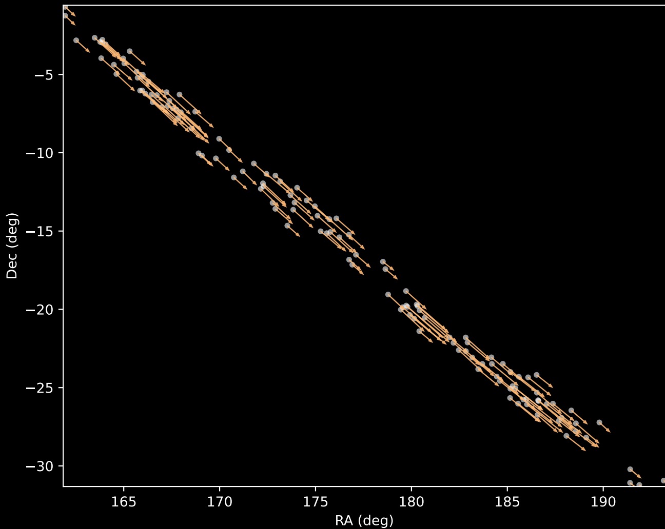
Gaia DR3 Cluster 3 Proper Motion Vectors (n=129)
