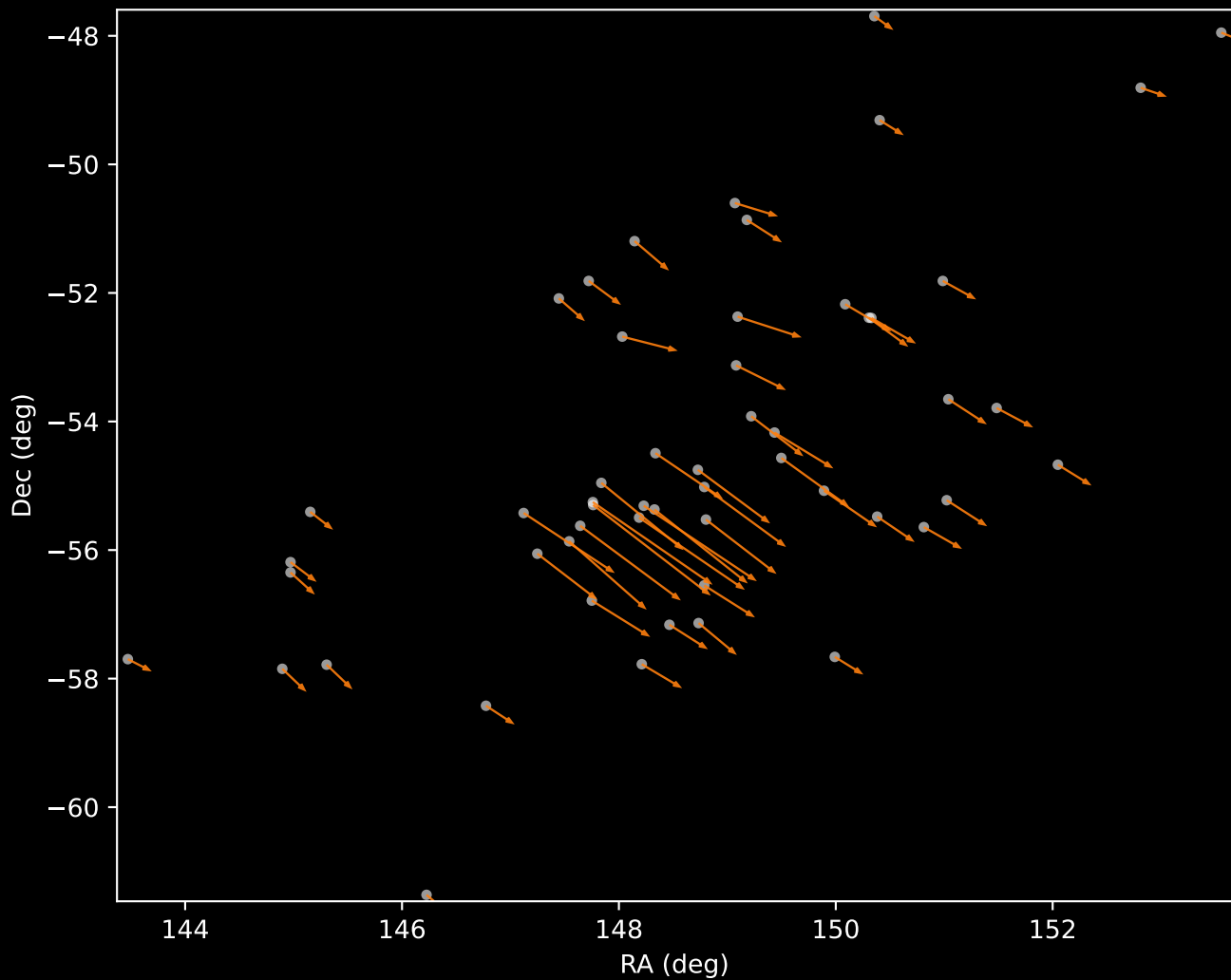
Gaia DR3 Cluster 2 Proper Motion Vectors (n=54)
