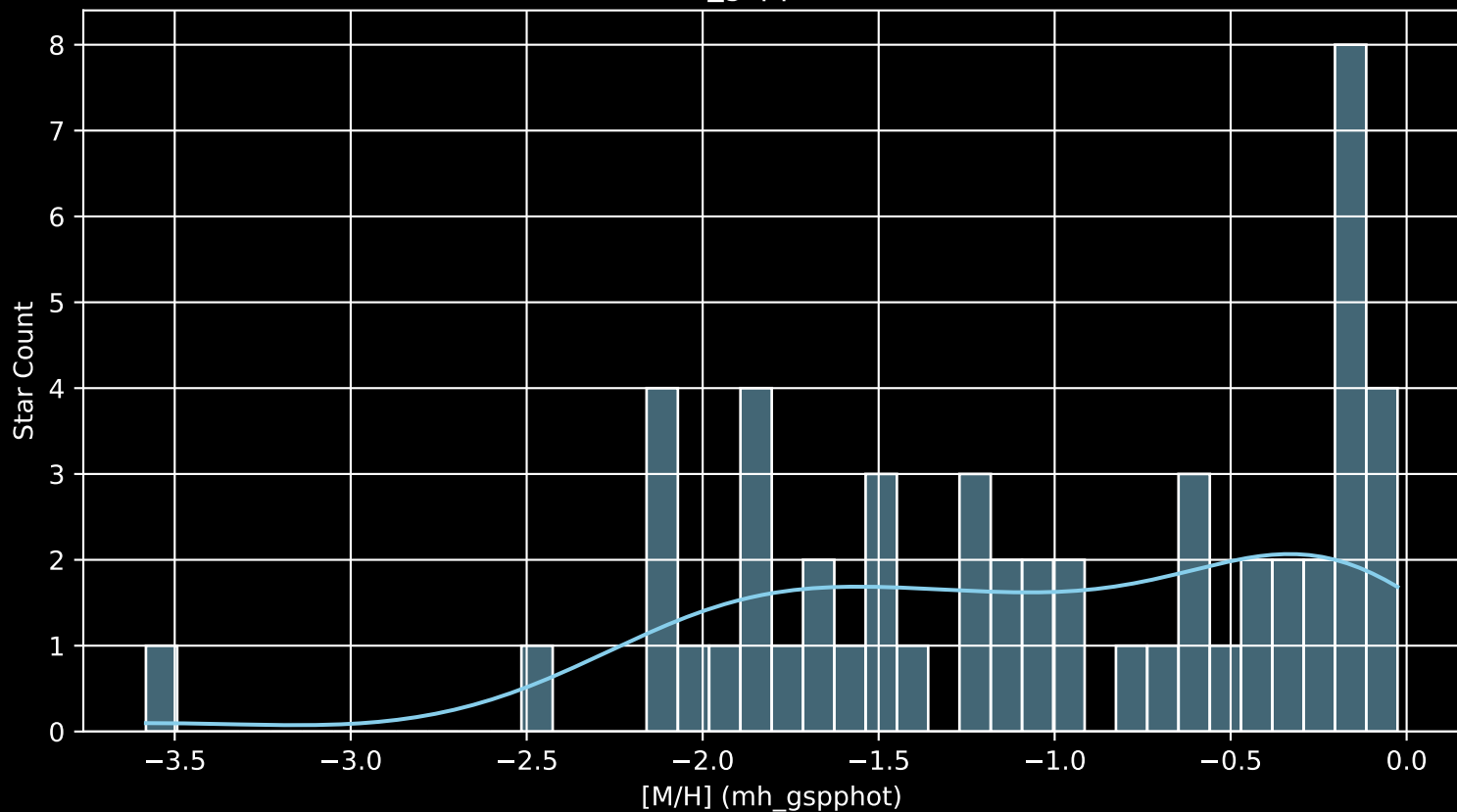
Gaia Stream: [NGC1261a [M/H] (mh_gspphot) (n= 53)
