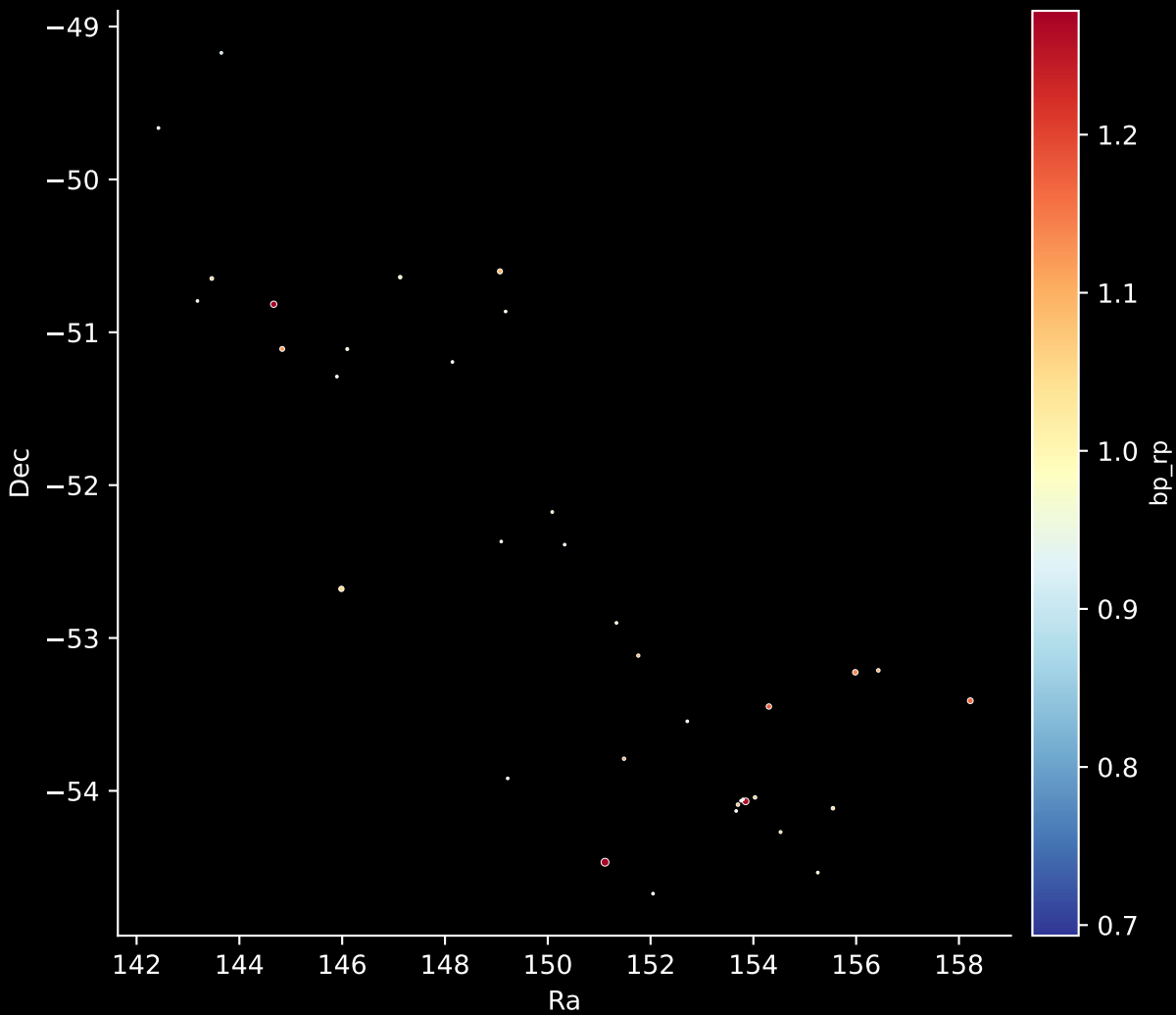
Gaia Stream: [NGC1261b] Stars: 50
