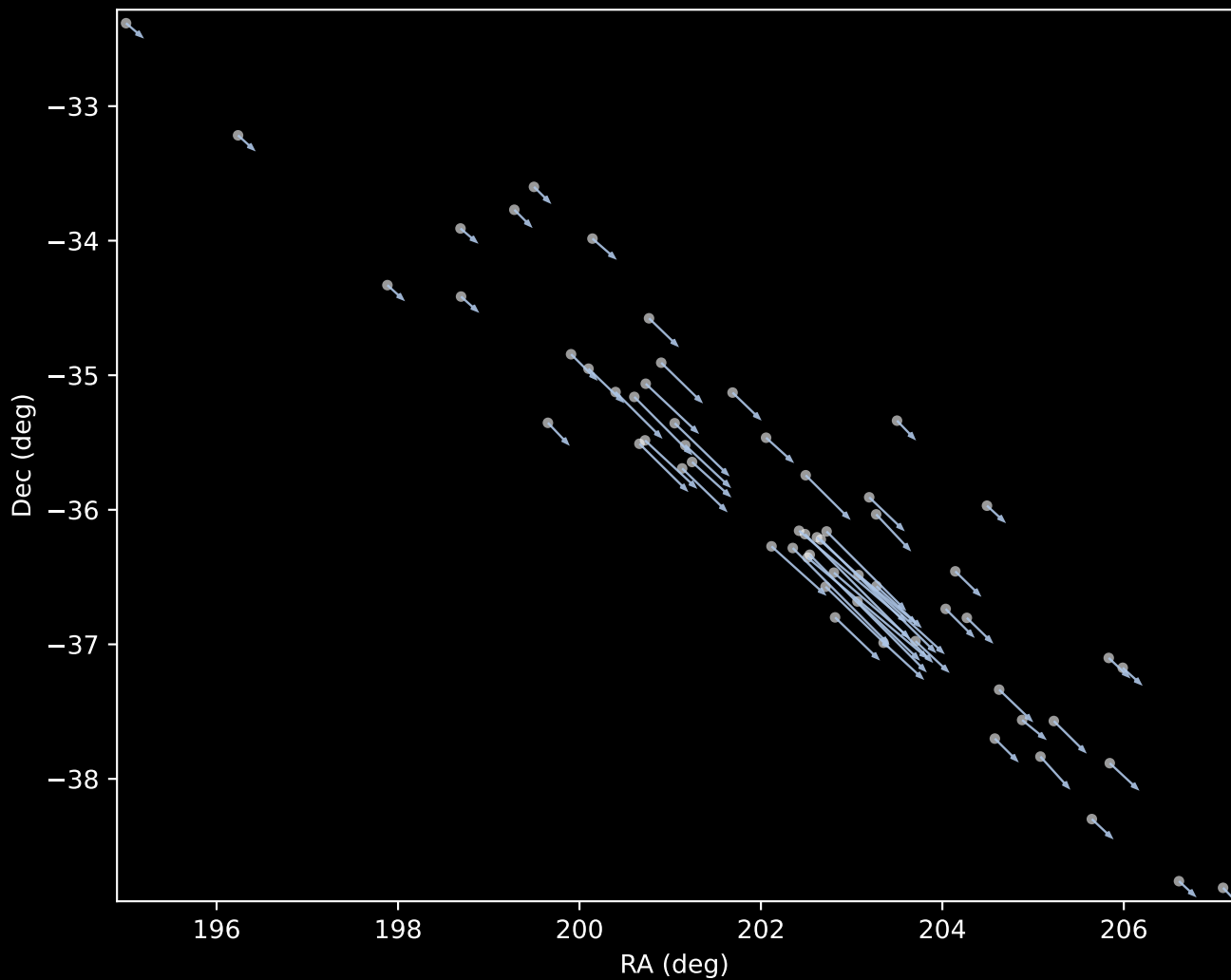
Gaia DR3 Cluster 1 Proper Motion Vectors (n=60)
