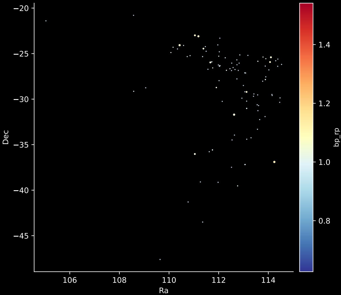
Gaia Stream: [NGC288] Stars: 133
