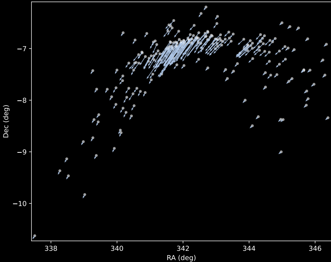
Gaia DR3 Cluster 1 Proper Motion Vectors (n=221)
