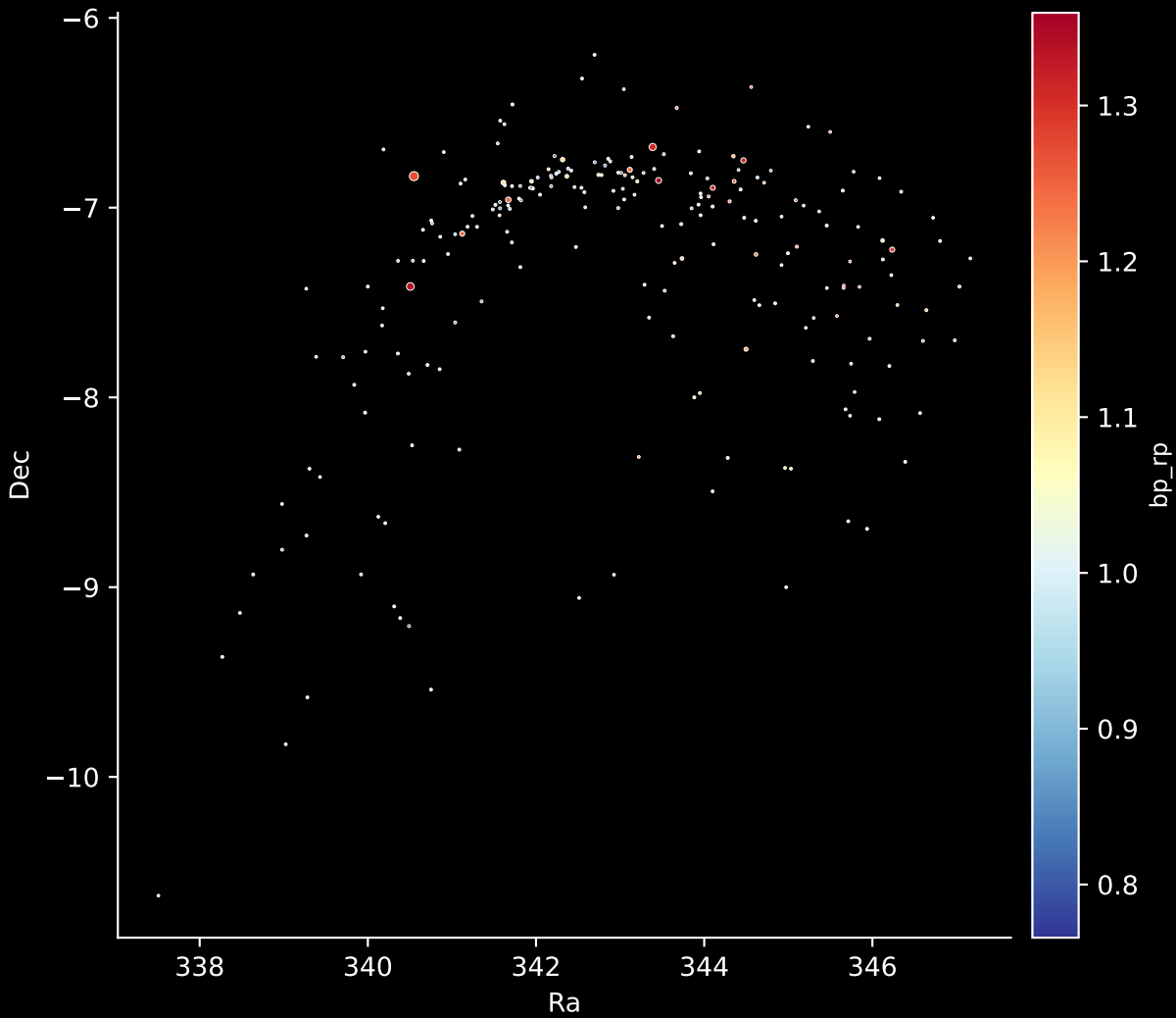
Gaia Stream: [NGC6101] Stars: 277
