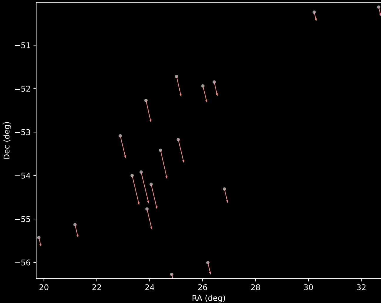
Gaia DR3 Cluster 27 Proper Motion Vectors (n=18)
