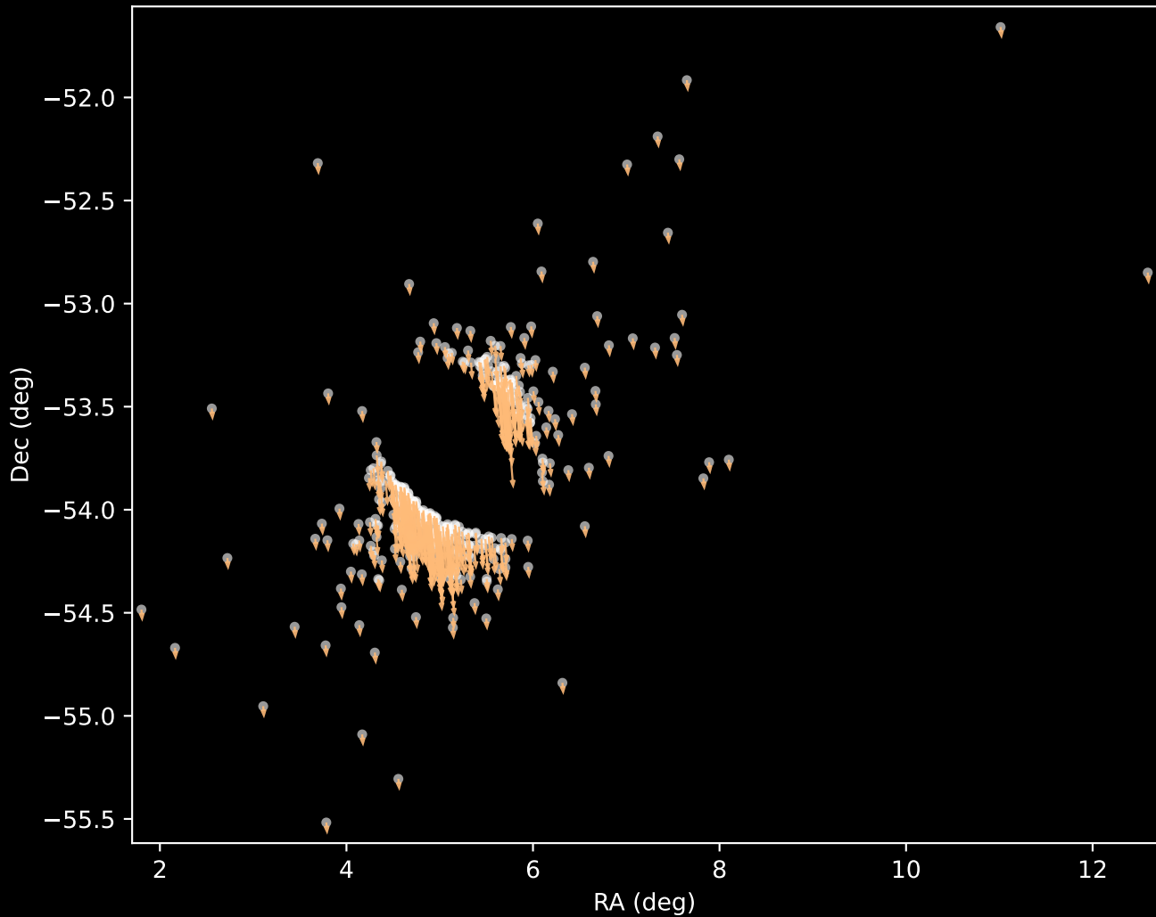
Gaia DR3 Cluster 3 Proper Motion Vectors (n=382)
