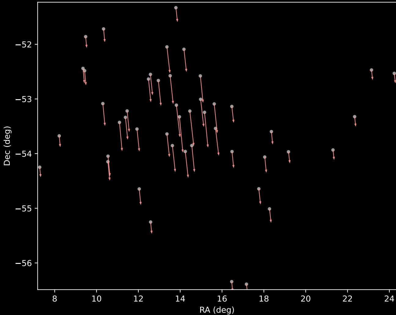
Gaia DR3 Cluster 7 Proper Motion Vectors (n=47)
