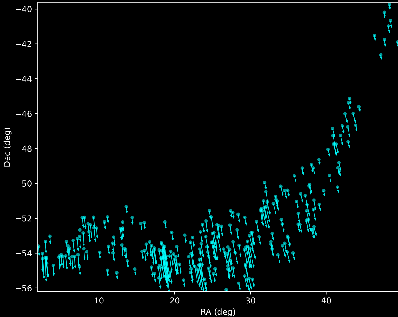
Gaia DR3 Noise Stream Proper Motion Vectors (n=262)
