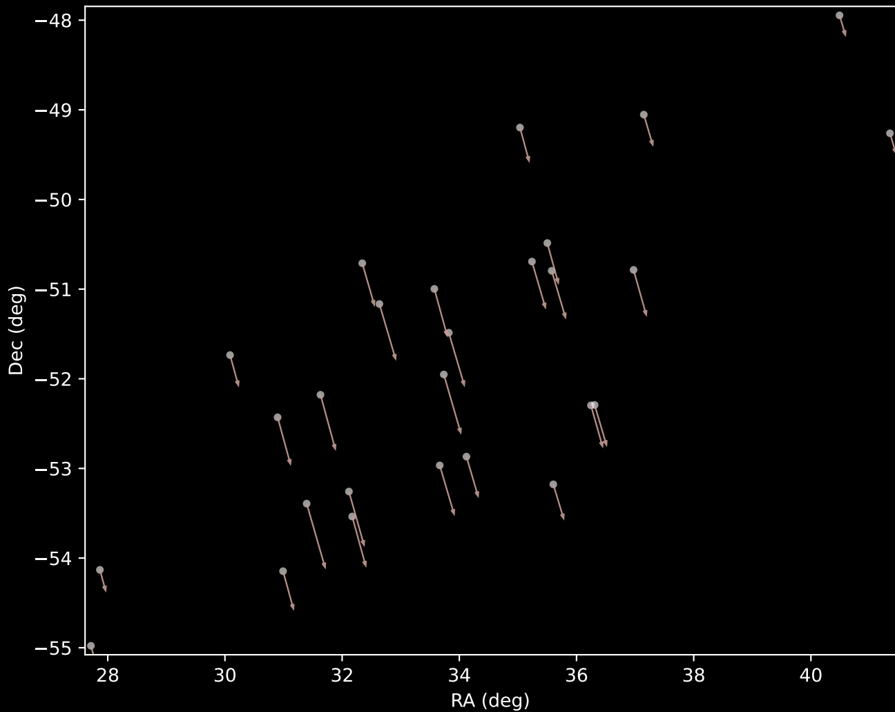
Gaia DR3 Cluster 11 Proper Motion Vectors (n=27)
