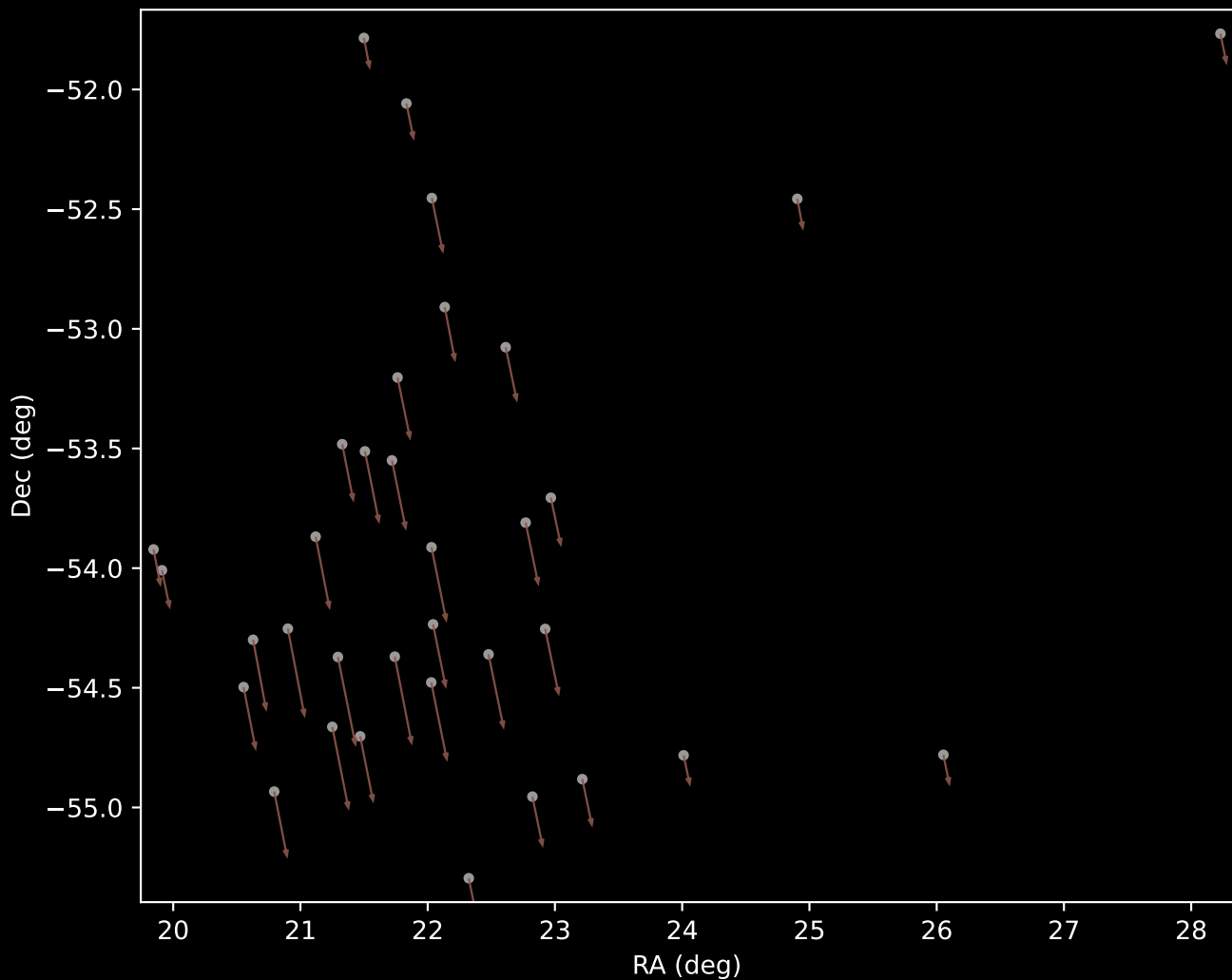
Gaia DR3 Cluster 30 Proper Motion Vectors (n=34)
